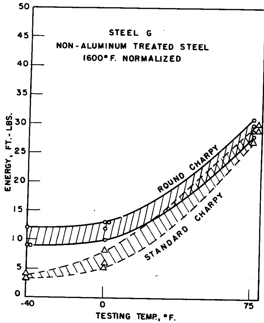
FIGURE 3 . COMPARISON OF NOTCH TOUGHNESS VALUES OF ROUND VERSUS STANDARD CHARPY TEST SPECIMENS ON IDENTICAL STEELS
