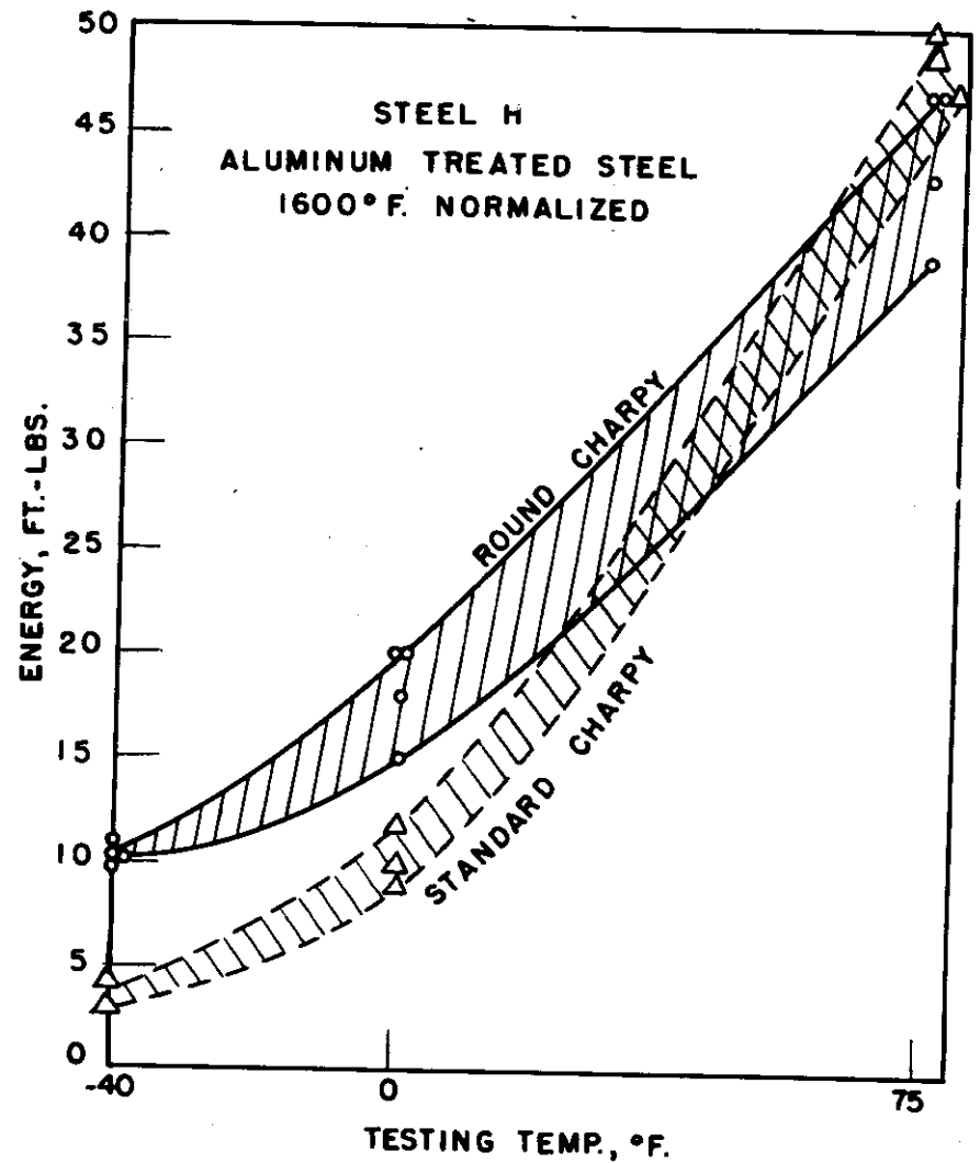
FIGURE 3 . COMPARISON OF NOTCH TOUGHNESS VALUES OF ROUND VERSUS STANDARD CHARPY TEST SPECIMENS ON IDENTICAL STEELS
