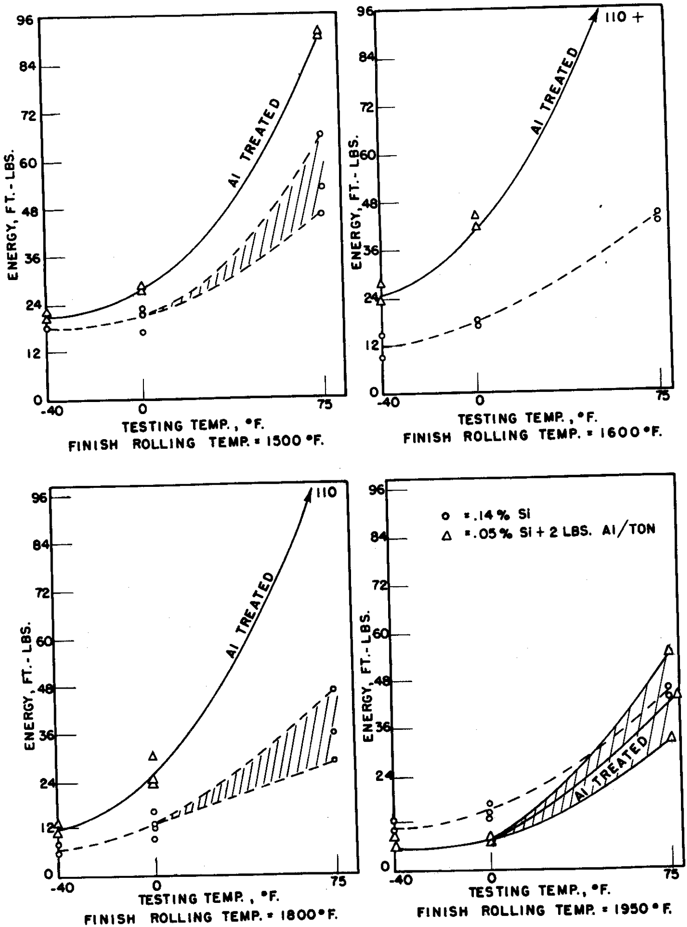
FIGURE 4. NOTCH TOUGHNESS CURVES ON HIGH-SILICON HULL PLATE STEEL HOT-ROLLED AT DIFFERENT TEMPERATURES
