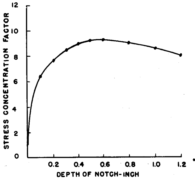
Figure 11. Variation in stress concentration as a function of notch depth for bar of indicated dimensions. (Calculation by L. R. Jackson, Applied Physics Division, Battelle Memorial Institute.)
