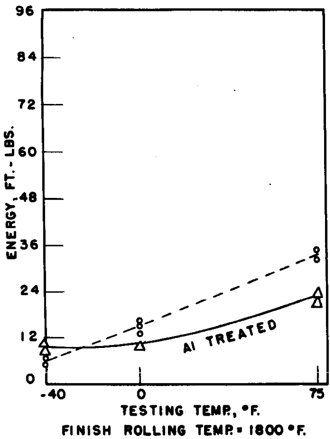
FIGURE 5 . NOTCH TOUGHNESS CURVES LOW-SILICON HULL PLATE STEEL HOT-ROLLED AT DIFFERENT TEMPERATURES
