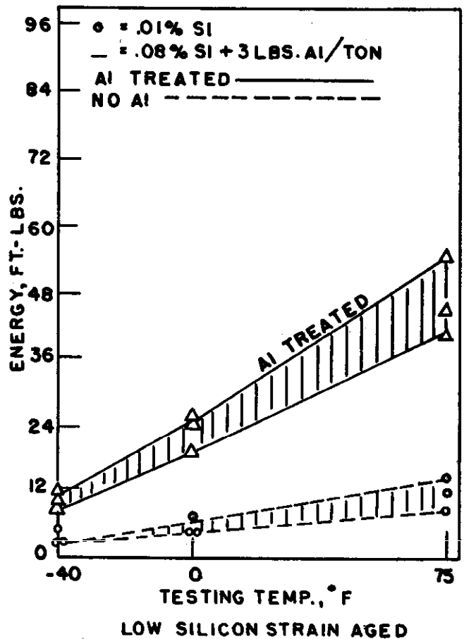
FIGURE 9. EFFECT OF STRAIN AGING UPON THE NOTCH TOUGHNESS OF HULL PLATE STEELS
