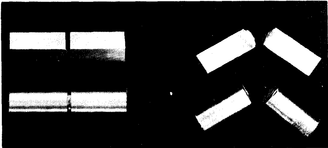
Figure 2. Photograph of V-Notch Charpy and round Charpy specimens before and after breaking.
