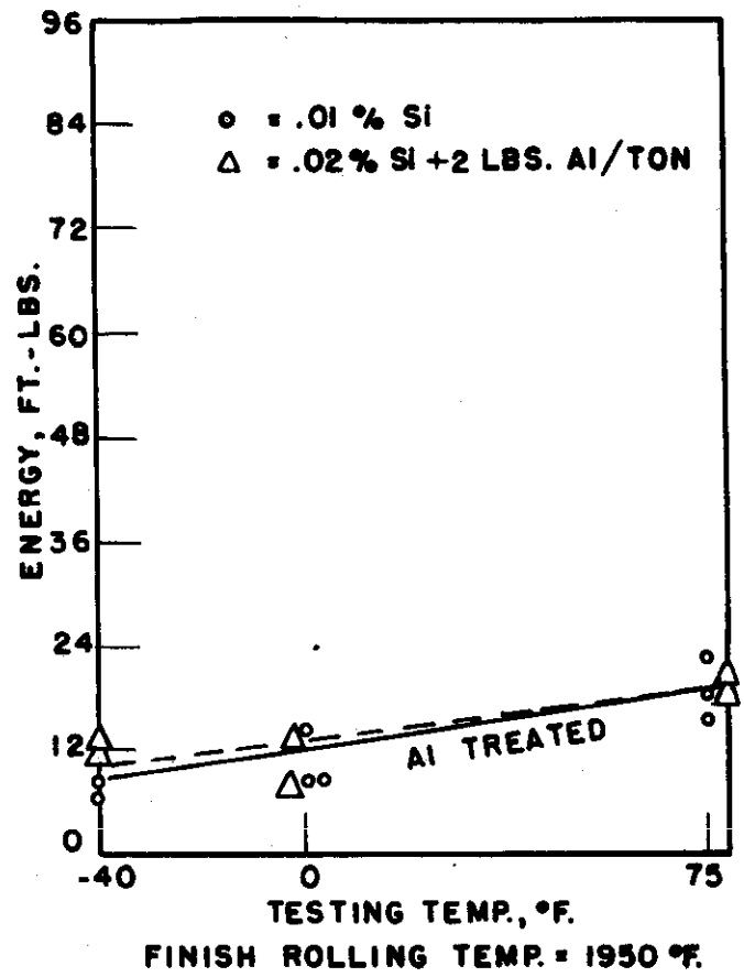
FIGURE 5 . NOTCH TOUGHNESS CURVES LOW-SILICON HULL PLATE STEEL HOT-ROLLED AT DIFFERENT TEMPERATURES
