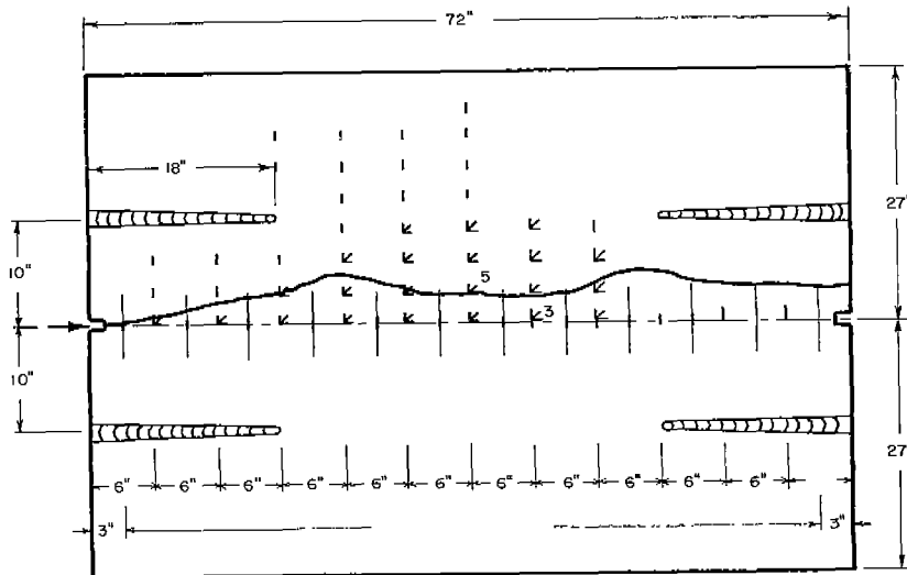
FIG. 9. PLATE LAYOUT--TEST 50.
