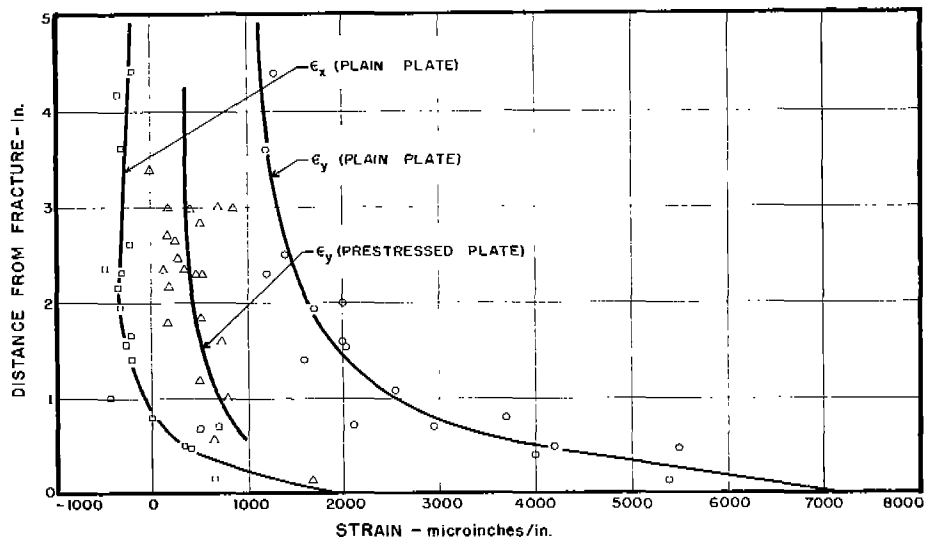
FIG. 19. PEAK STRAIN VS. DISTANCE FROM PROPAGATING FRACTURE IN PLAIN AND PRESTRESSED WIDE PLATE TESTS.
