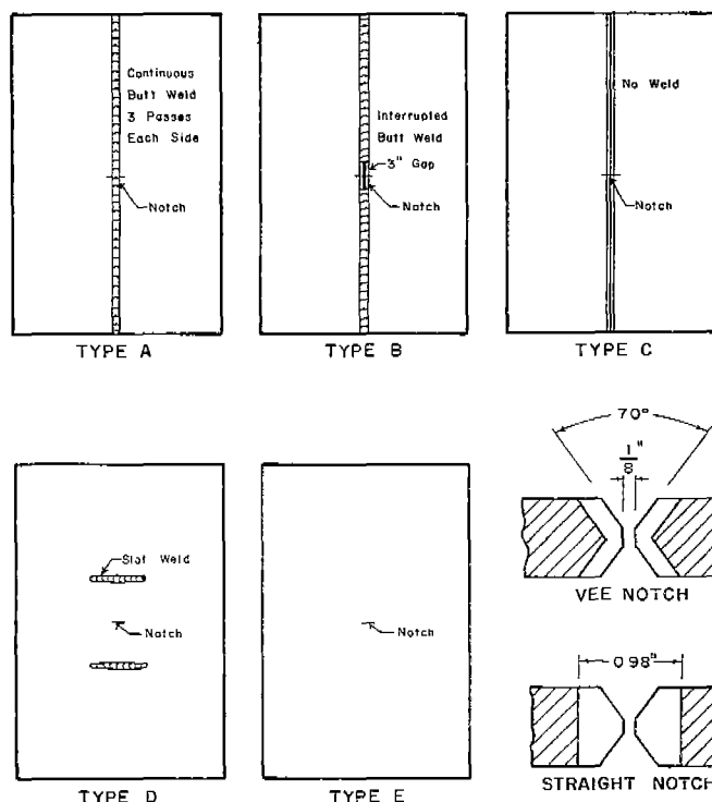
FIG. 12. SPECIMEN TYPES AND NOTCH DETAILS.
