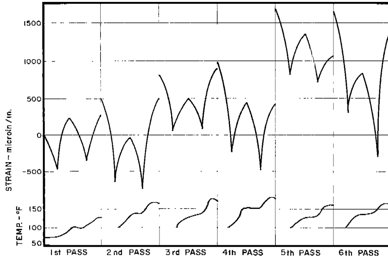
FIG. 13. STRAIN AND TEMPERATURE VARIATION DURING PREPARATION OF TYPE B SPECIMEN.
