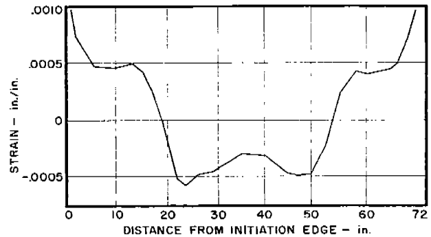
(b) AVERAGE LONGITUDINAL RESIDUAL STRAIN
