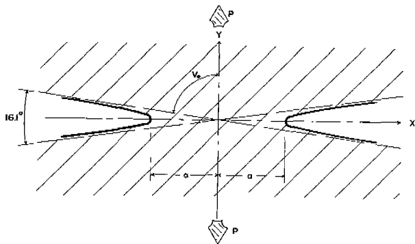
FIG. 17. MODEL USED IN STRESS ANALYSIS
