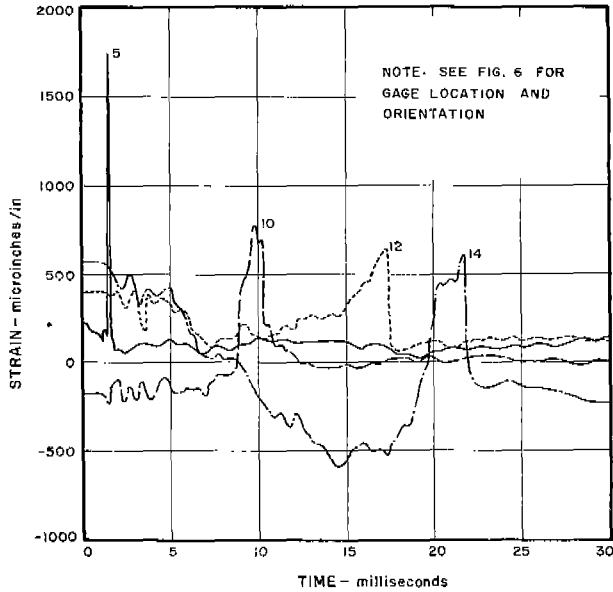
FIG. 8. TYPICAL STRAIN-TIME RECORDS-- TEST 46. oriented strain gages located at the positions indicated in Fig. 6.
