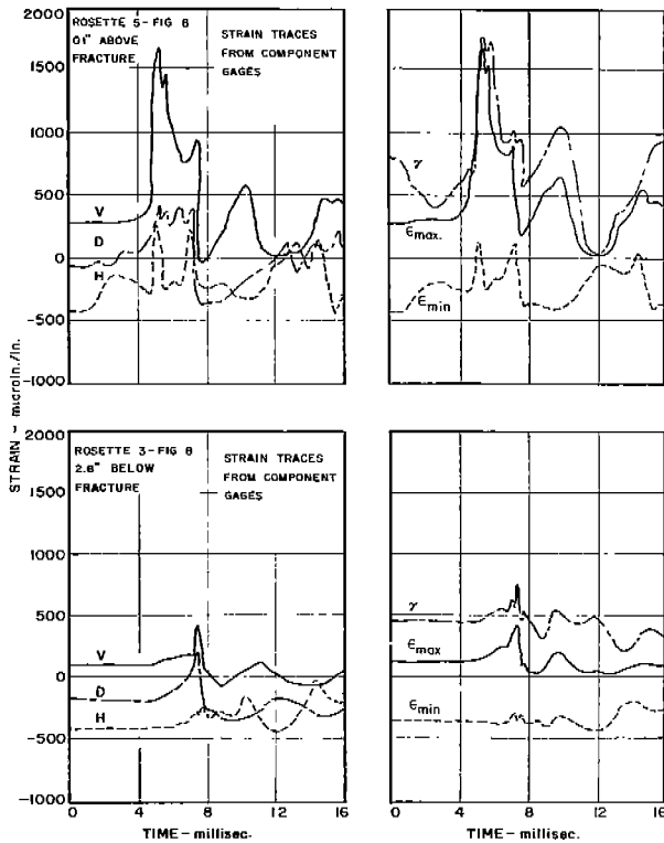
FIG. 10. STRAIN-TIME TRACES AND COMPUTED PRINCIPAL STRAINS--PRESTRESSED PLATE TEST 50.
