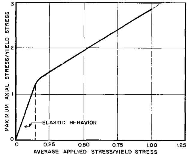
FIG. 18. MAXIMUM AXIAL STRESS AT NOTCH TIP VS. APPLIED STRESS.
