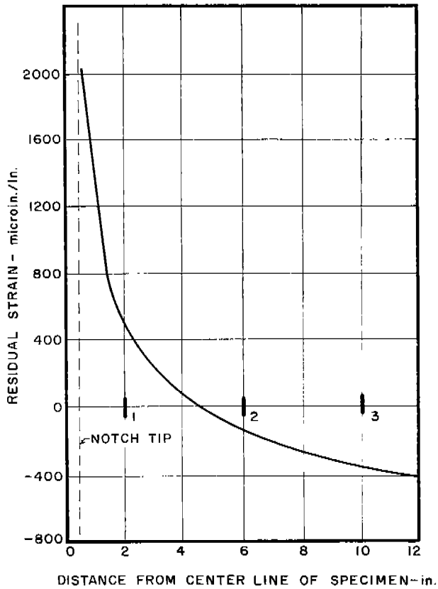
FIG. 14. RESIDUAL STRAIN DISTRIBUTION ACROSS SPECIMEN--TEST 56.
