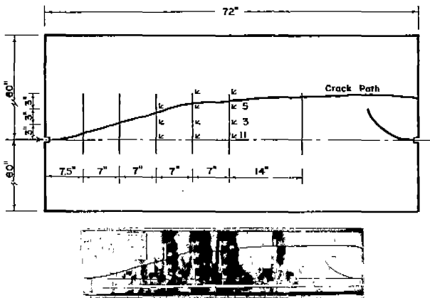
FIG. 2. PLAIN PLATE--TEST 39.
