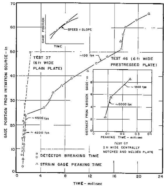
FIG. 7. FRACTURE SPEEDS ACROSS PLATE WIDTHS--TESTS 37, 46, AND 67.
