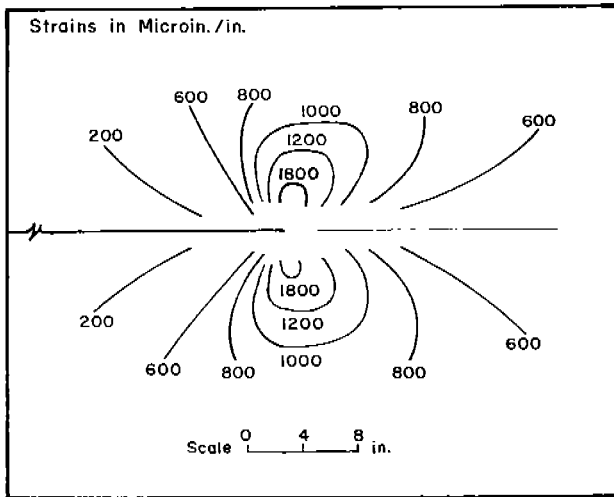
FIG. 4. MAJOR PRINCIPAL STRAIN CONTOURS.
