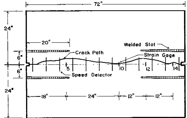
(a) PLATE LAYOUT AND FRACTURE PATH
