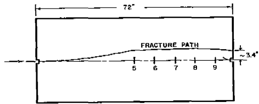
(a) PLATE LAYOUT AND FRACTURE PATH
