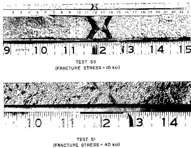
FIG. 16. FRACTURE TEXTURES--TESTS 51, and 53.
