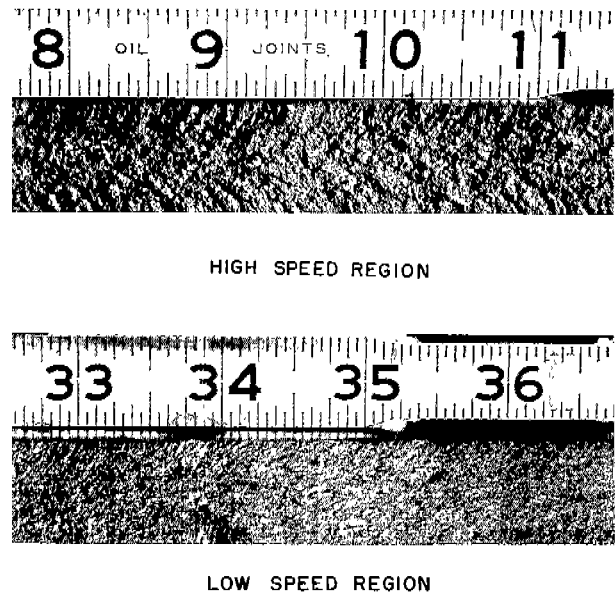
FIG. 11. FRACTURE TEXTURE--TEST 50.
