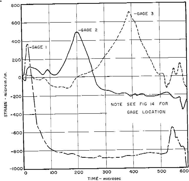
FIG 15. STRAIN-TIME RECORDS--TEST 56.
