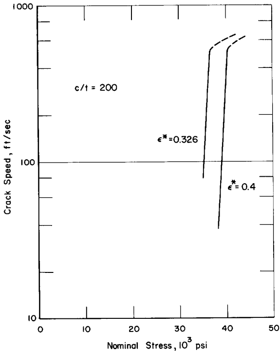
Fig. 15. Influence of Nominal Stress on Steady-State Crack Speed in Mild Steel (Curves 1.10, Fig. 1d and Table 1).
