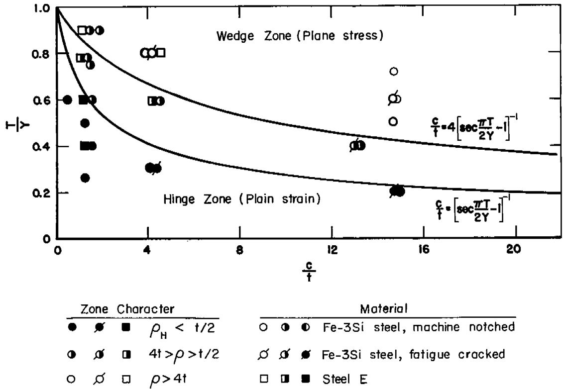
Fig. 7. Influence of Stress Level, Crack Length, and Thickness on the Character of the Plastic Zone in Fe-3Si Steel and Steel E.
