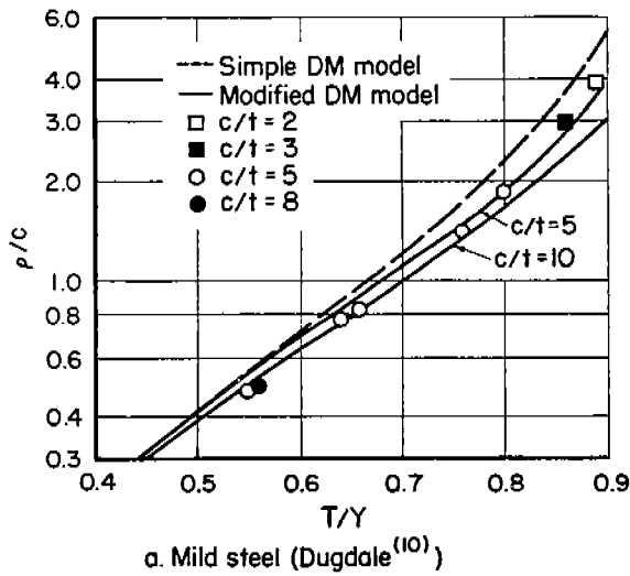
Fig. 11. Comparison of the Measured and Calculated Plastic-Zone Sizes
