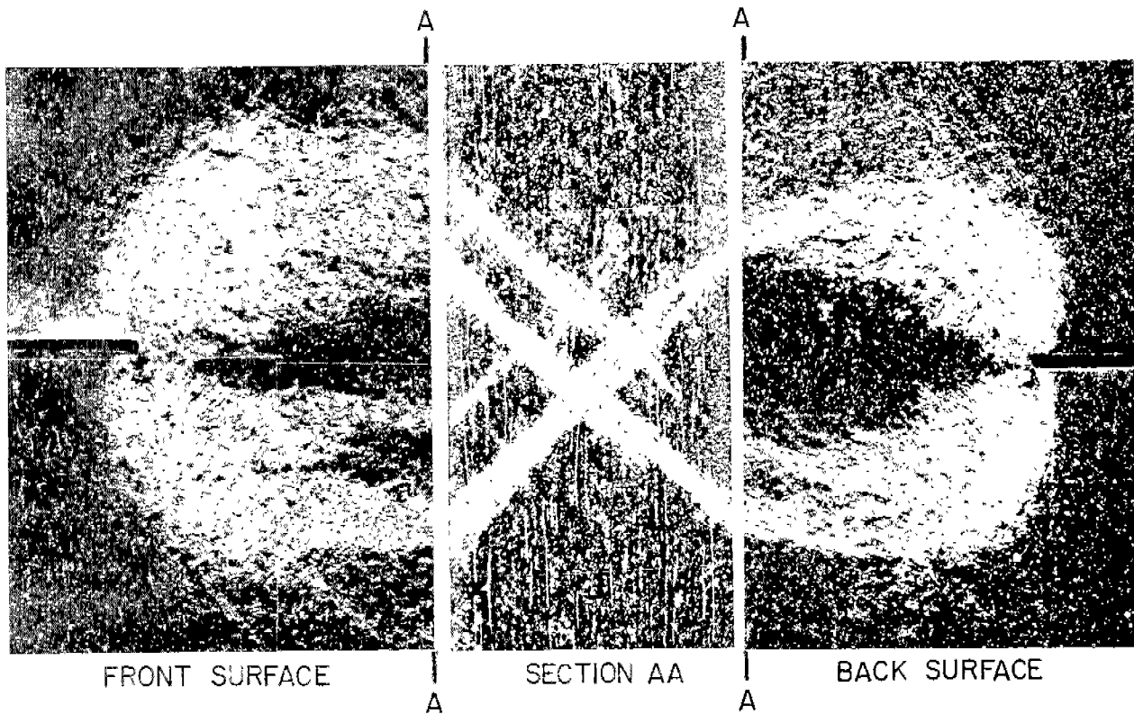
FRONT SURFACE SECTION AA BACK SURFACE Fig. 4. Appearance of Plastic Zone on the Front Surface, Back Surface, and a Normal Section
