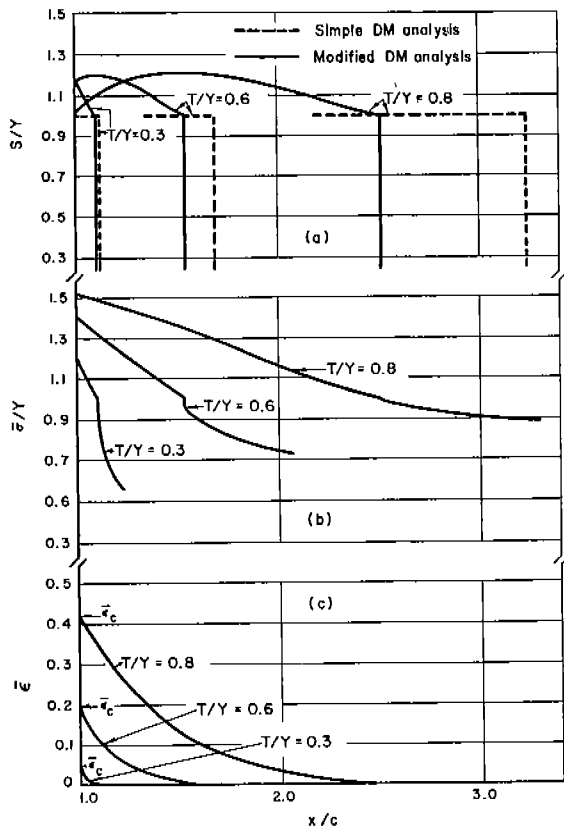
Fig. 10. Stress and Strain Gradients Calculated for a Crack in 4330 M Steel (Curve 1.4, Fig. 1c, Table 1, c = 3.75 in., t = 0.140 in.): (a) Internal tension (b) Stress (c) True strain (plastic)
