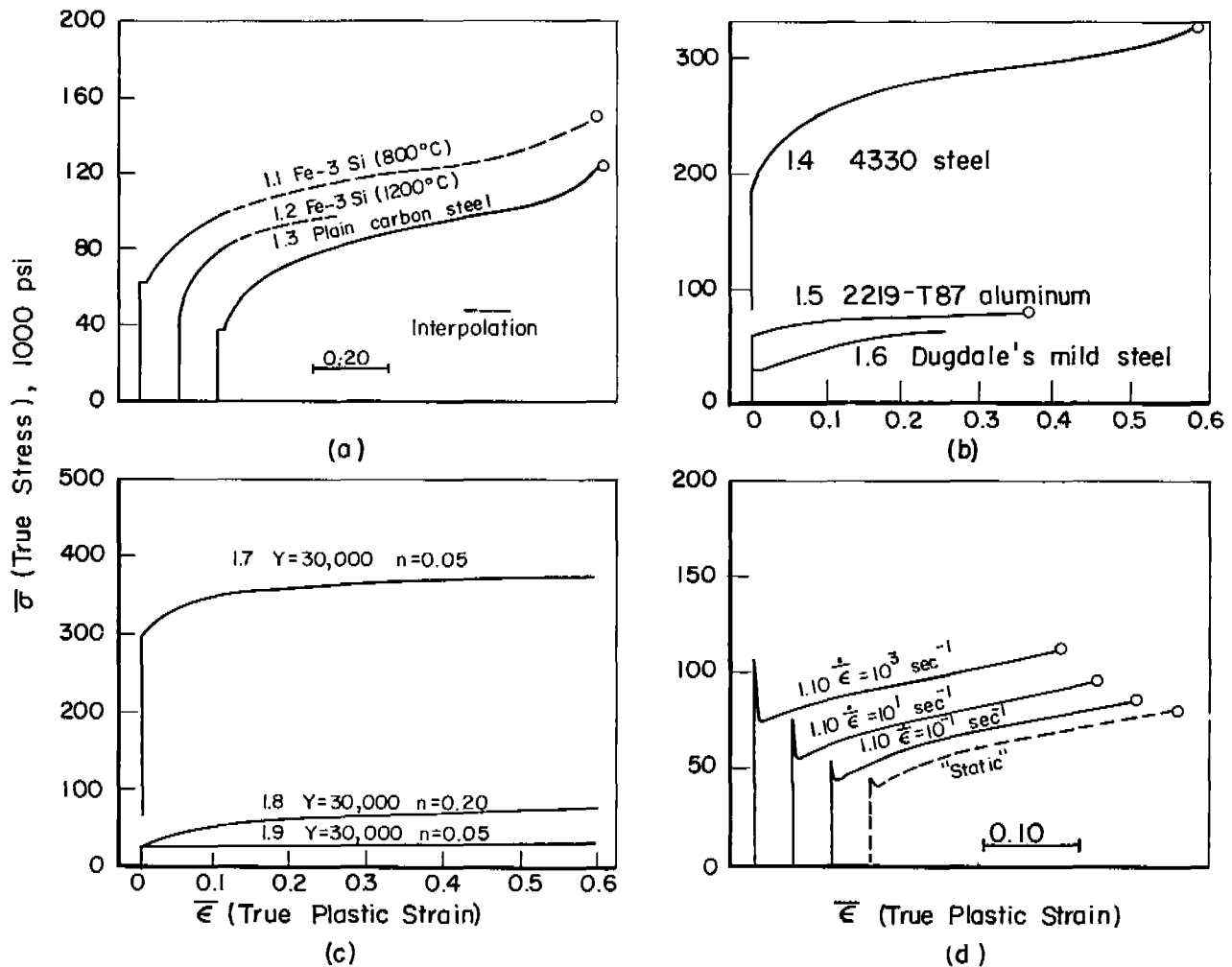
Fig. 1. True-Stresses/True-Strain Curves
