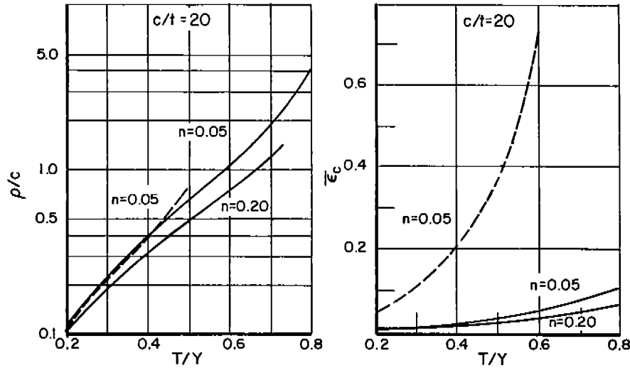
Fig. 12. Influence of strength level, work hardening, and ductility as shown by calculations for the hypothetical steels of Fig. 1c (Curves 1.7, 1.8, and 1.9, and Table 1)
