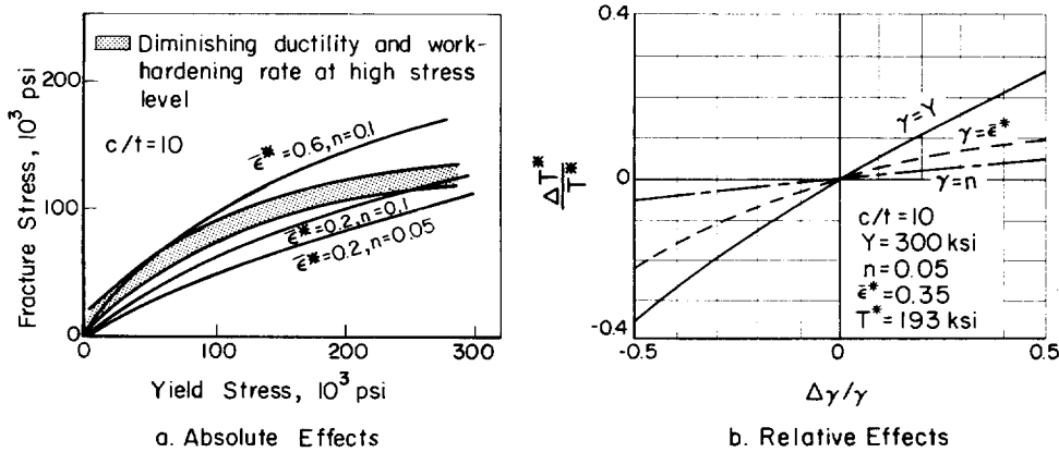
Fig. 14. Calculated Curves Showing the Influence of Yield-Strength Level, Work-Hardening Rate, and Ductility on the Fracture Stress of Hypothetical Steels (Equation 1, Table 1).
