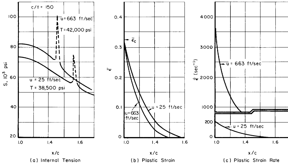
Fig. 16. Tension, Strain, and Strain Rate in Advance of a Propagating Crack in Mild Steel (Curves 1.10, Fig. 1d, Table 1).
