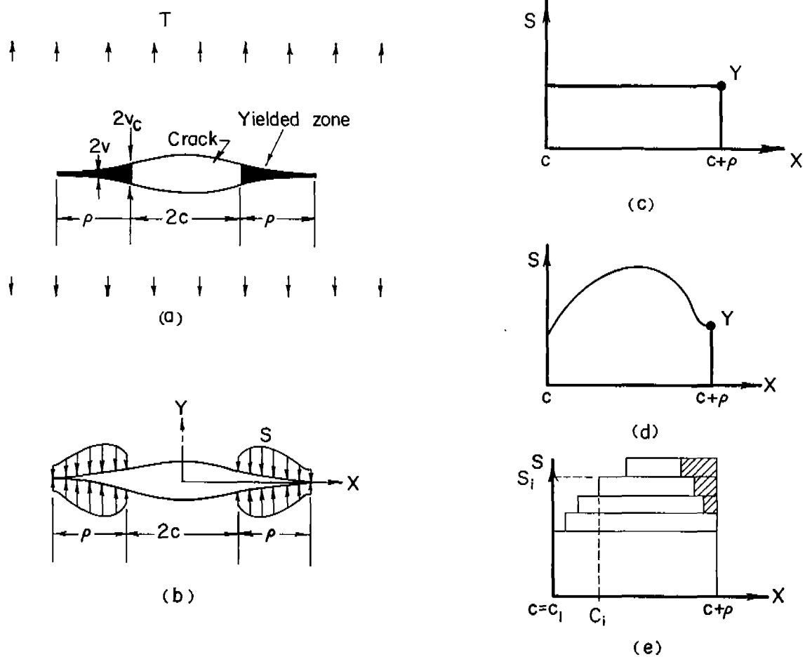
Fig. 9. The DM Model: (a) Crack with Wedge-shaped Plastic Zones, (b) Crack with "Equivalent" Internal Tension, (c) Uniform Tension Distribution of Dugdale, (d) Varying Tension Distribution, and (e) Stepwise Approximation of the Varying Tension Distribution.
