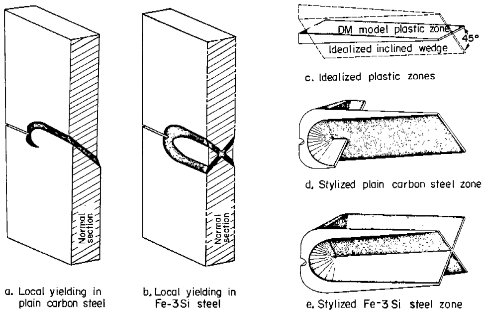
Fig. 8. Three-Dimensional Character of Plane-Stress Plastic Zones.
