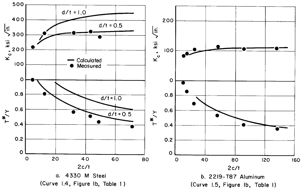
Fig. 13. Comparison of Calculated Fracture Stress and K_c Levels with Values Measured experimentally.
