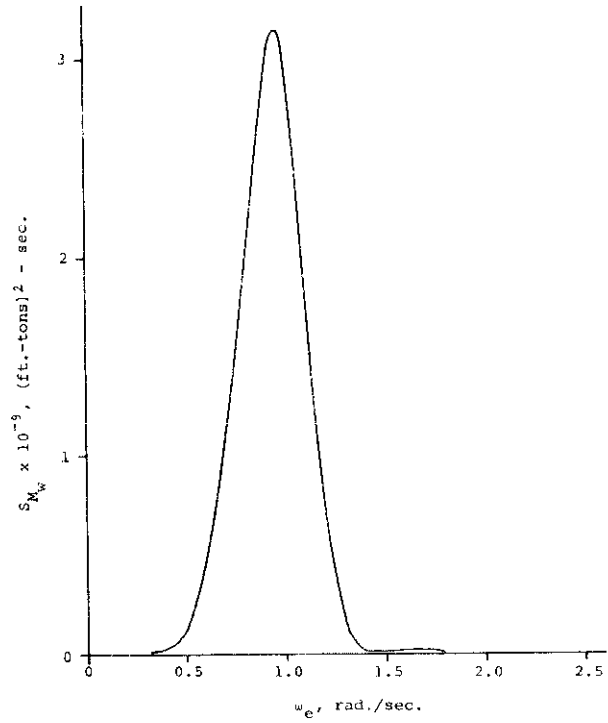
Fig. 5. Midship Wave-Induced Bending Moment Power Spectrum, SS WOLVERINE STATE, V = 12 kts., Sea State 7
