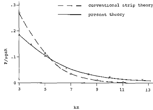
Fig. 13. Comparison of Theoretical Expressions for Sectional Wave Force on a Semicircle
