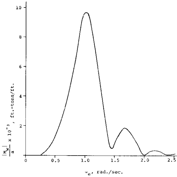
Fig. 4. Midship Wave-Induced Bending Moment Response Amplitude Operator, SS WOLVERINE STATE, V = 12 kts., Head Seas
