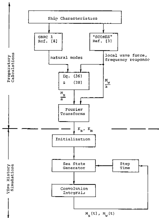
Fig. 12. Flow Chart for the Calculation of Springing and Wave Bending Moment Time Histories
