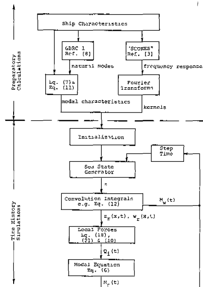
Fig. 3. Flow Chart for the Calculation of Slamming and Wave Bending Moment Time Histories
