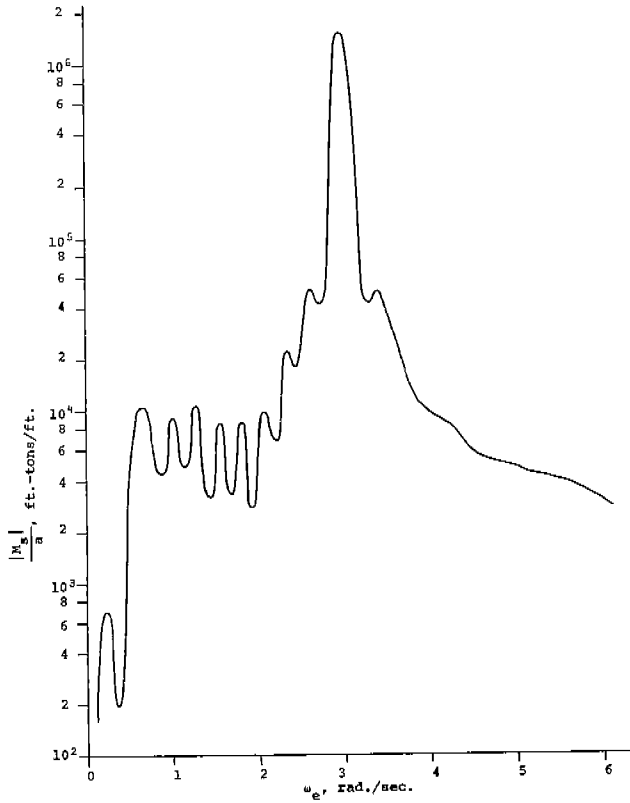
Fig. 7. Midship Springing Bending Moment Response Amplitude Operator, 200,000 dwt. Tanker, V = 16.7 kts.
