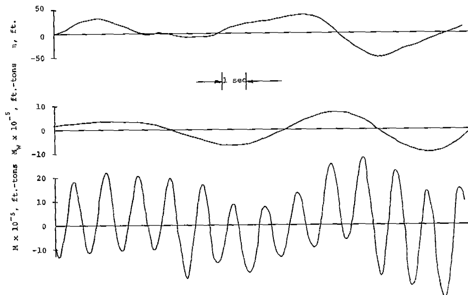
Fig. 2. Midship Bending Moment Time Histories, USS ESSEX, V = 13.8 .kts., Sea State 9
