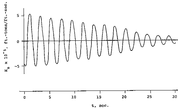
Fig. 9. Kernel Function for Midship Springing Bending Moment, 200,000 dwt. Tanker, V = 16.7 kts.
