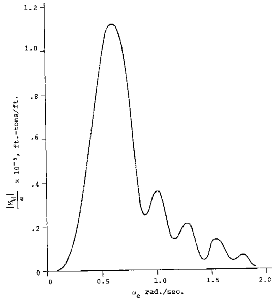
Fig. 8. Midship Wave-Induced Bending Moment Response Amplitude Operator, 200,000 dwt. Tanker, V = 16.7 kts.
