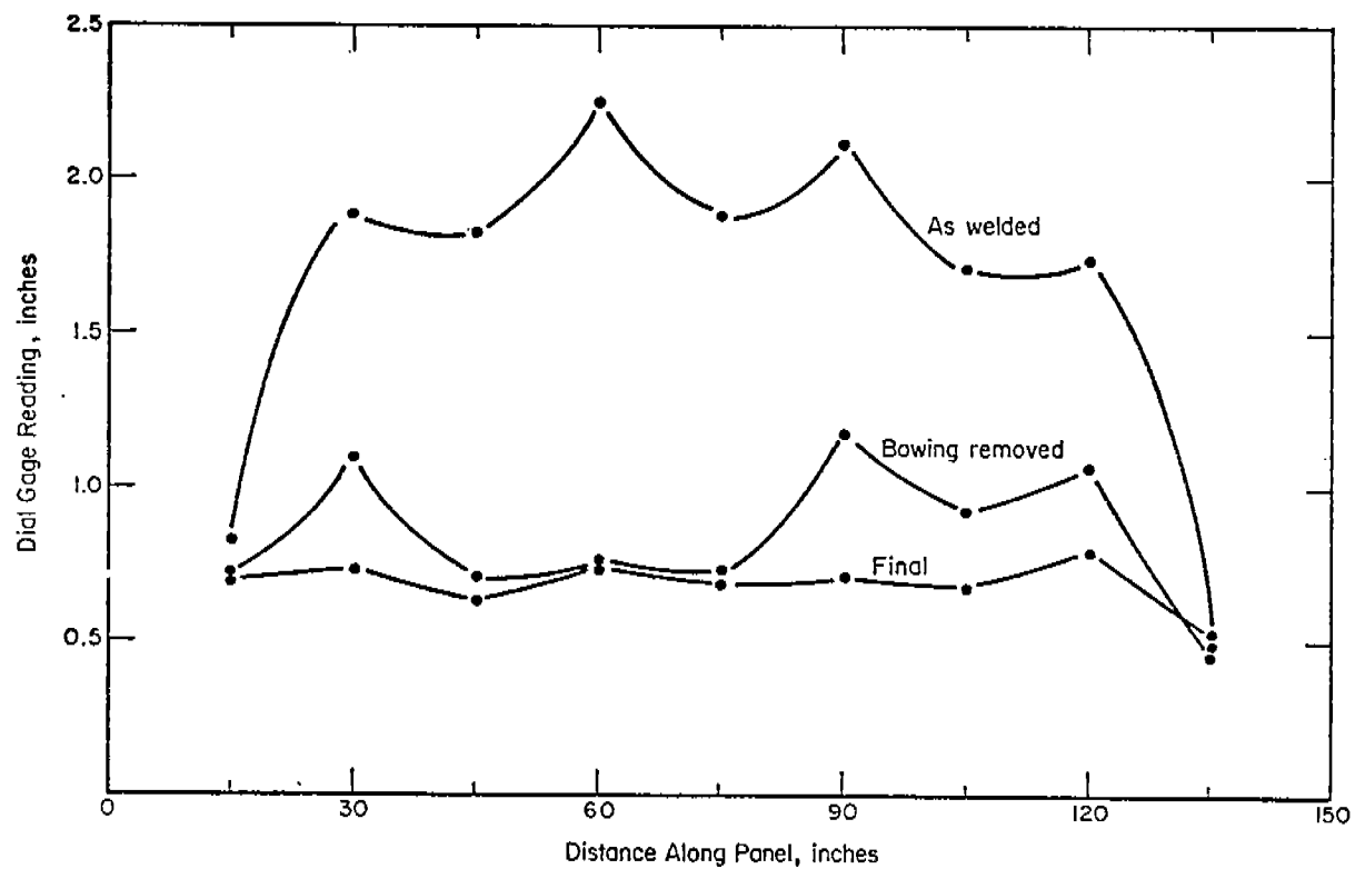
FIGURE 2. PANEL CONTOUR SHOWING EFFECTS OF FLAME STRAIGHTENING
