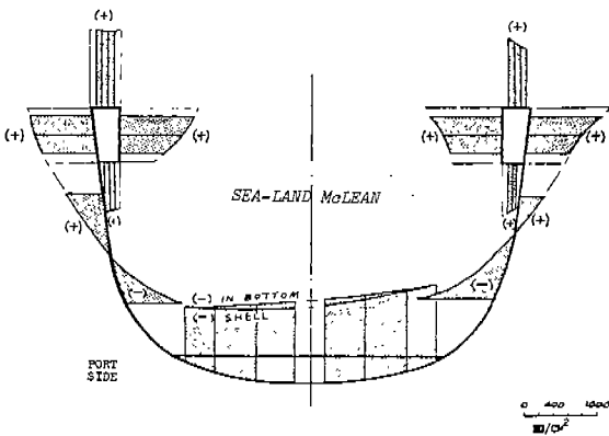
Fig. 17 - Longitudinal Stresses Due to Pure Vertical Bending Loads of Section Frame 222 - (Symmetric Loading) (First Loading Case).
