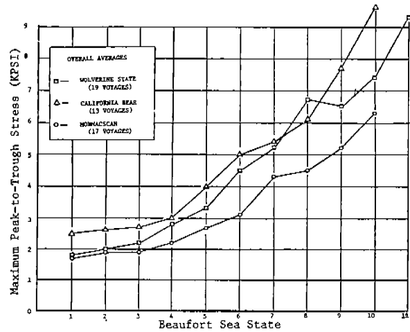
Fig. 4 - Average Plot of Maximum Peak-to-Trough Stress vs. Beaufort Sea State, 3 Ships.
