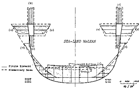
Fig. 16 - Total Longitudinal Stresses of Section Frame 222 (First Loading Case).
