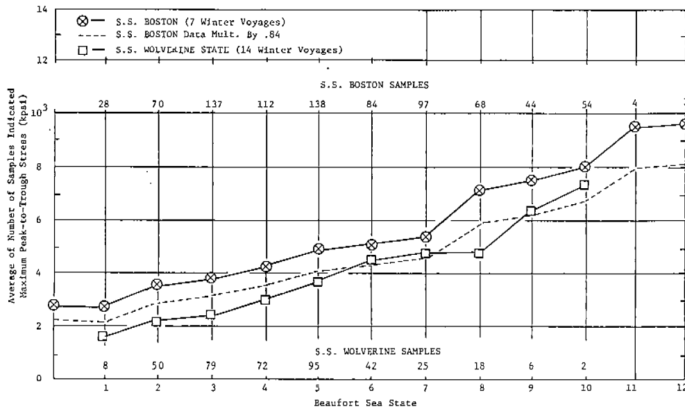
Fig. 6 - Vertical Longitudinal Bending Stress Comparison - S.S. BOSTON and S.S. WOLVERINE STATE .
