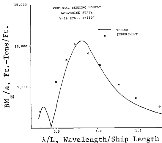
Fig. 8 - Comparison of Theory and Experiment, Vertical Bending Moment, \beta=150^\circ .
