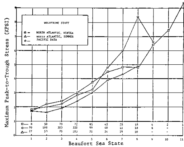
Fig. 5 - Average Plot of Maximum Peak-to-Trough Stress vs. Beaufort Sea State, S.S. WOLVERINE STATE
