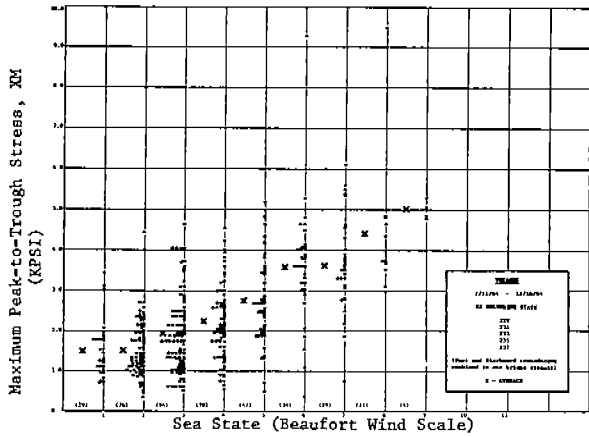
Fig. 2 - Maximum Peak-to-Trough Stress vs. Sea State S.S. WOLVERINE STATE .
