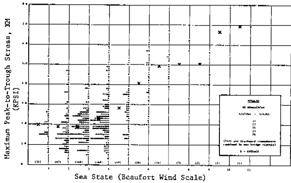
Fig. 3 - Maximum Peak-to-Trough Stress vs. Sea State S. S. MORMACSCAN .
