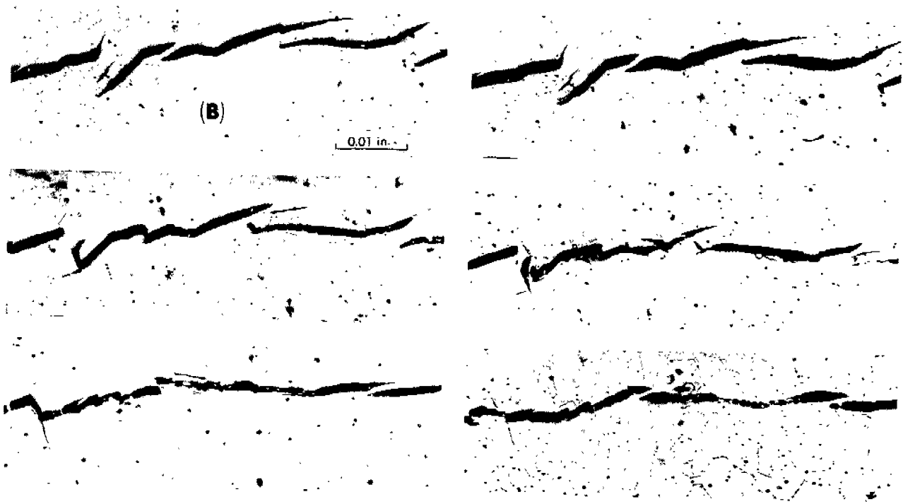
Fig. 10 - Interconnections Between Microcracks Revealed by Progressive Sectioning. The Depth of Each Section Below the Starting Section is Indicated.
