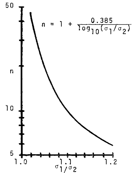
b. Determination of n
