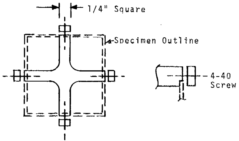
a. Cruciform (Schematic)
