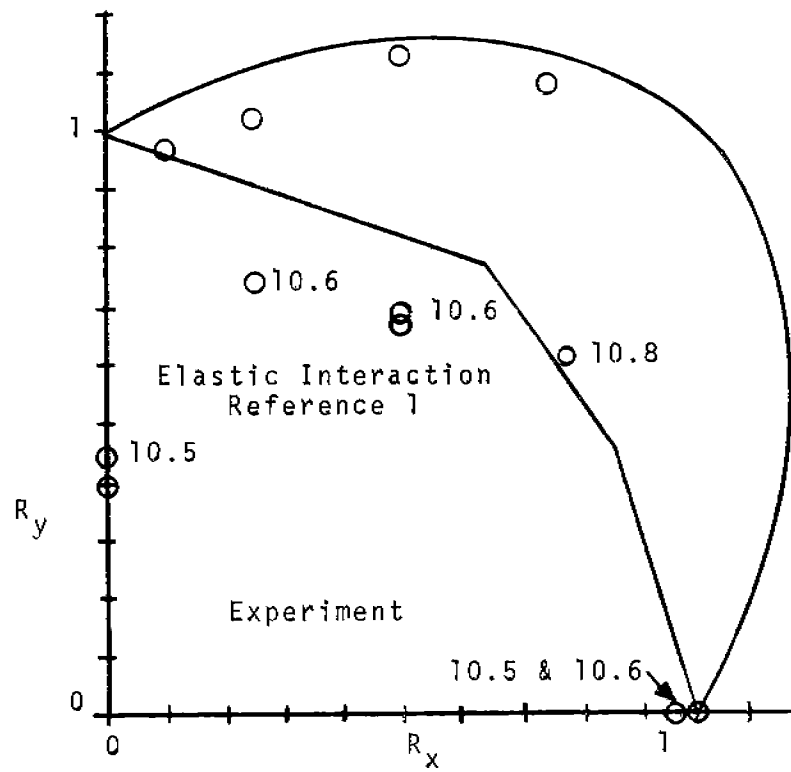
FIGURE 20 BIAxIAL STRENGTH COMPARISON, 1010 STEEL
