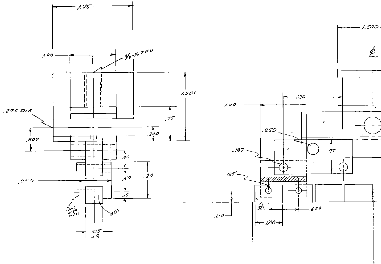
FIGURE I-3 WHIFFLETREE FOR TRANSVERSE LOADING OF 4130 SPECIMENS WITH b/t = 70
