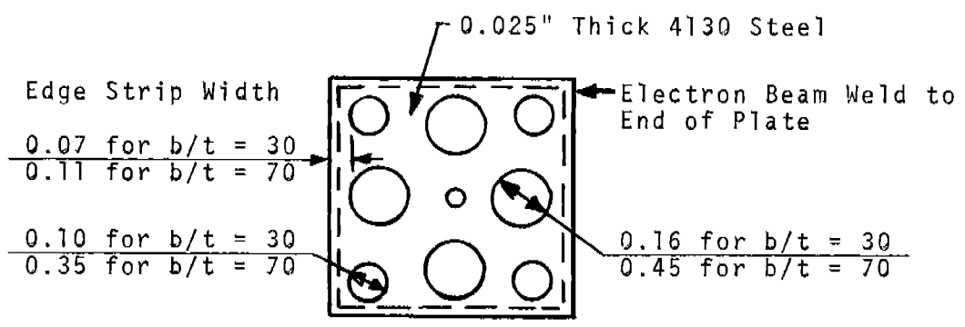
c. Final Design Perforated Cover Plate
