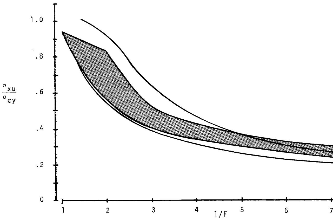
FIGURE 11 COMPARISON OF 4130 STEEL THEORETICAL LONGITUDINAL STRENGTH CURVES WITH HIGH-STRENGTH STEEL DATA
