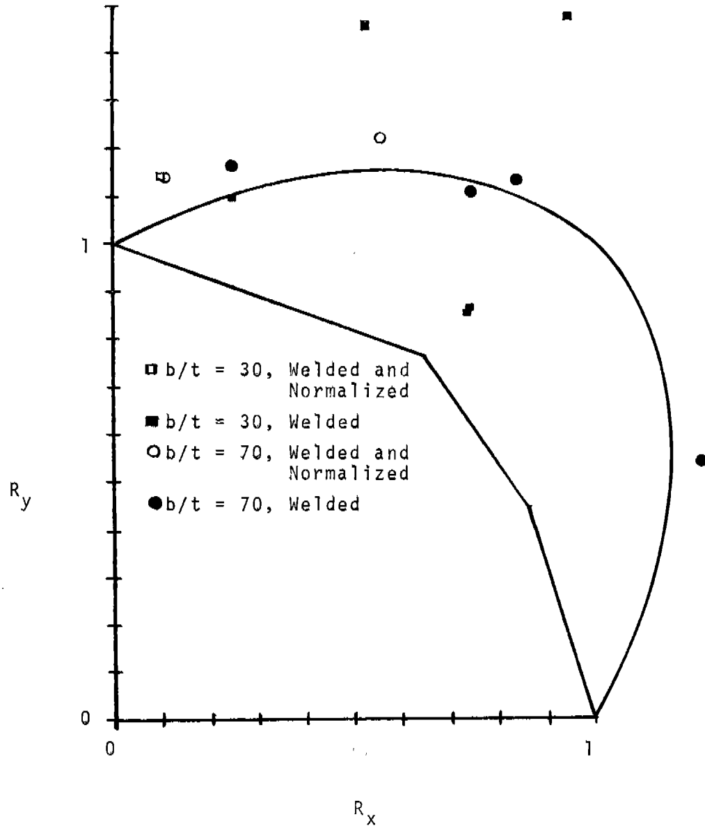
FIGURE 21 BIAxIAL STRENGTH COMPARISON, 4130 STEEL
