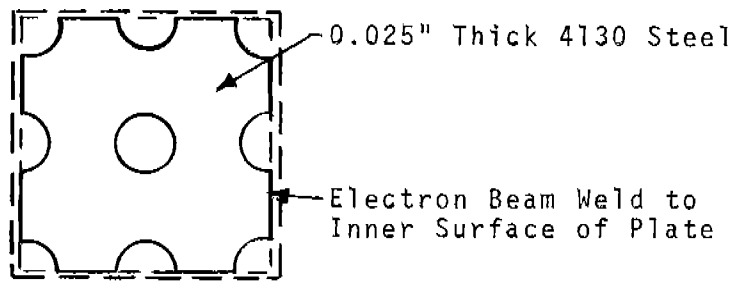
b. Locally Attached Plate (Schematic)
