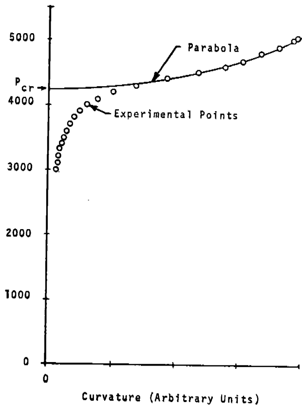
FIGURE 6 POST BUCKLING CURVATURE
