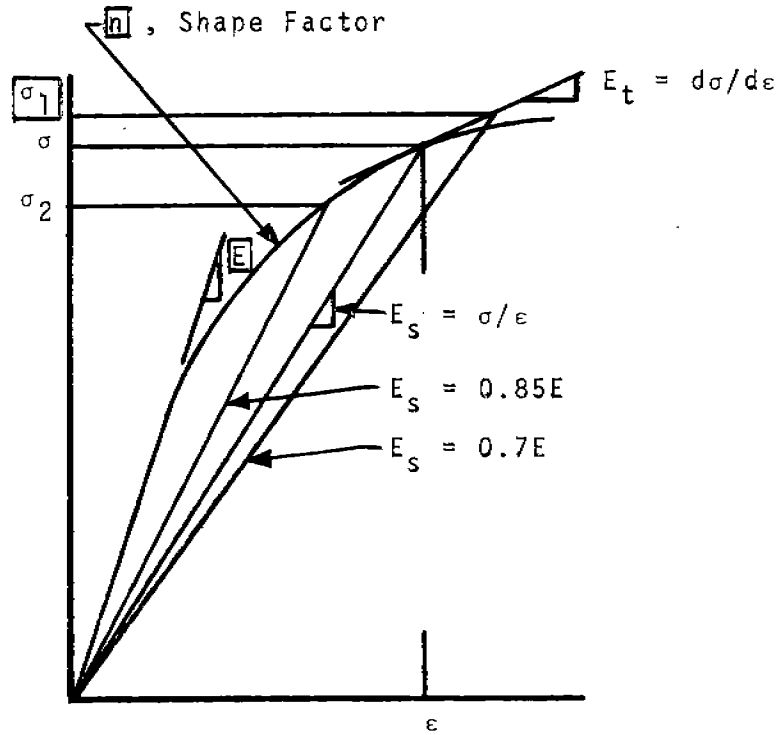
a. Curve Properties Showing 3 Parameters of Ramberg and Osgood
