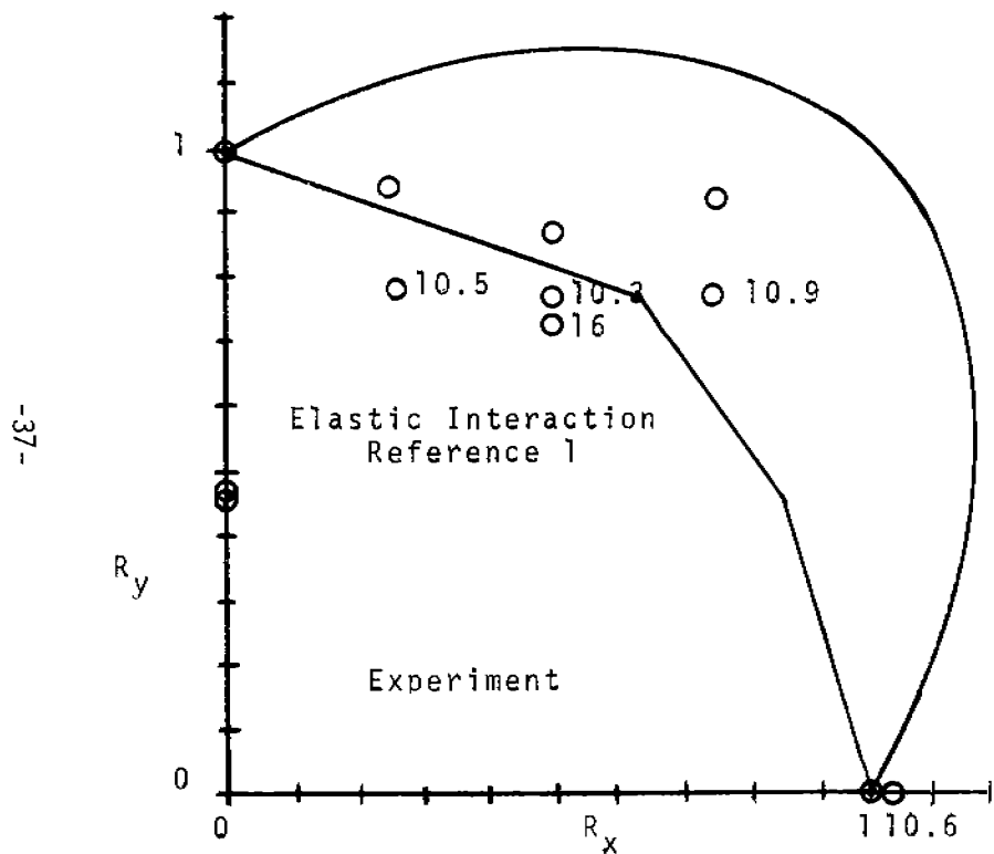
FIGURE 19 BIAxIAL STRENGTH COMPARISON, 1010 STEEL
