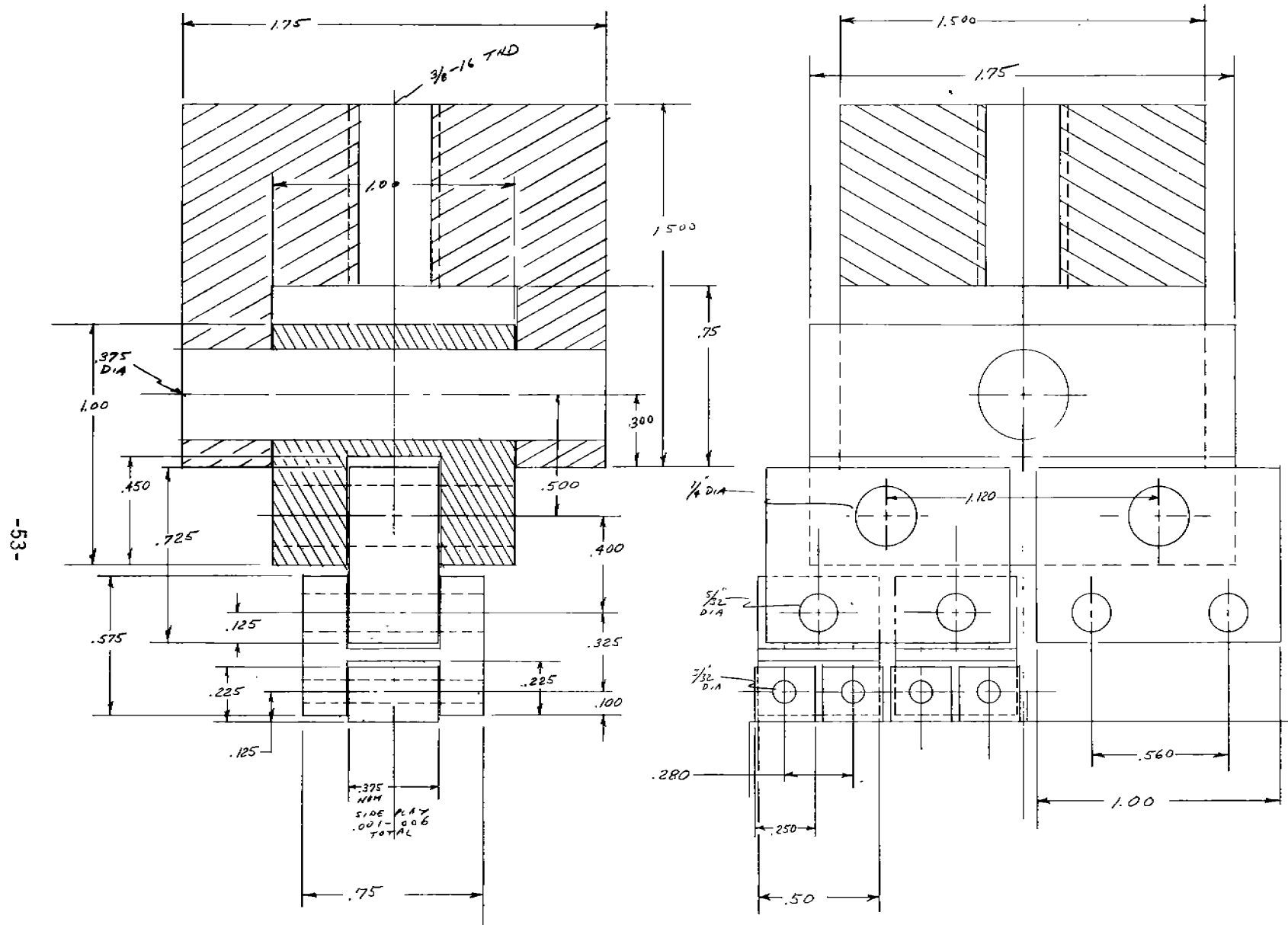
FIGURE I-4 WHIFFLETREE FOR TRANSVERSE LOADING OF 4130 SPECIMENS WITH b/T = 30
