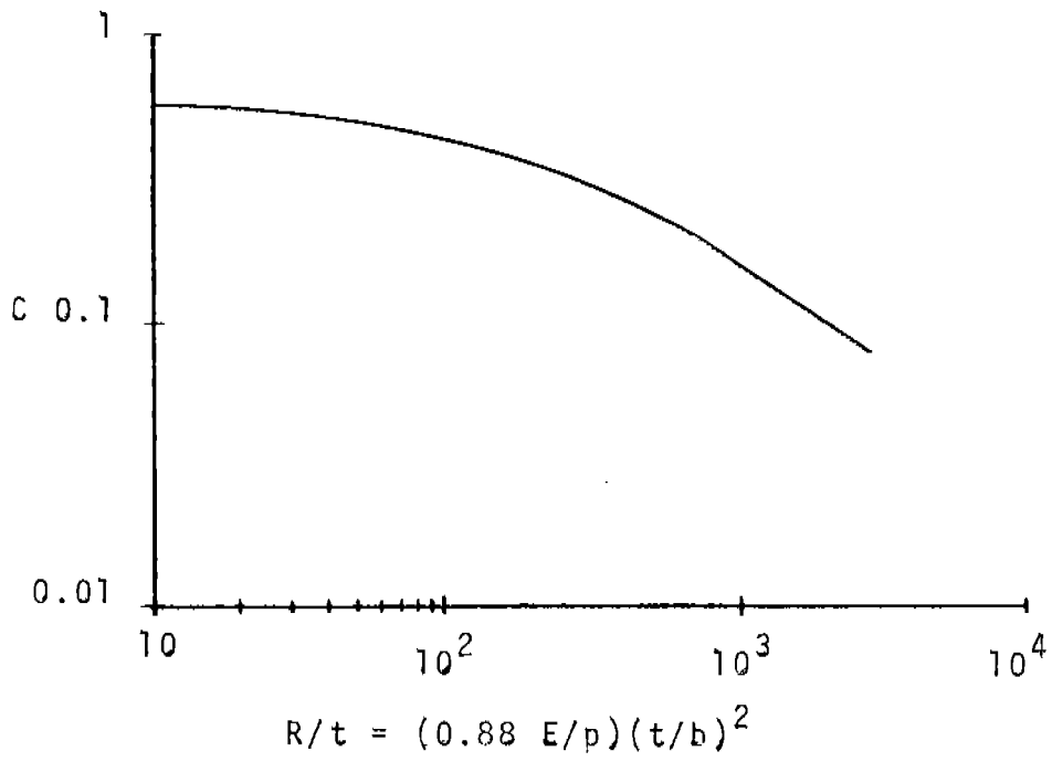
FIGURE 22 BUCKLING COEFFICIENT FOR NORMAL PRESSURE EFFECT, EQ. (26)
