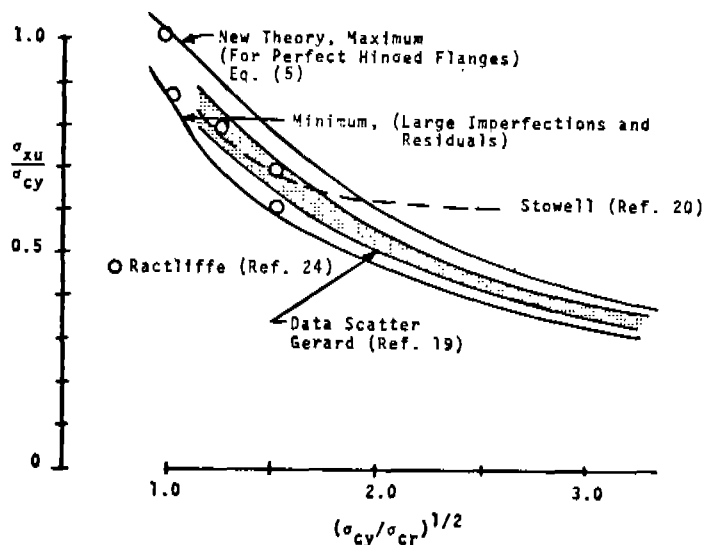
FIGURE 14 FLANGE STRENGTH COMPARISONS
