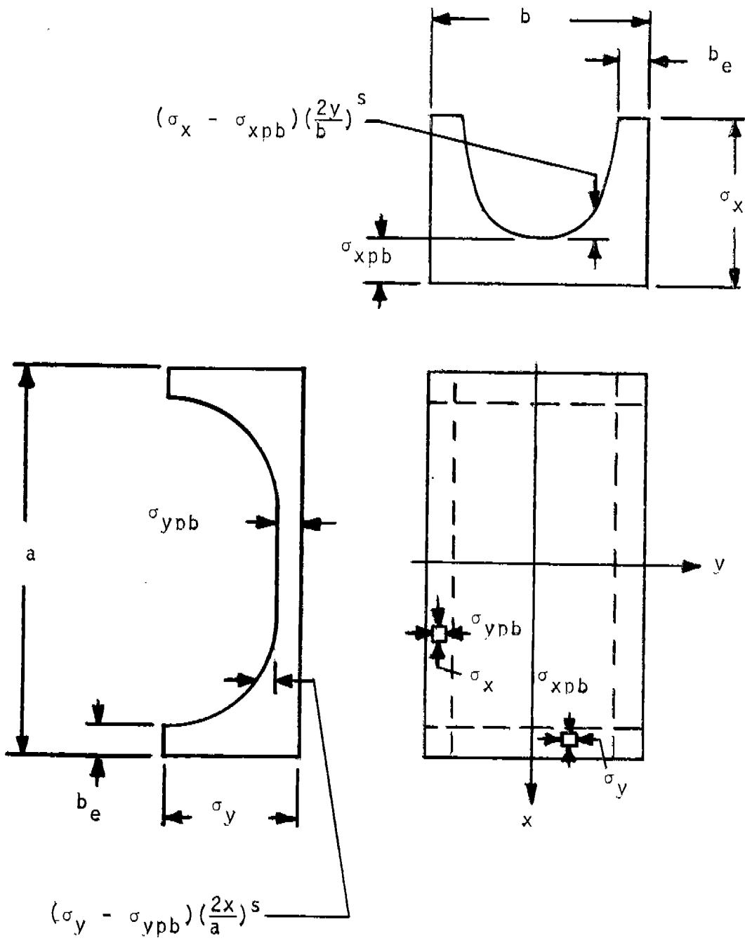
FIGURE 16 BIAXIAL POSTBUCKLING STRESS DISTRIBUTION
