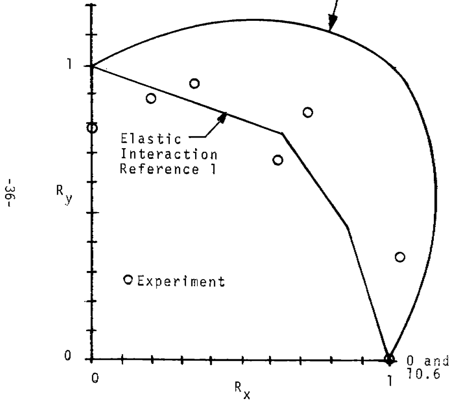
FIGURE 17 BIAXIAL STRENGTH COMPARISON, 1010 STEEL, b/t = 30
