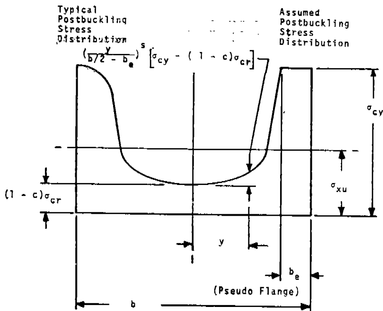
FIGURE 1 LONGITUDINAL POSTBUCKLING STRESS DISTRIBUTION IN SUPPORTED PLATES
