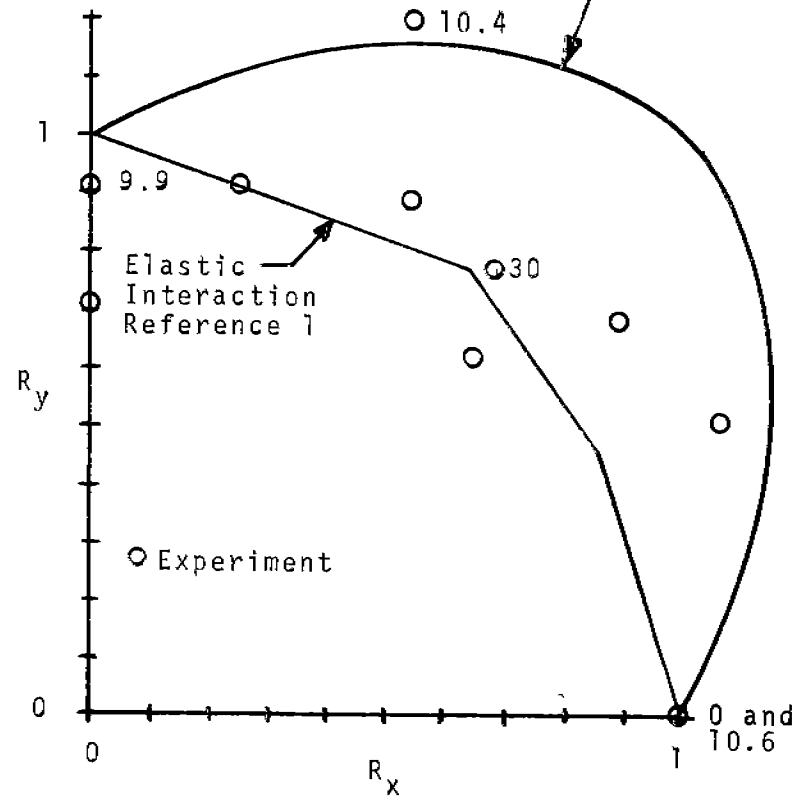
FIGURE 18 BIAXIAL STRENGTH COMPARISON, 1010 STEEL, b/t = 50
