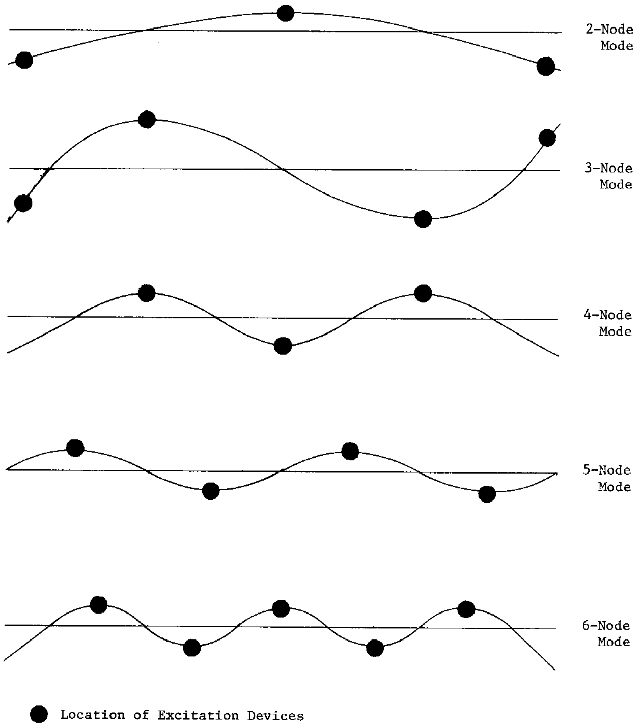
Figure 3-11 APPROXIMATE LOCATION OF EXCITATION DEVICES
