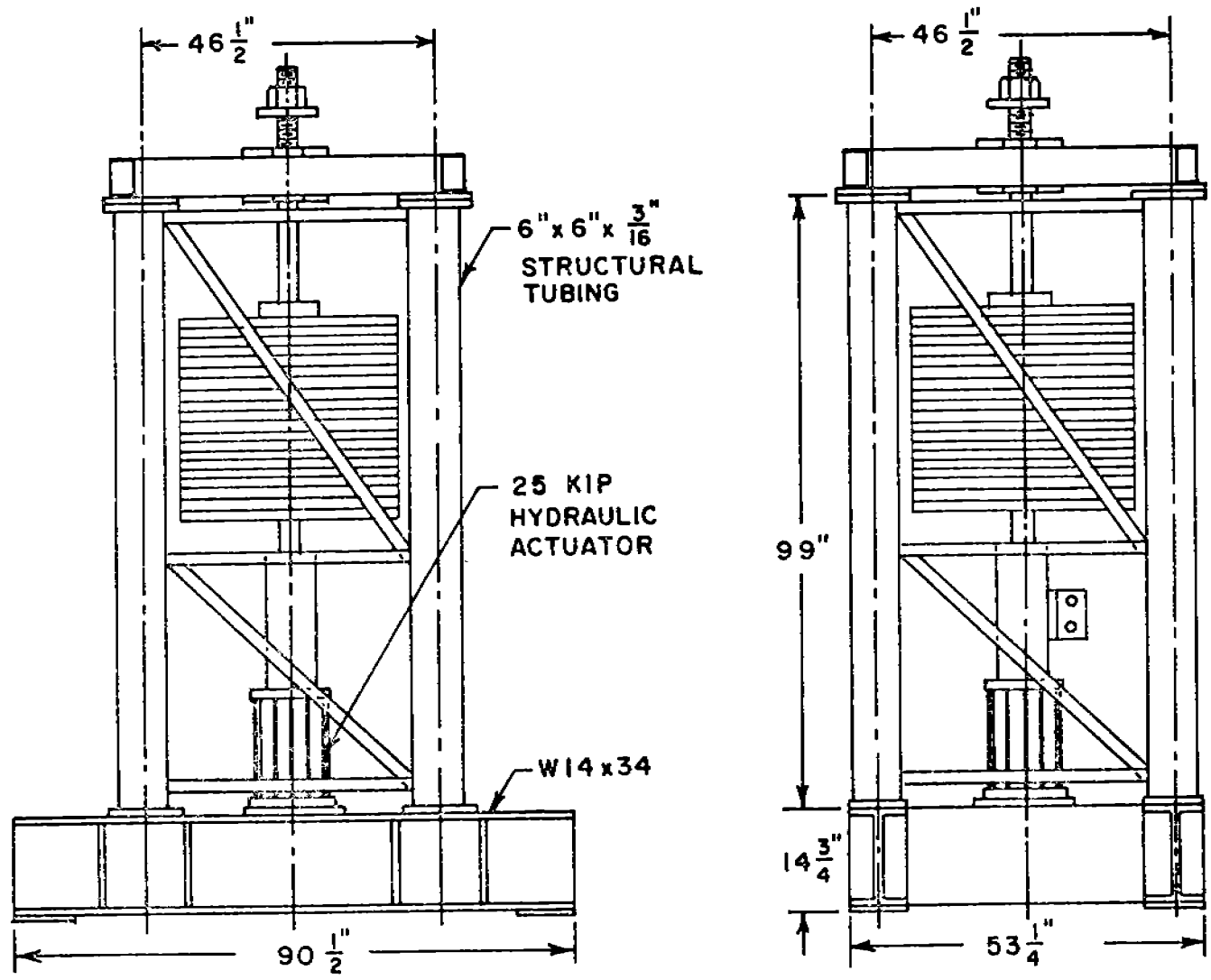
Figure 3-7 HYDRAULIC ACTUATOR AND LOAD DISTRIBUTION FRAME USED BY BALDWIN (Reference 3-5)
