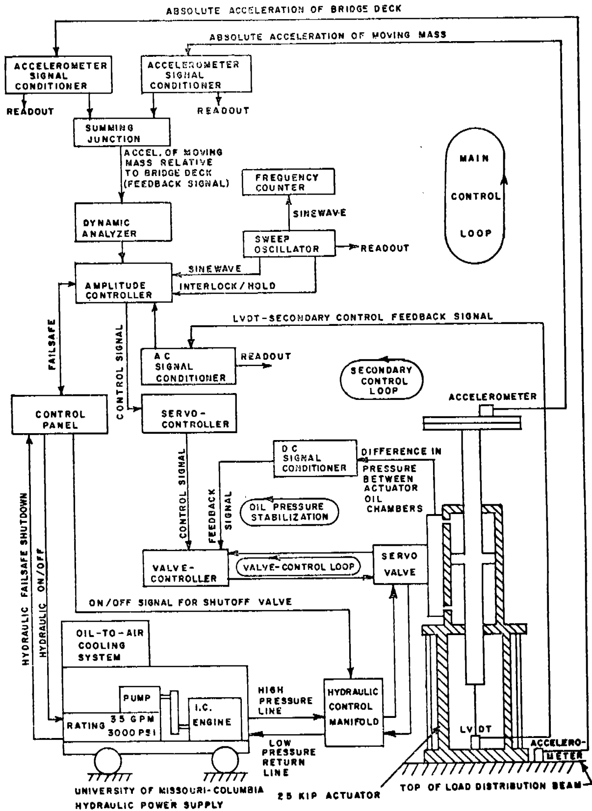
Figure 3-9 SCHEMATIC OF ELECTROHYDRAULIC VIBRATION EXCITATION SYSTEM USED DURING DYNAMIC TESTS OF A HIGHWAY BRIDGE (from Reference 3-5)
