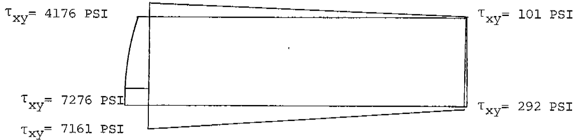
COMBINED SHEAR STRESSES
