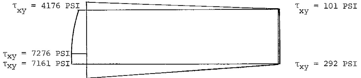
COMBINED SHEAR STRESSES
