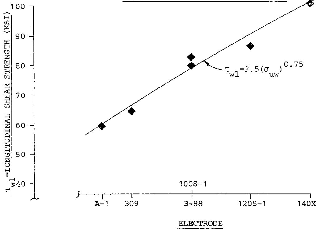
FIGURE 8 BARE ELECTRODE STRENGTH VALUES
