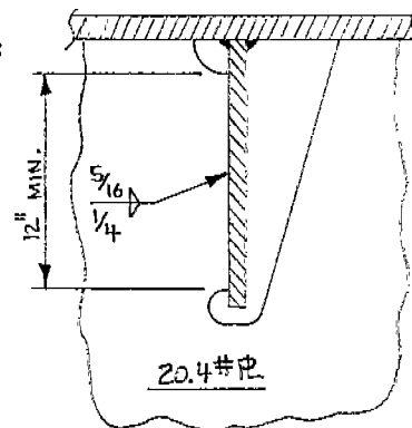
SECTION LKG. FWD
