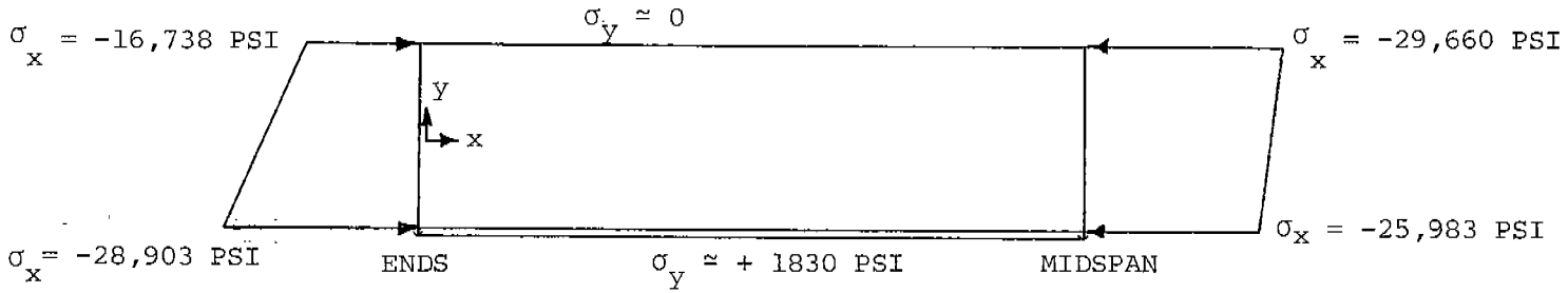
COMBINED NORMAL STRESSES
