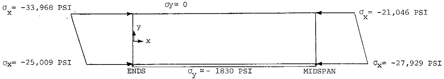
COMBINED NORMAL STRESSES
