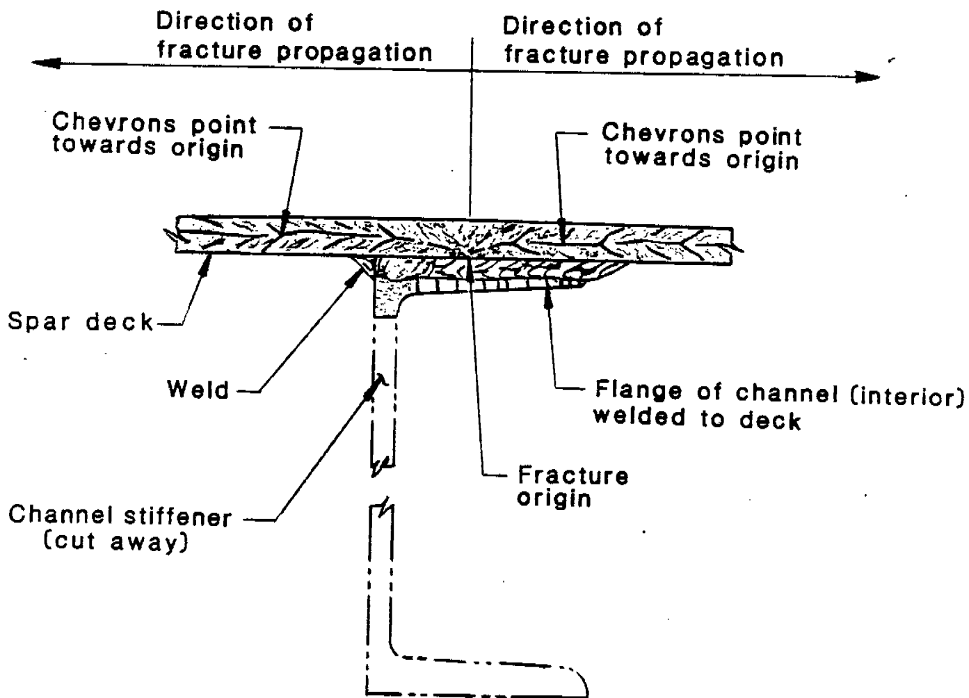
Figure 4-8. Location of the Fracture Origin in Sample No. 6.
