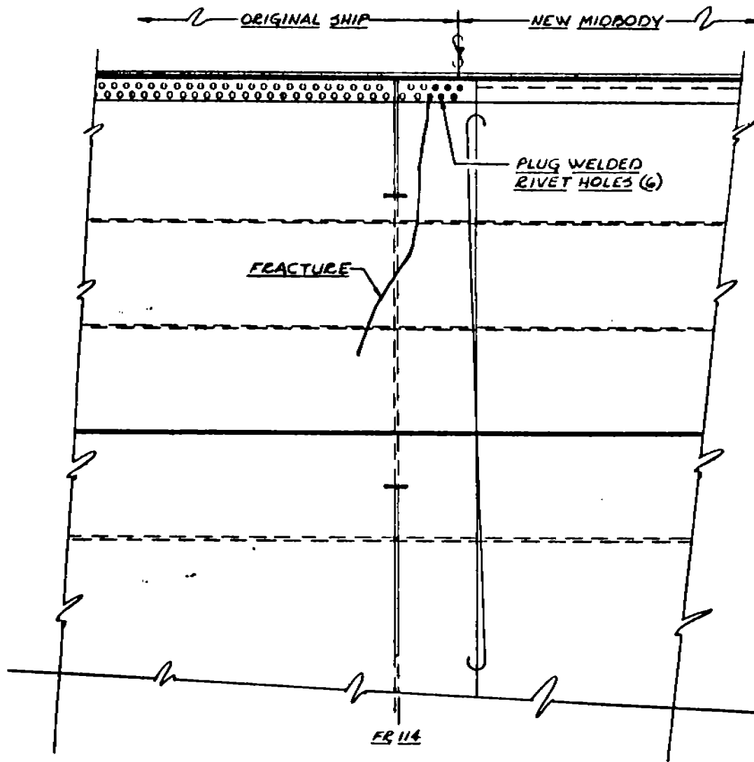
SKETCH C LONG'L BHD.
