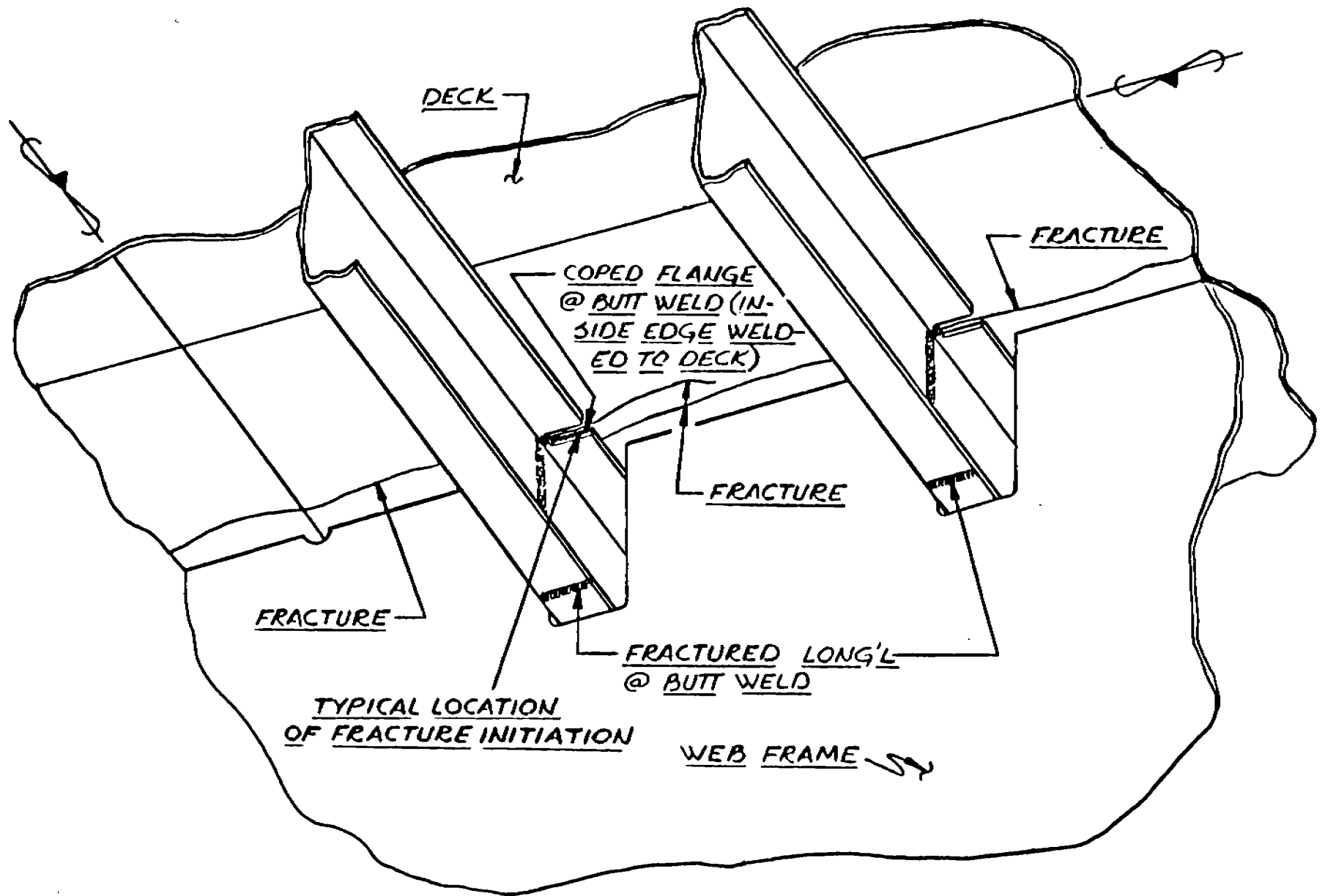
Figure 4-5. Construction Details Associated with the Initiation of the Fracture on the Great Lakes Bulk Carrier
