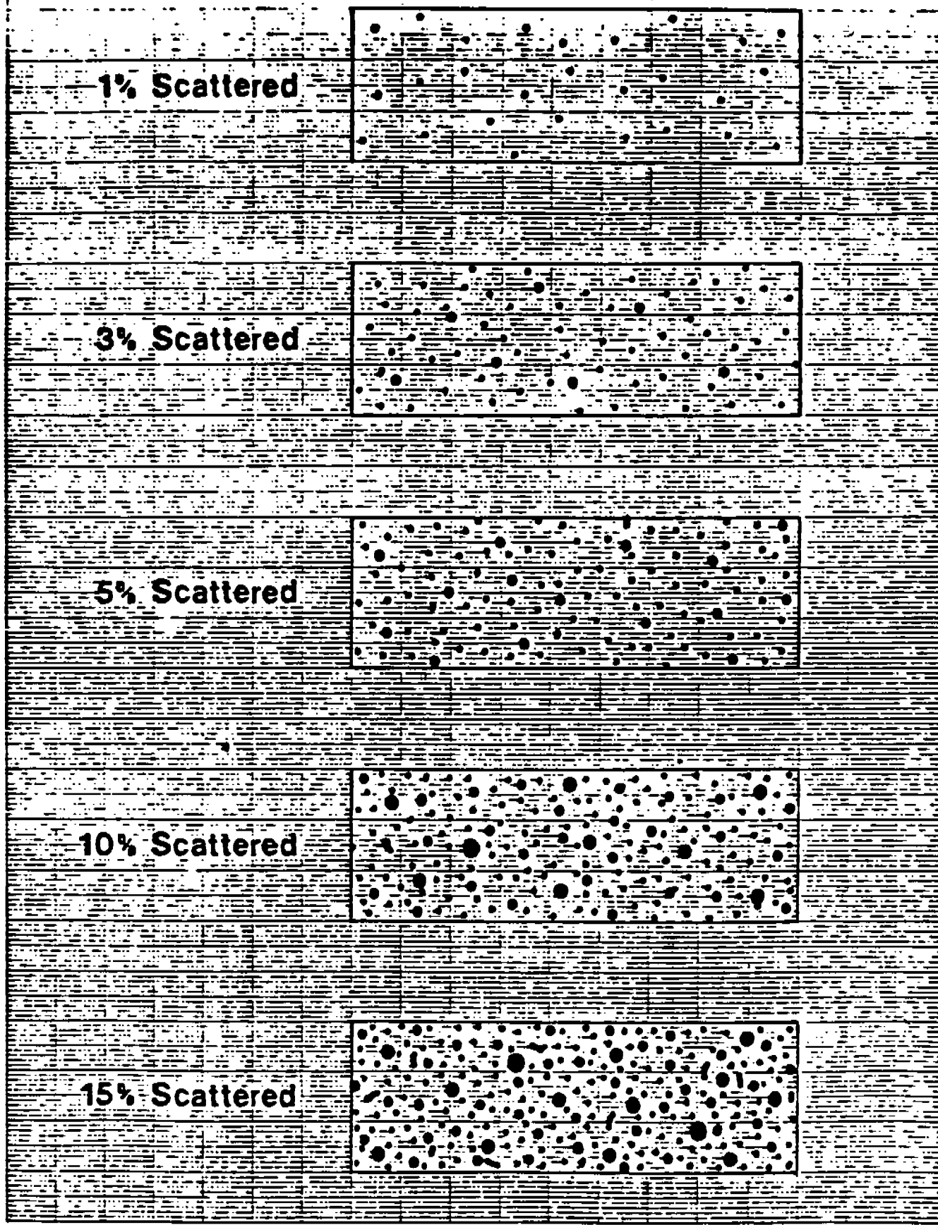
FIGURE 5-9 PITTING INTENSITY DIAGRAMS
