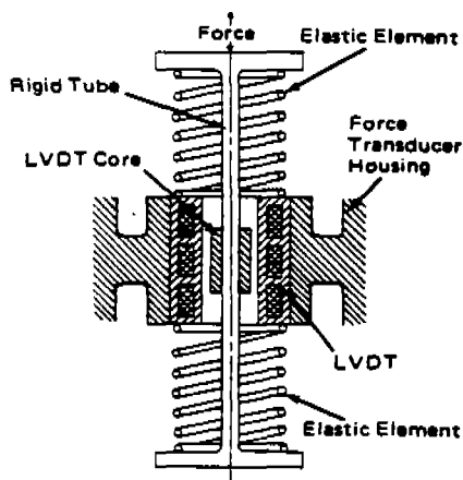
SCHMATIC DIAGRAM GRAM RANGE FORCE TRANSDUCER
