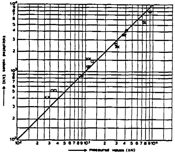
CALCULATED AND EXPERIMENTAL DATA OF F_y
