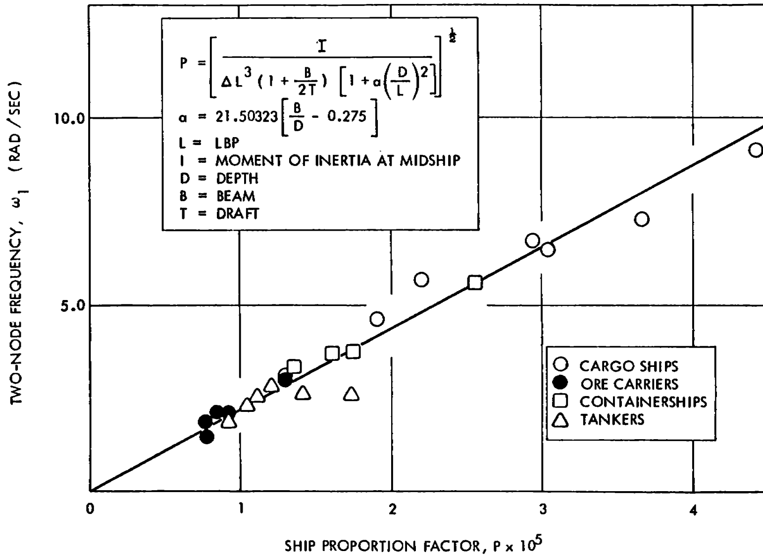
FIGURE 7 - EFFECT OF SHIP PROPORTIONS ON THE HULL FLEXIBILITY (REPRESENTED BY THE TWO-NODE FREQUENCY), FROM REF. 55
