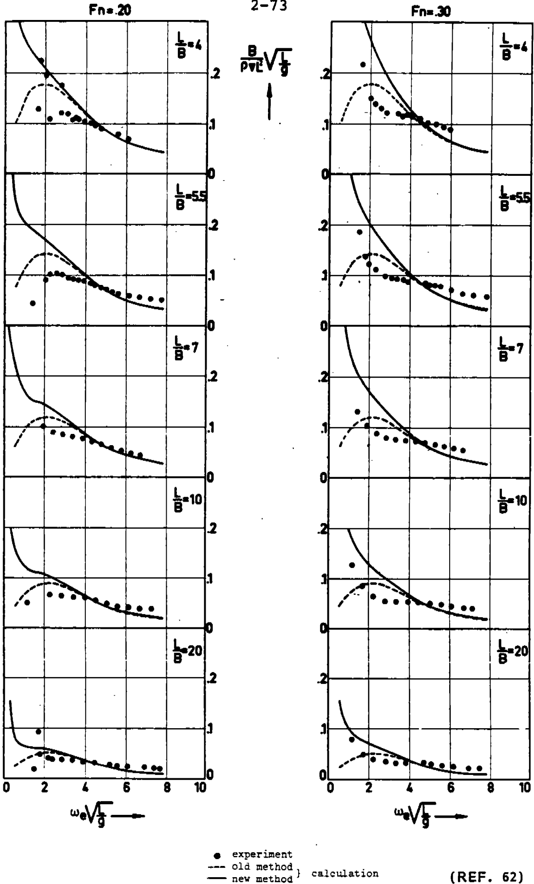
FIGURE 14 - PITCH DAMPING COEFFICIENT
