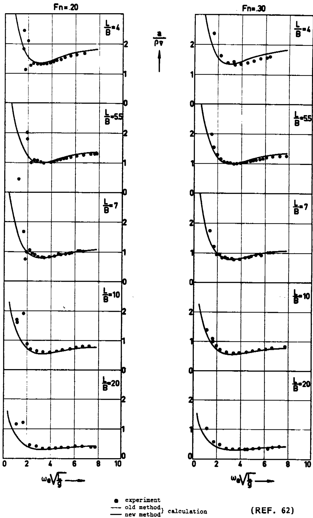
FIGURE 11 - ADDED MASS COEFFICIENT FOR HEAVE
