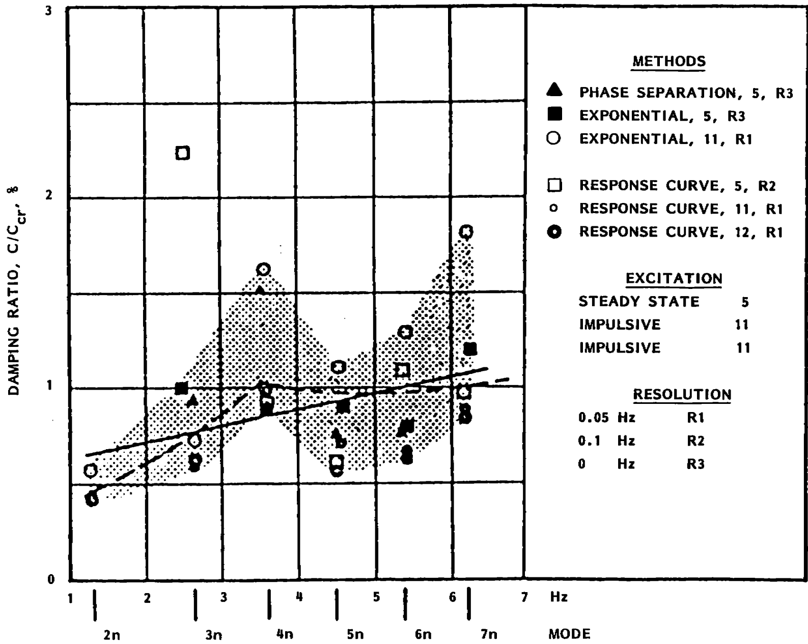
FIGURE 5 - COMPARISON OF DAMPING COEFFICIENTS DETERMINED BY STEADY STATE AND TRANSIENT (IMPULSIVE) EXCITATION (REF. 12)
