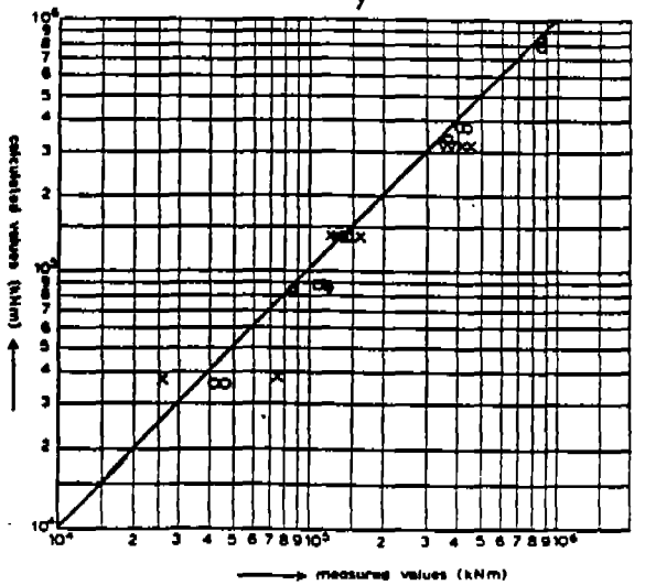
CALCULATED AND EXPERIMENTAL DATA FOR M_z
