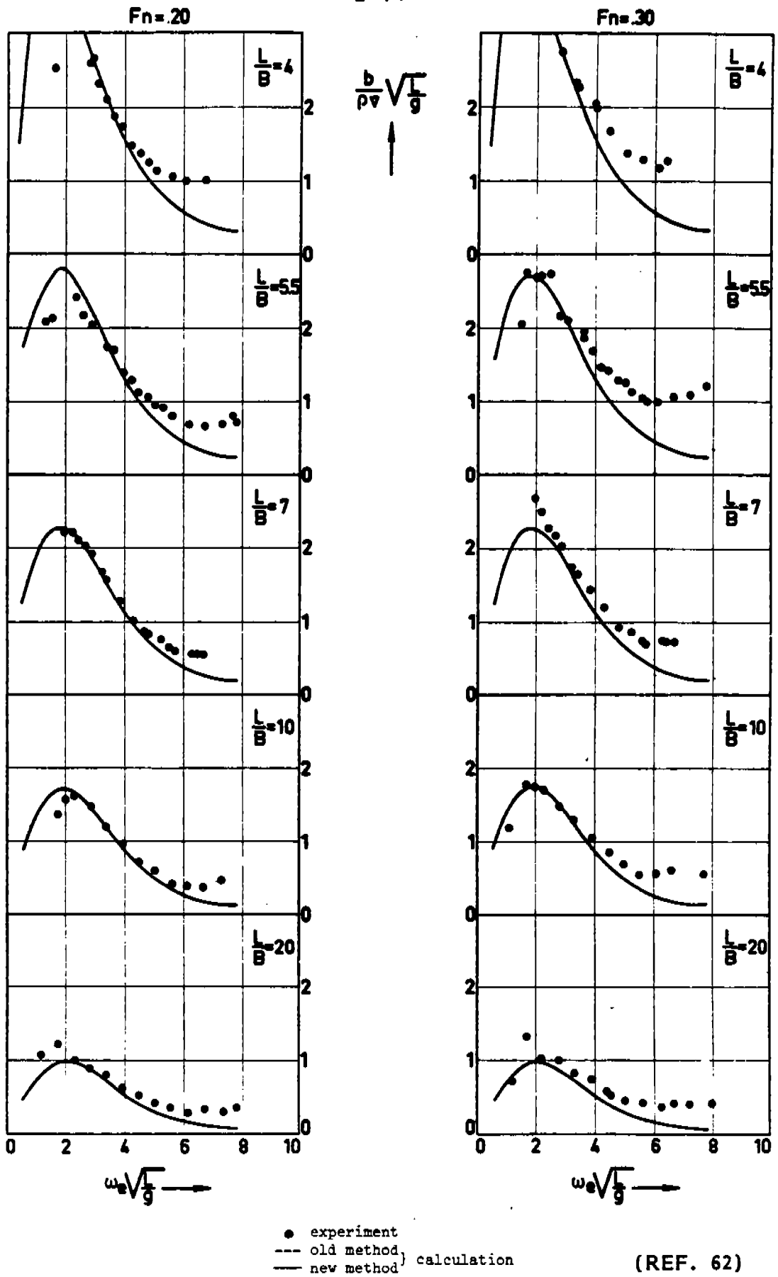
FIGURE 12 - HEAVE DAMPING COEFFICIENT
