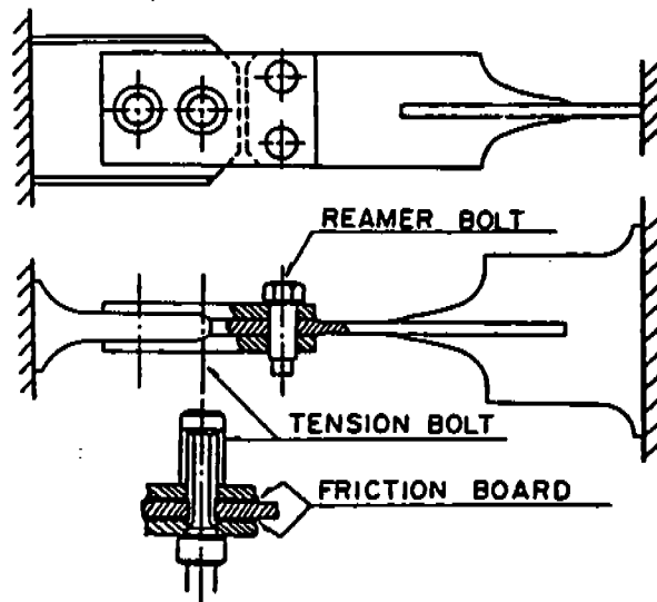
FIGURE 19 - NEW TYPE OF EXCITER (REF. 8)
