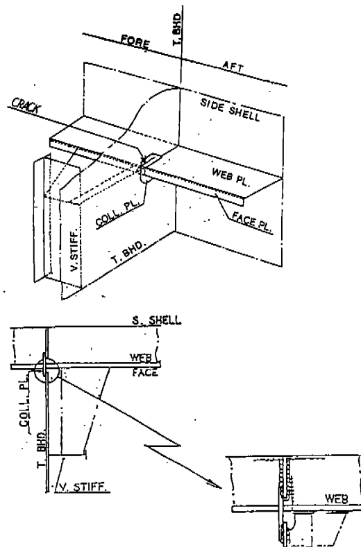
Figure 3.13 - Side Shell Longitudinals Cracks at Transverse Bulkheads
