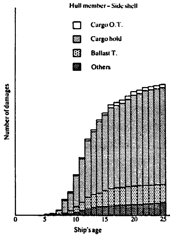
Figure 3.3 - Relation Between Frequency of Damage Due to Corrosion and Fatigue in Side Shell Members, Service Conditions, and Ship Age
