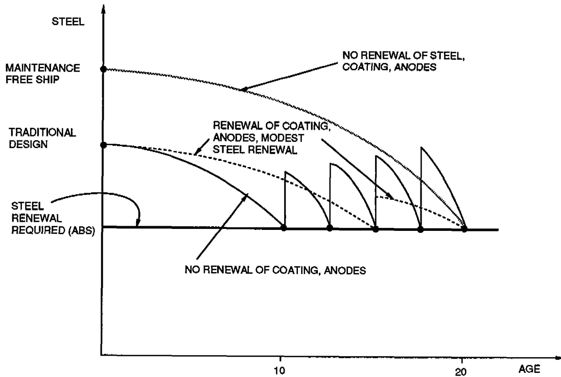
Figure 3.23 - Effective Ship Structure Steel Weight as Function of Design, MSIP Strategy, and Age
