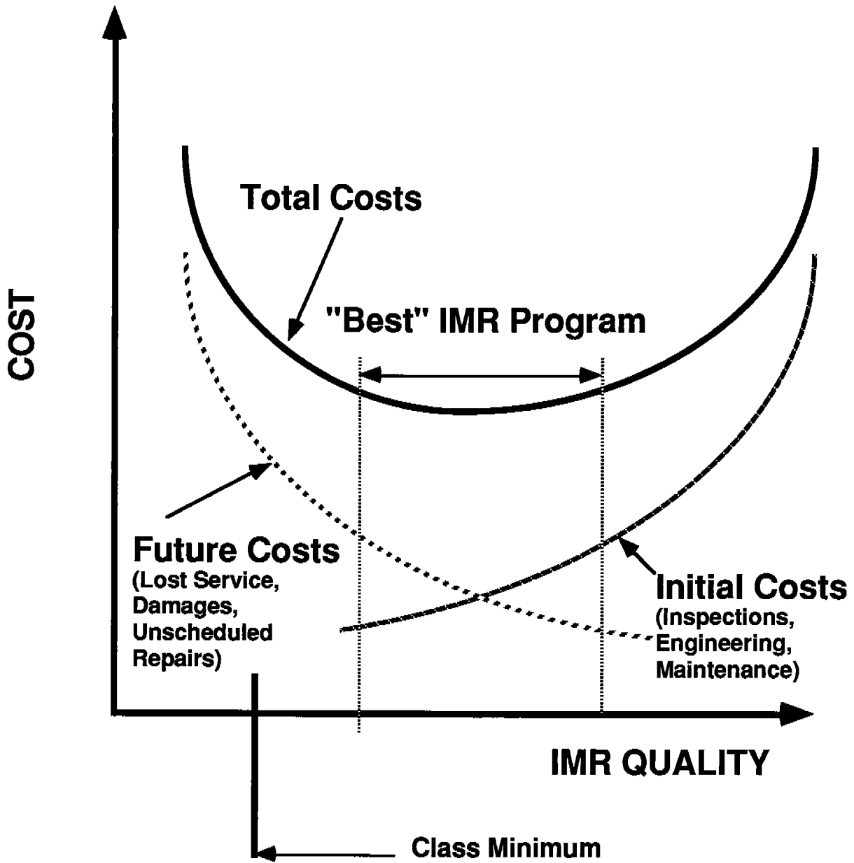
Figure 5.5 - Cost Based Evaluation of Desirable IMR Quality
