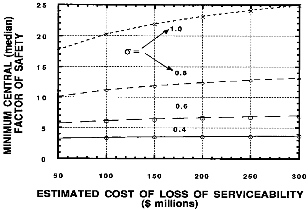
Figure 7.10 - Minimum Central Factor of Safety as a Function of the Estimated Costs Associated With Loss of Serviceability of the Ship Hull Structure
