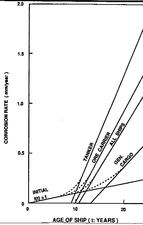
Figure 3.5 - Corrosion Rate as a Function of Ship Age and Type
