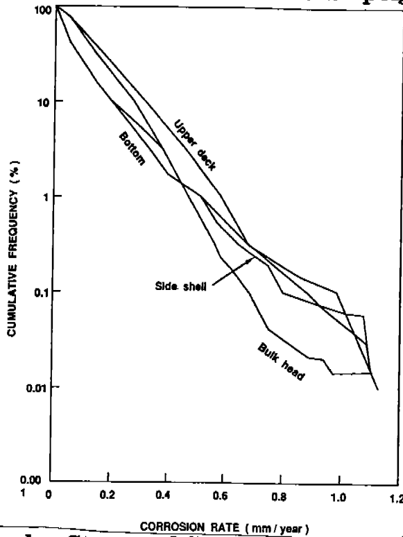
Figure 3.6 - Tanker Structural Components Corrosion Rate Statistics
