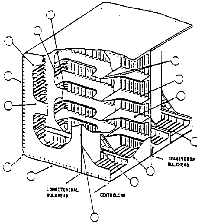
Figure 3.7 - Typical Fatigue Damage Locations in VLCCs
