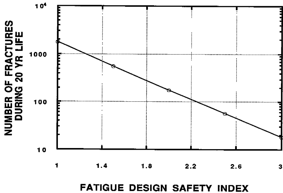
Figure 7.15 - Total Number of Fatigue Fractures Expected in Example ULCC Hull Structure as a Function of the Fatigue Design Safety Index
