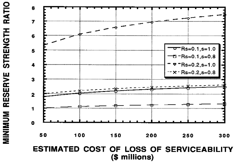
Figure 7.11 - Minimum Reserve Strength Ratio as a Function of the Estimated Costs Associated With Loss of Serviceability of the Ship Hull Structure
