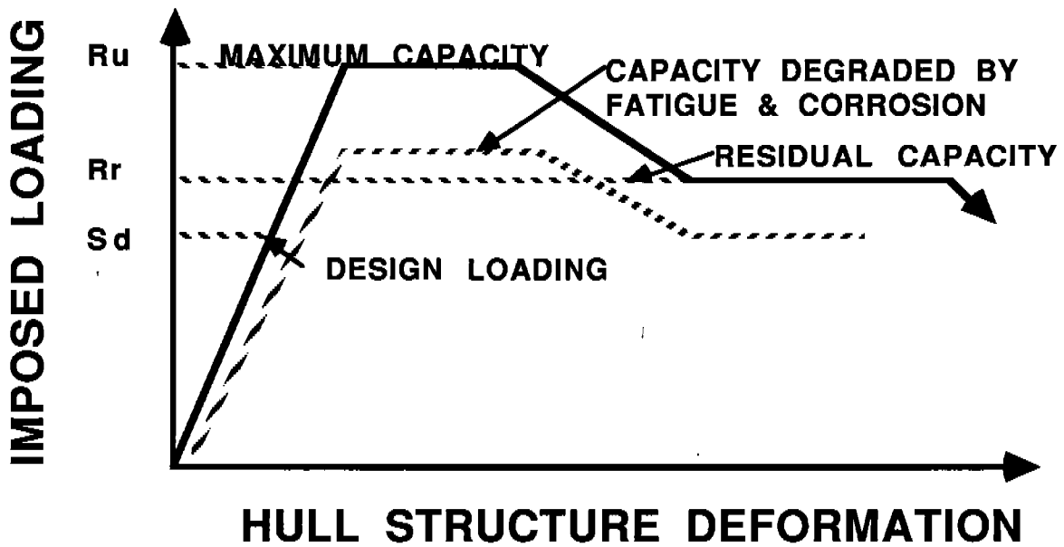
Figure 7.1 - Initial and Degraded Hull Structure Performance Characteristics
