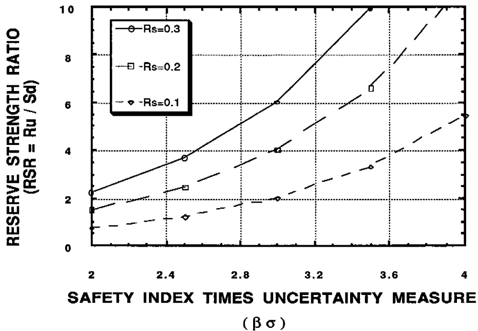
Figure 7.4 - Required Reserve Strength Ratio as a Function of Loading Ratios (median expected maximum loading / design loading)
