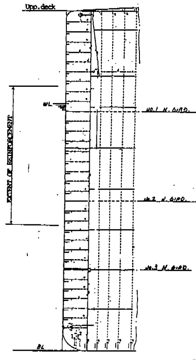
Figure 3.16 - Extent of Reinforcements to Side Shell Longitudinals
