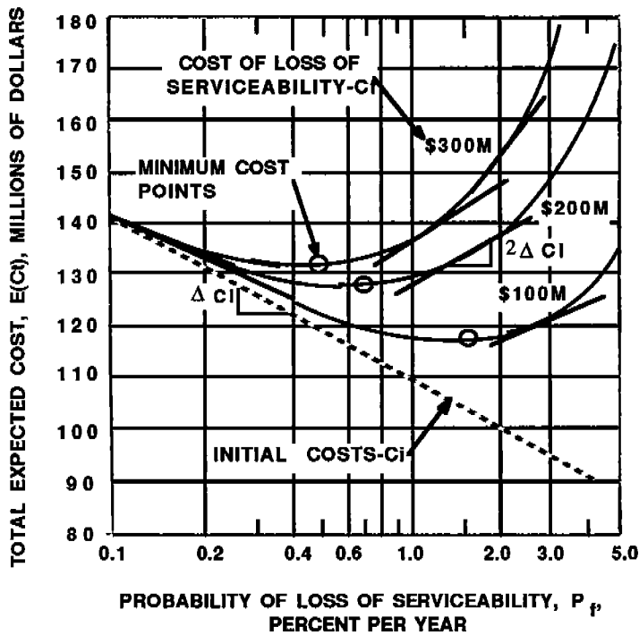
Figure 3.17 - Optimized Utility, Minimum Total Cost Evaluation
