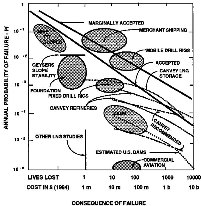
Figure 3.18 - Historic Relationships of Risks and Consequences for Engineered Structures
