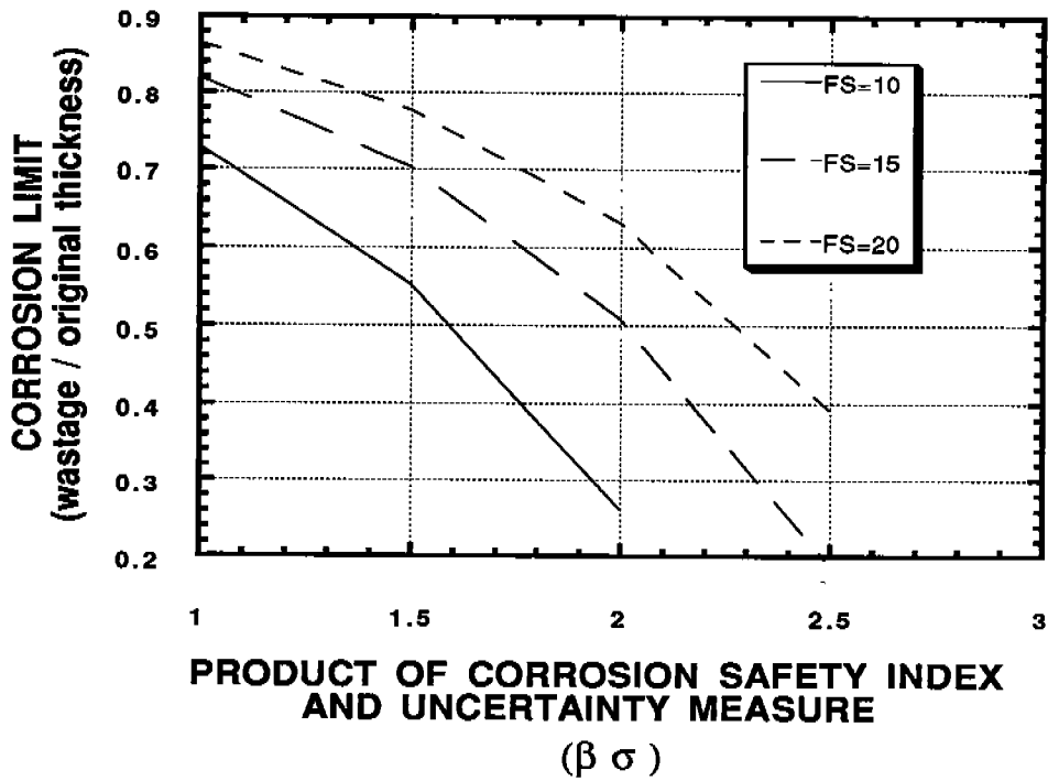
Figure 7.17 - Corrosion Limit as a Function of the Design Corrosion Safety Index and Total Uncertainty Measure (loadings, capacities, corrosion)
