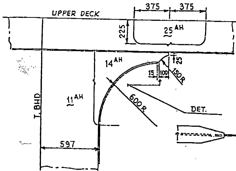
Modified Design EXPECTED FATIGUE LIFE 44.4 YEARS
