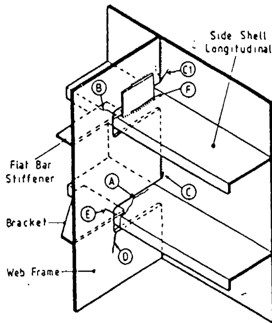
Figure 3.8 - Typical Fatigue Damage to Side Shell Members and Connections
