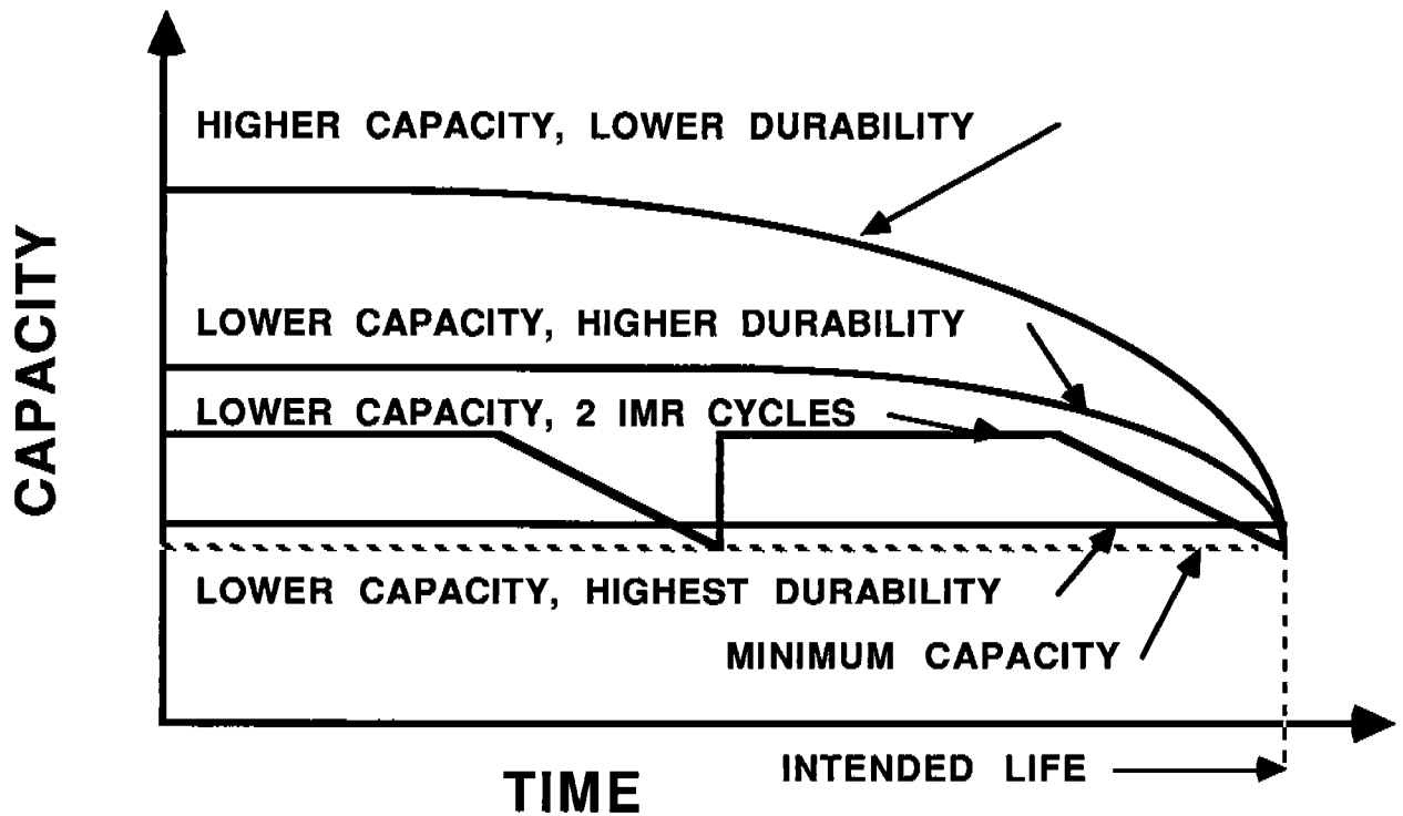
Figure 7.1 - Initial and Degraded Hull Structure Performance Characteristics
