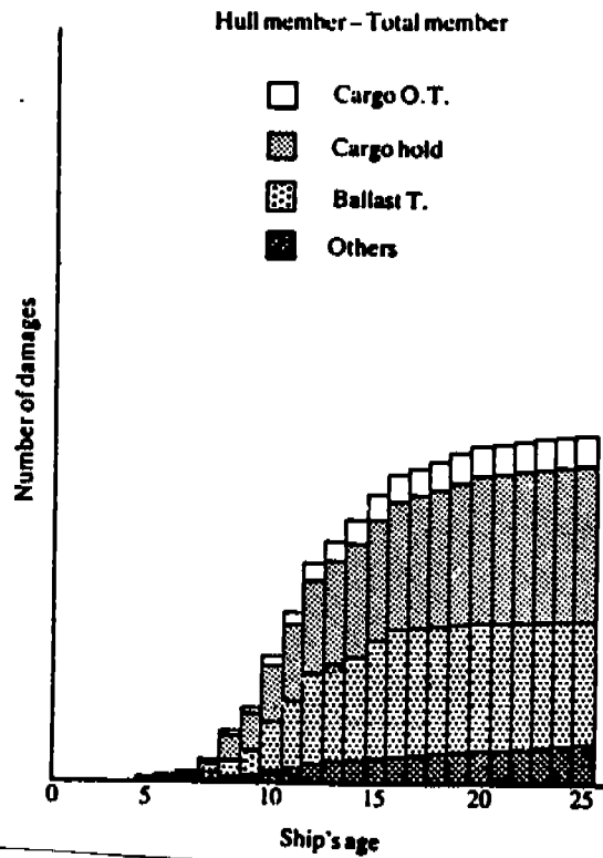
Figure 3.2 - Relation Between Frequency of Damage Due to Corrosion and Fatigue for All Structural Members, Service Conditions, and Ship Age
