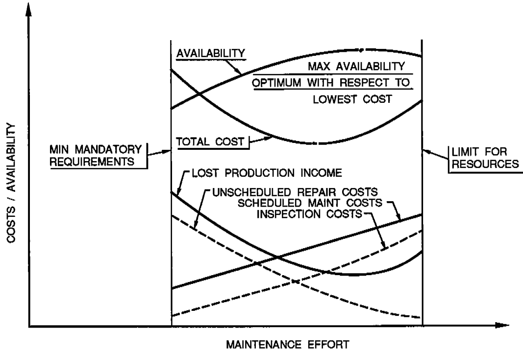
Figure 3.22 - Cost - Benefit Evaluation as a Function of Ship Structure MSIP Effort
