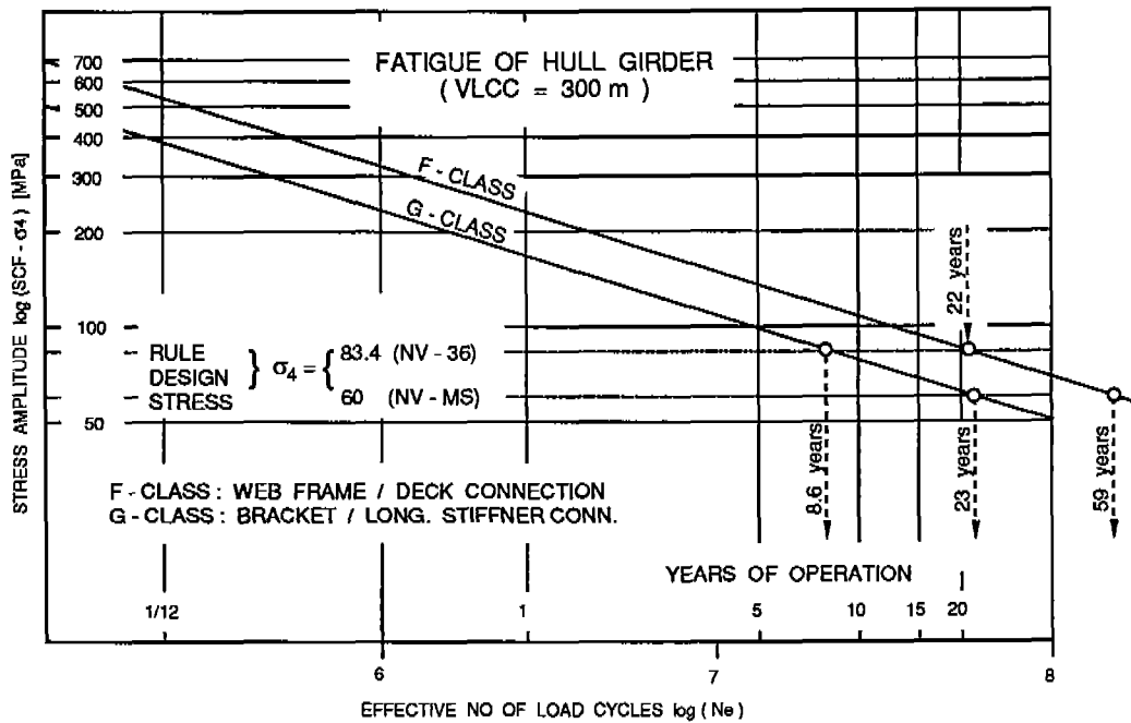
Figure 3.20 - Fatigue of 300 meter VLCC Hull Girder Deck - Bottom Structure Elements in World-Wide Operation
