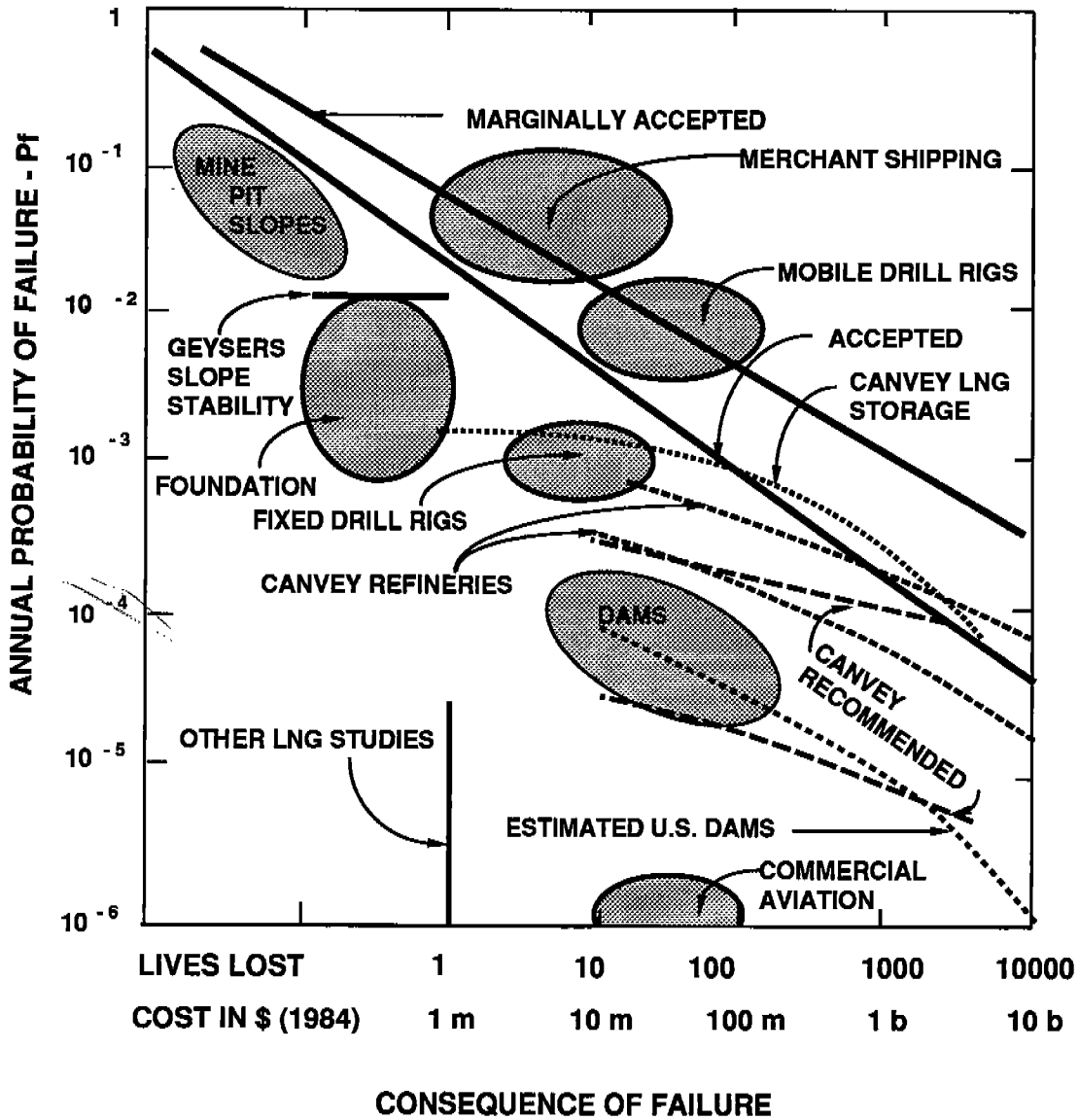
Figure 7.8 - Historic Data on Likelihoods and Consequences of Failures of Engineered Structures
