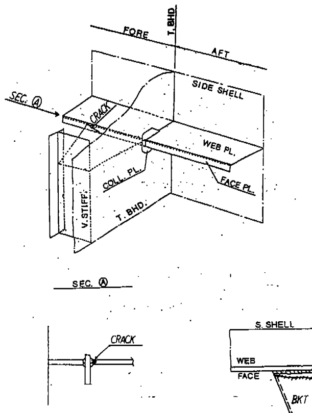
Figure 3.14 - Side Shell Longitudinals Cracks at Transverse Bulkheads
