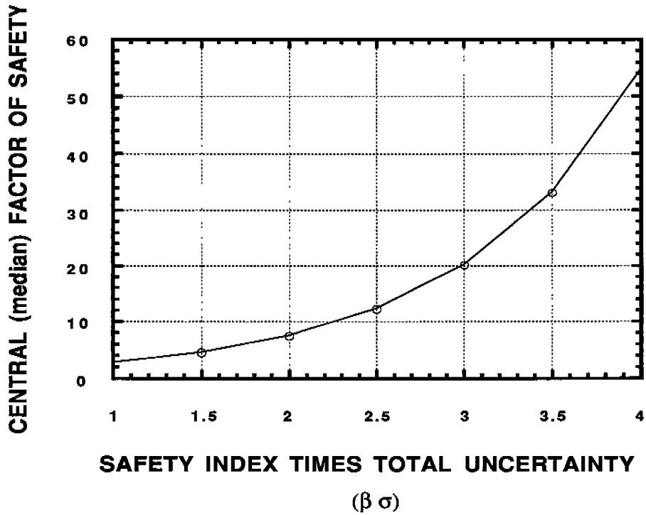
Figure 7.3 - Required Central Factor of Safety as a Function of Required Safety Index and Total Uncertainty in Hull Structure Loadings and Capacities
