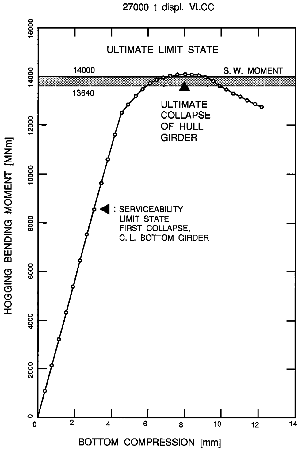
Figure 15 - Tanker Hull Structure Serviceability and Ultimate Limit State Capacities
