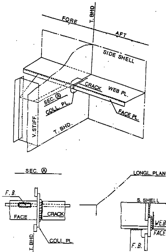
Figure 3.10 - Side Shell Longitudinals Cracks at Transverse Bulkheads
