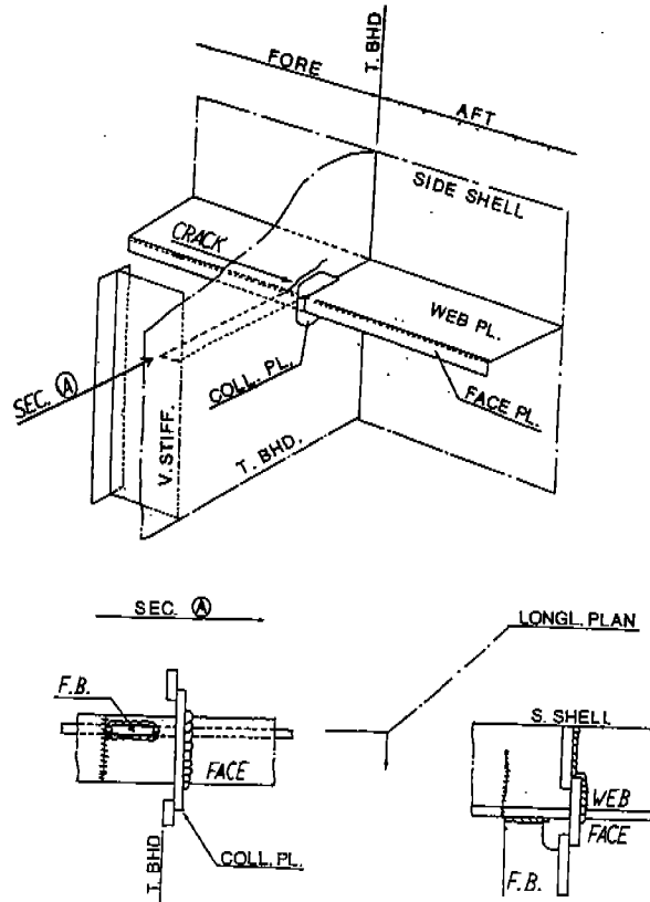
Figure 3.9 - Side Shell Longitudinals Cracks at Transverse Bulkheads
