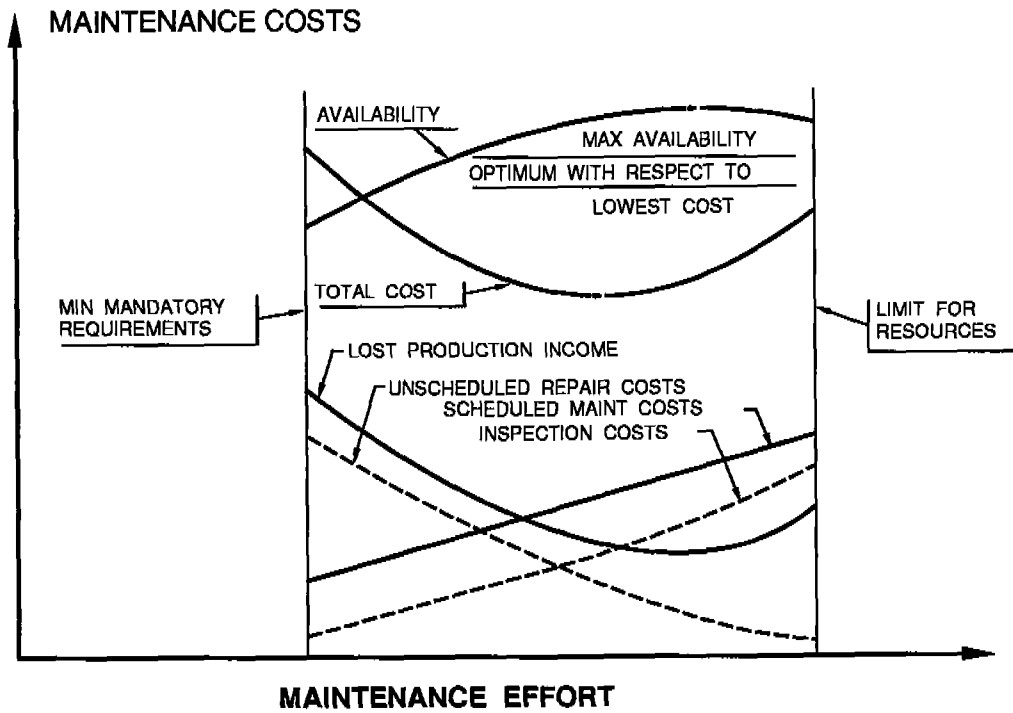
Figure 7.6 - Hull Structure Maintenance Cost - Benefit Evaluation
