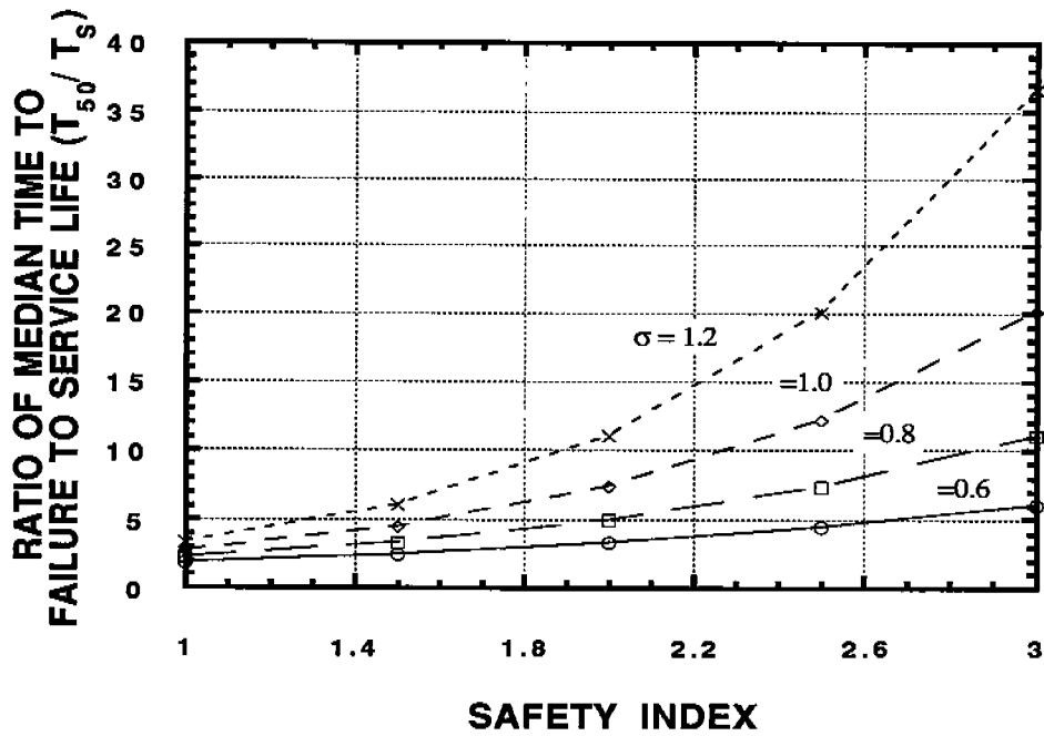
Figure 7.13 - Required Fatigue Design Factor of Safety as a Function of the Fatigue Design Safety Index and Total Uncertainties in Time to Failure
