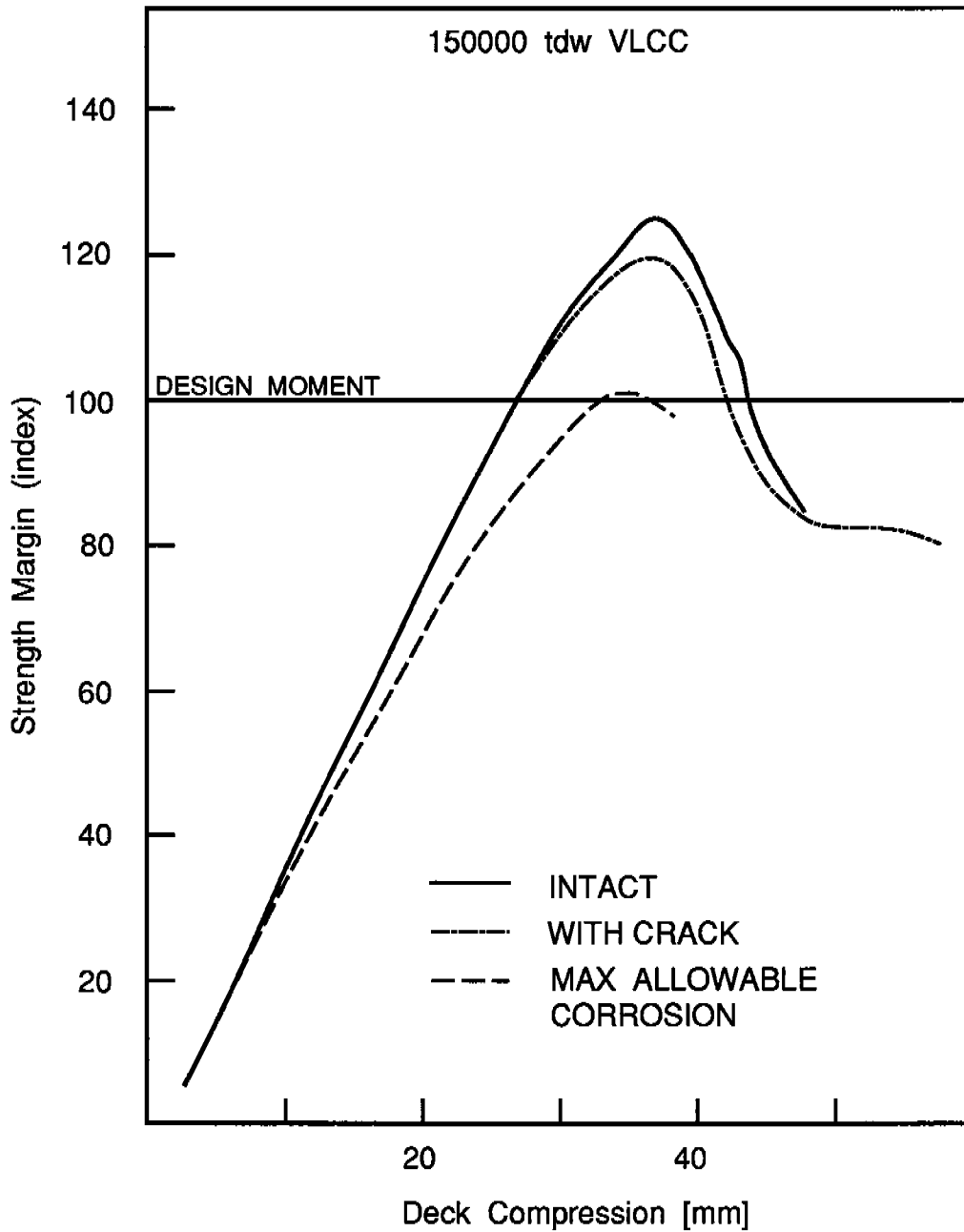
Figure 3.21 - Effects of Fatigue Cracking and Corrosion on the Longitudinal Bending Capacity of a 150,000 DWT VLCC
