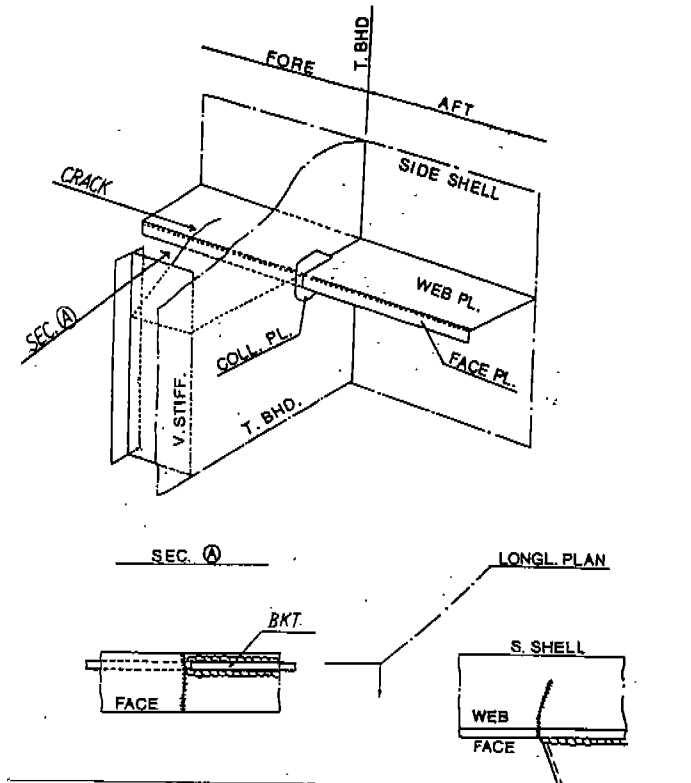
Figure 3.11 - Side Shell Longitudinals Cracks at Transverse Bulkheads
