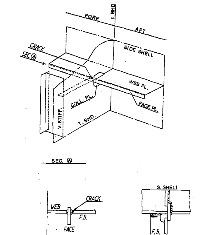
Figure 3.12 - Side Shell Longitudinals Cracks at Transverse Bulkheads
