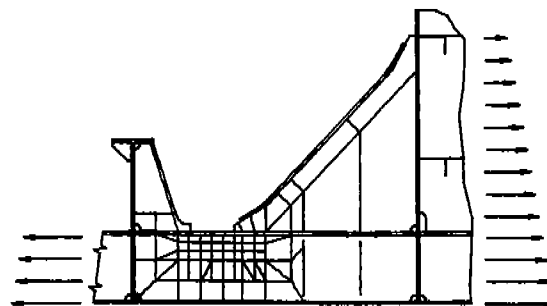
Detail Stresses using Finite Element Model
