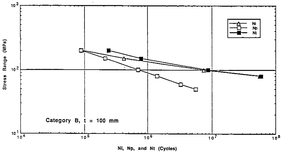
Fig. B-5 Predicted N_I , N_p and N_T for Category B A36 steel weldments. Thickness = 100mm, K_{fmax} = 3.0 .
