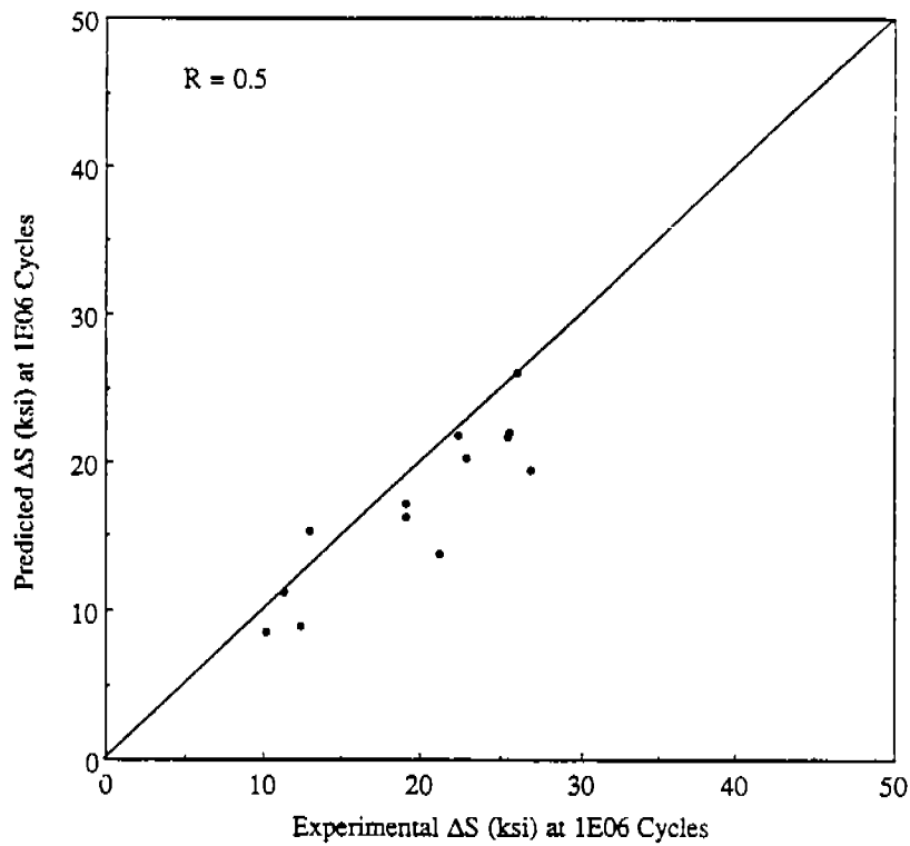
Fig. A-7 Predicted and estimated mean fatigue strength at 10 6 cycles for R=0.5
