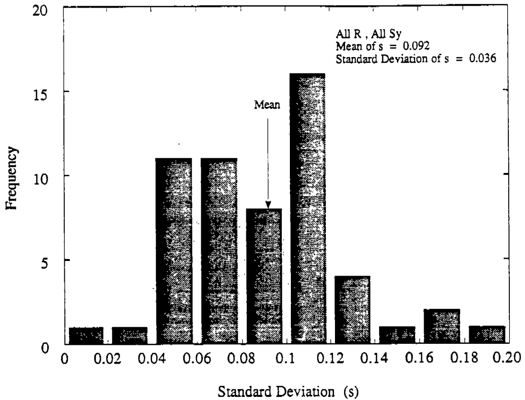
Fig. A-1 Histogram of standard deviations on the log of fatigue strength for all R ratios and all values of base metal yield strength
