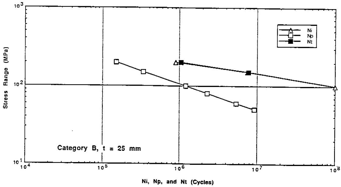
Fig. B-4 Predicted N_I , N_p and N_T for Category B A36 steel weldments. Thickness = 25mm, K_{fmax} = 2.0 .
