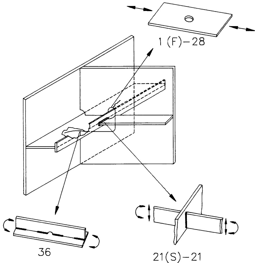
FIGURE 5-1: FATIGUE IN WEB FRAME BRACKET
