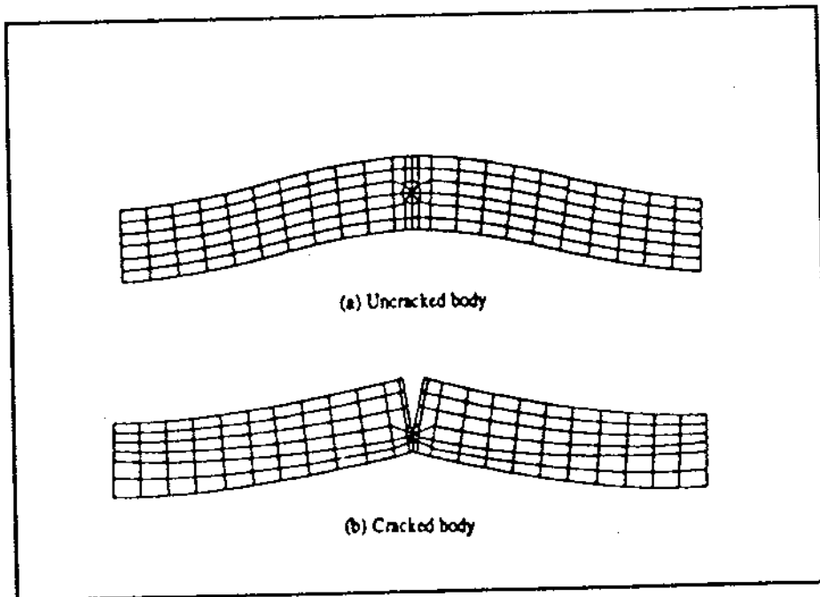
Fig 4.8 Deformed Shapes of the Plate with Fixed Ends Subjected to Bending
