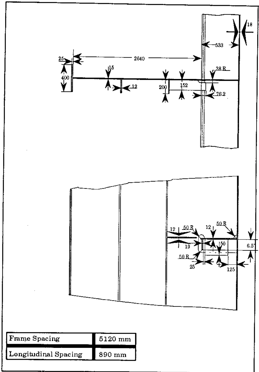
Fig 6.4 Configuration for Detail in Sideshell 32- 36.
