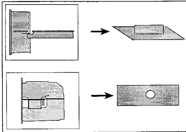
Fig 6.9 Proposed CSD and Corresponding Specimens
