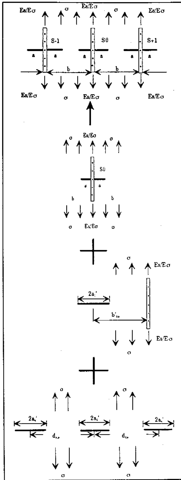
Fig 1 Ancillary configuration for collinear cracks in a periodically stiffened panel
