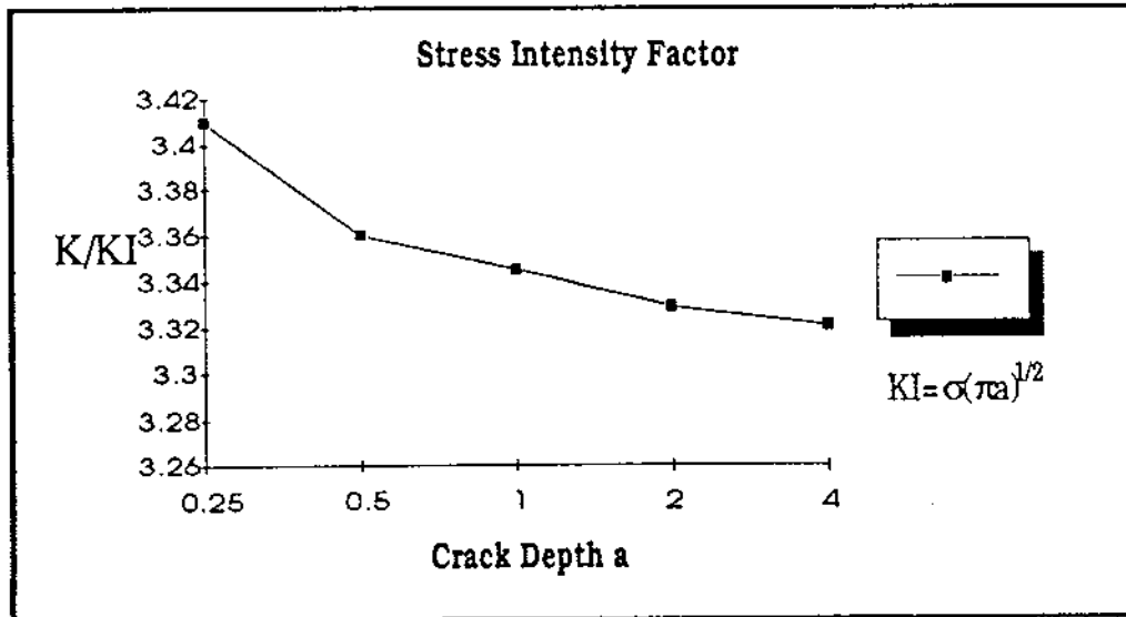
Fig. 6.12 Stress Intensity Factor for Specimen A
