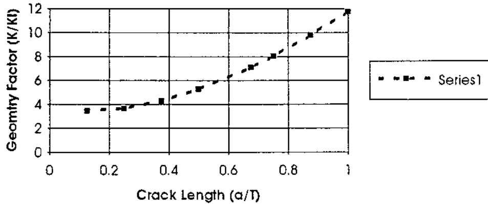
Fig 6.15 Stress Intensity Factor for Specimen B
