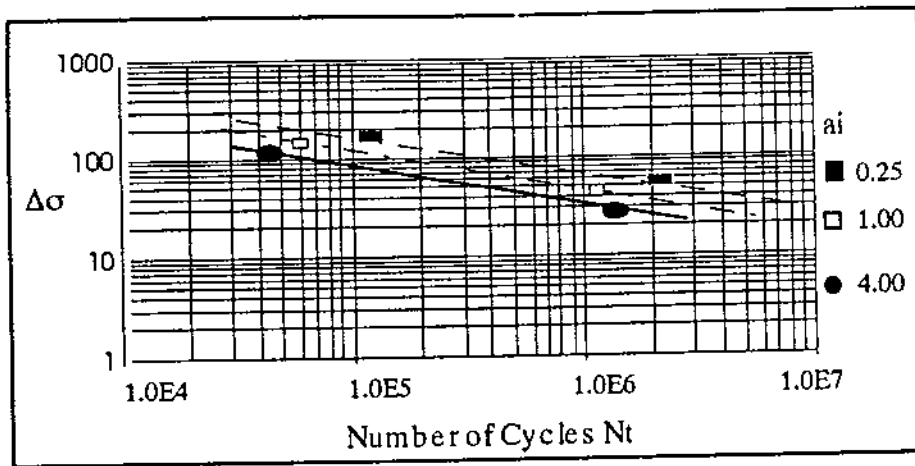
Fig 4.15 Equivalent S-N curves for non load carrying joint with initial crack length a_i = 0.25\text{mm}, 1\text{mm}, 4\text{mm}
