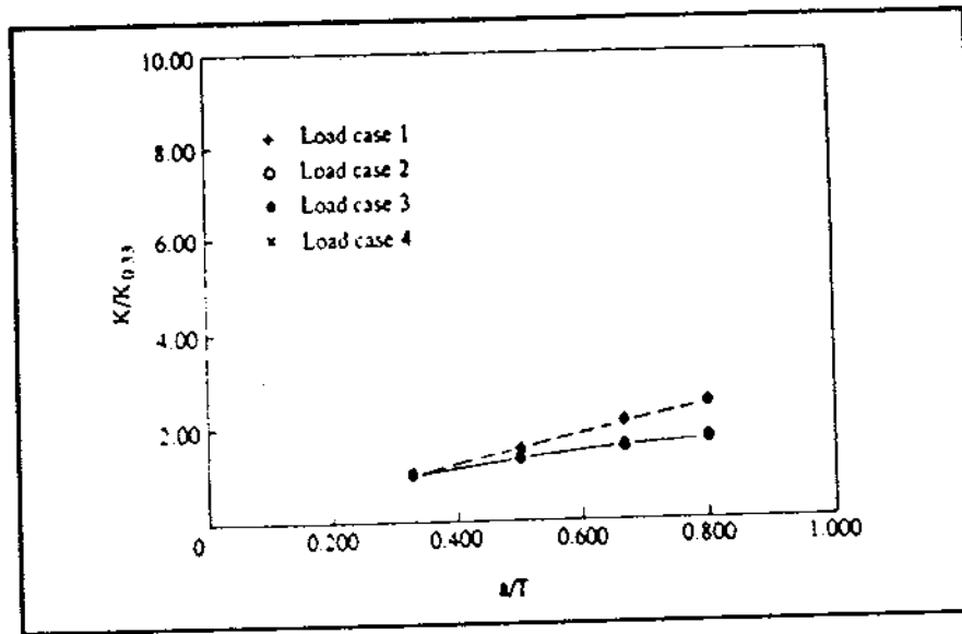
Fig 4.5 Variation of SIFs for the Edge Cracked Plate, Configuration (3)
