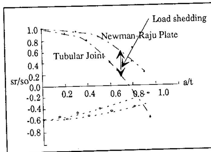
Fig 1.4 Load Shedding Study in Offshore Tubular Joints.
