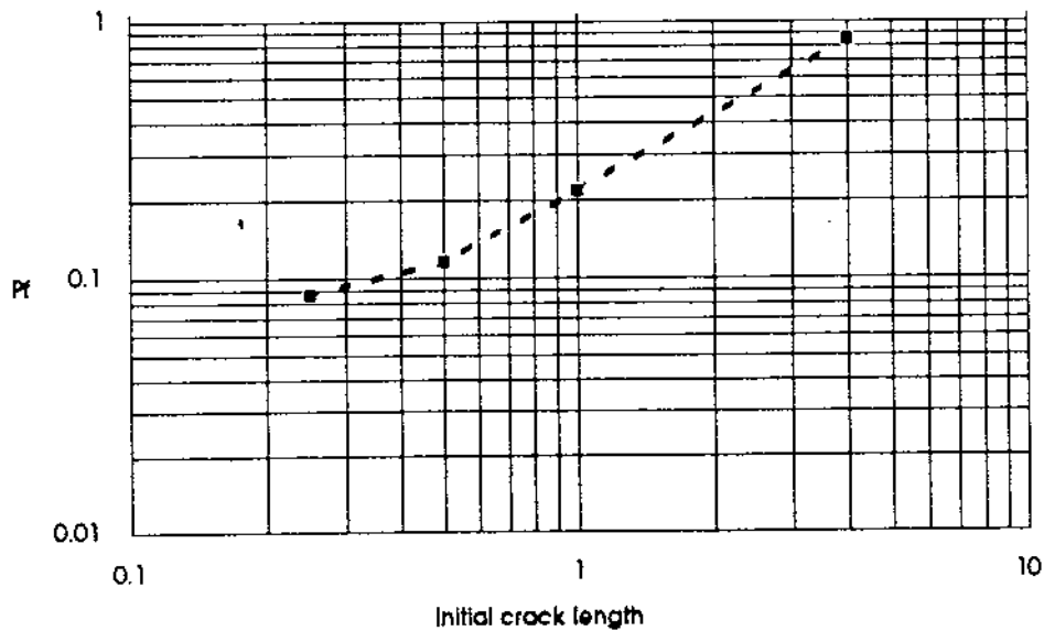
Fig 7.6 Probability of Failure during the Remaining 10 Years Service Life in Fitness for Purpose Analysis. (Load Shedding is not included)
