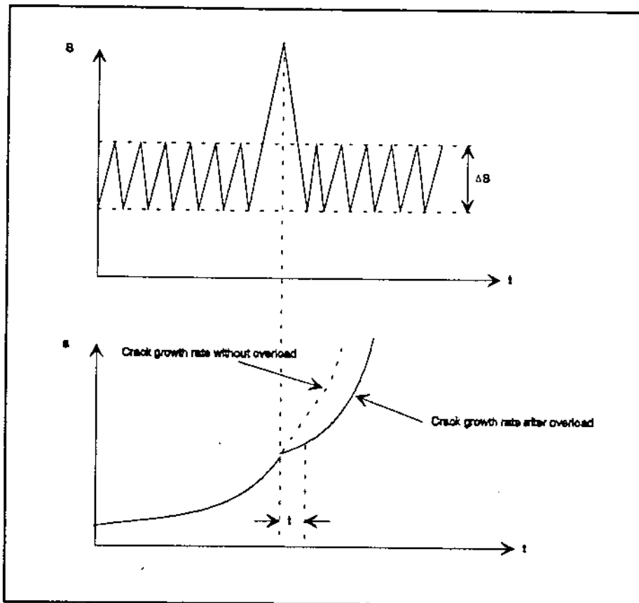
Fig. 5.1 Load Sequence during the Crack Propagation
