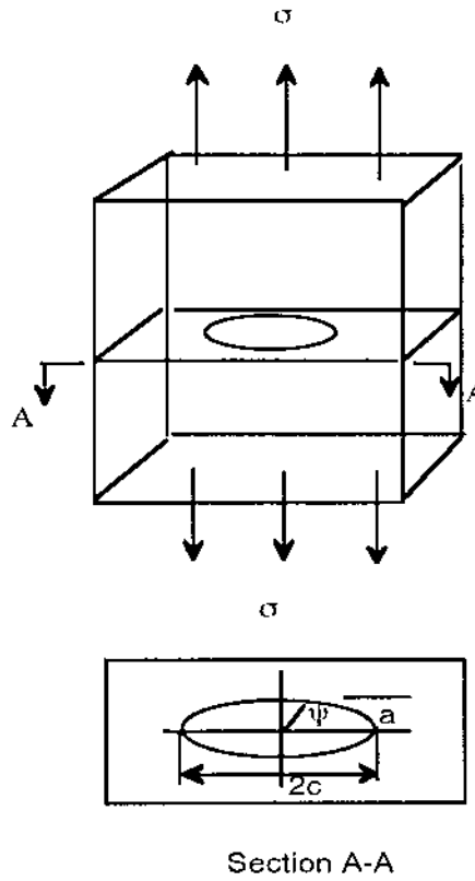
Fig. 2.2 Three-dimensional standard case : Embedded elliptical crack in an infinite solid subjected to uniform tension.
