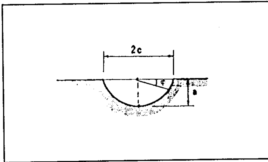
Fig. 3.5 Crack Front as Given by the Angle \phi
