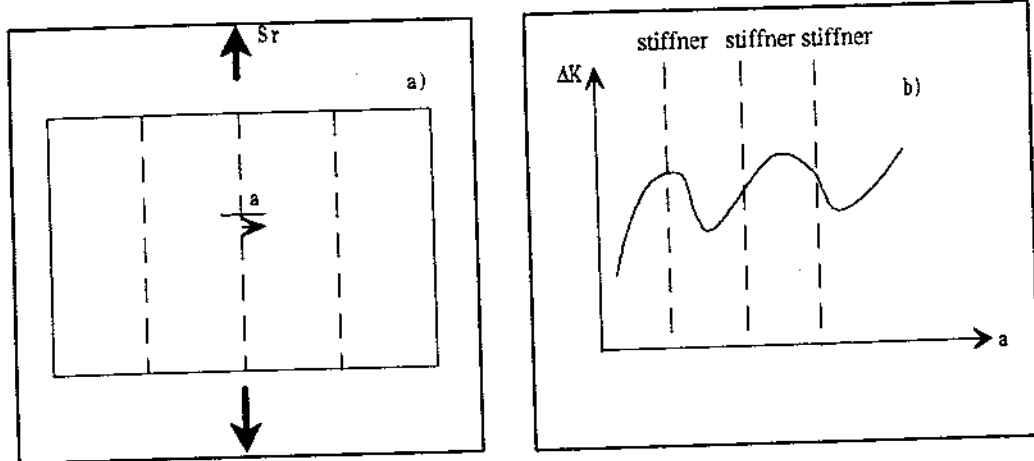
Fig 1.8 Fatigue Loaded Stiffened Plate
