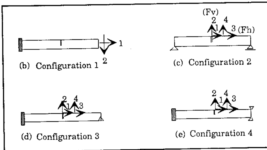
Fig 4.2 Edge Crack Plate under Four Different Load Cases
