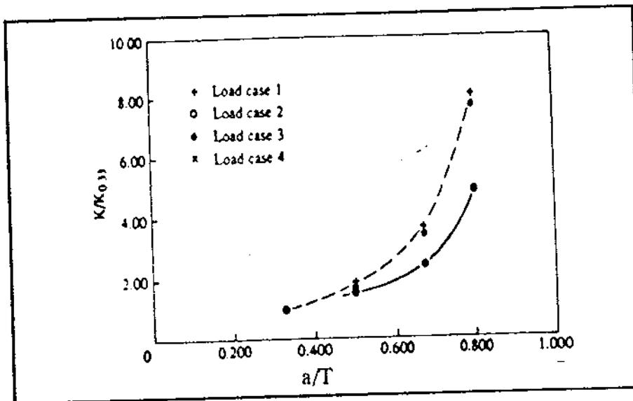
Fig 4.3 Variation of SIFs for the Edge Cracked Plate, Configuration (1)
