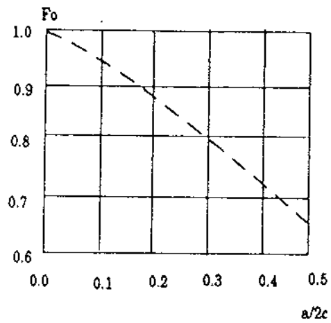
Fig. 2.6 The basic (elliptic) shape correction factor
