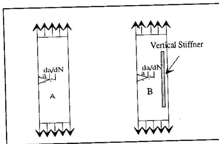
Fig 1.3 Description of Load shedding due to adjacent structures
