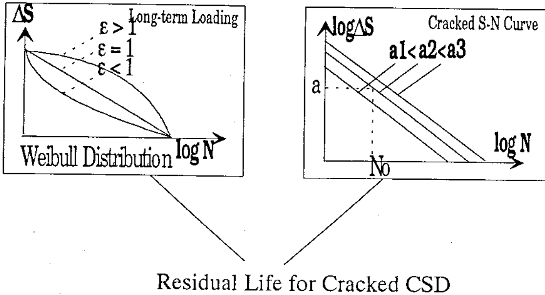
Fig 6.1 Remaining Life Estimation based on Fitness for Purpose Evaluation.
