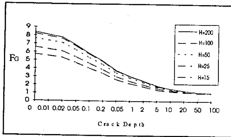
Fig 6.5 Stress Gradient Factor Vs Gusset Height for Plate with Welded on Gusset Plate
