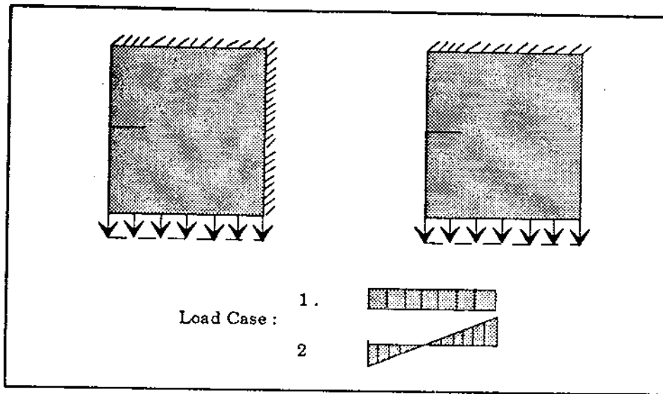
Fig 2.5 Boundary conditions and load cases for proposed cracked plate
