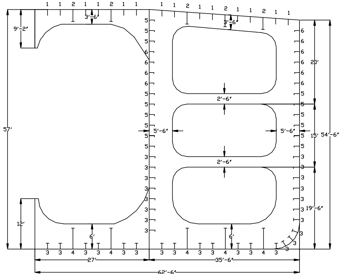
Figure 4-22. Schematic Diagram of Tanker Vessel Showing Cross-Sectional Dimensions (Feet and Inches) and Stiffeners Type Codes
