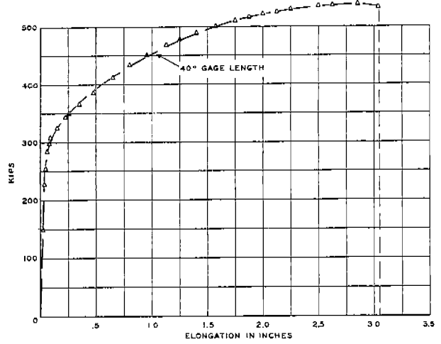
FIG. XXVI-B LOAD-ELONGATION DIAGRAM TYPE ZB SPECIMEN DN-ZB-H14 -20°F
