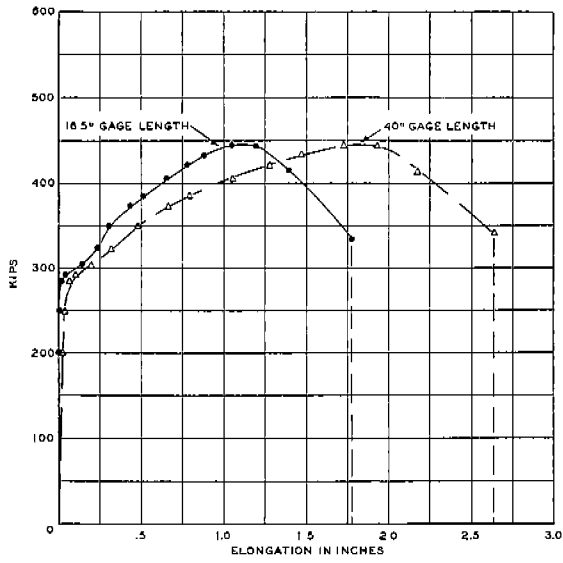
LEGEND SPECIMEN SIZE: 13\frac{1}{2}'' \times 40'' \times \frac{3}{4}'' FIG. IX-B LOAD-ELONGATION DIAGRAM TYPE YW3 SPECIMEN DN-YW3-H12 50°F
