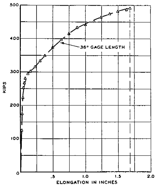
FIG. XLV-B LOAD-ELONGATION DIAGRAM TYPE ZC2 SPECIMEN ABS-B-ZC2-II6 -20°F 0% SHEAR
