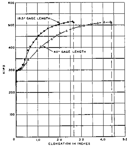
LEGEND SPECIMEN SIZE: 1\frac{1}{2}'' \times 40'' \times \frac{3}{4}'' FIG. V-B LOAD-ELONGATION DIAGRAM TYPE YW1 SPECIMEN DN-YW1-G4 0°F
