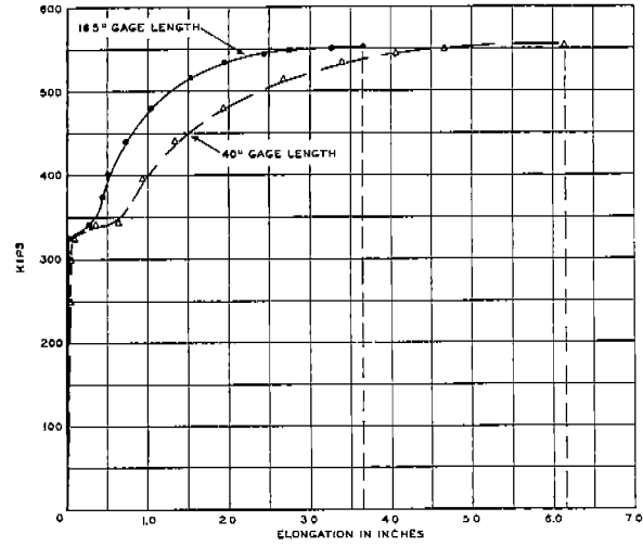
LEGEND: SPECIMEN SIZE: 1\frac{1}{2}'' \times 40'' \times \frac{3}{4}'' FIG. VI-B LOAD-ELONGATION DIAGRAM TYPE YW1 SPECIMEN DN-YW1-F10 -35°F
