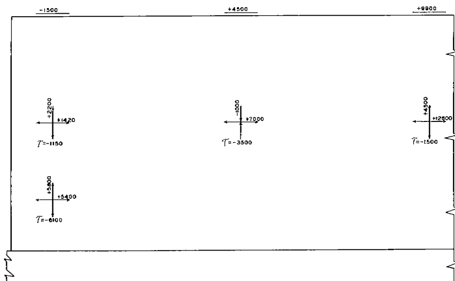
FIG. 31 STRESS COMPONENTS AT 150 KIPS SPECIMEN DN-Z3-H6
