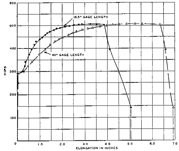
LEGEND: SPECIMEN SIZE: 13\frac{1}{2}'' \times 40'' \times \frac{3}{4}'' FIG. II-B LOAD-ELONGATION DIAGRAM TYPE YWI SPECIMEN DN-YWI-G5 30°F
