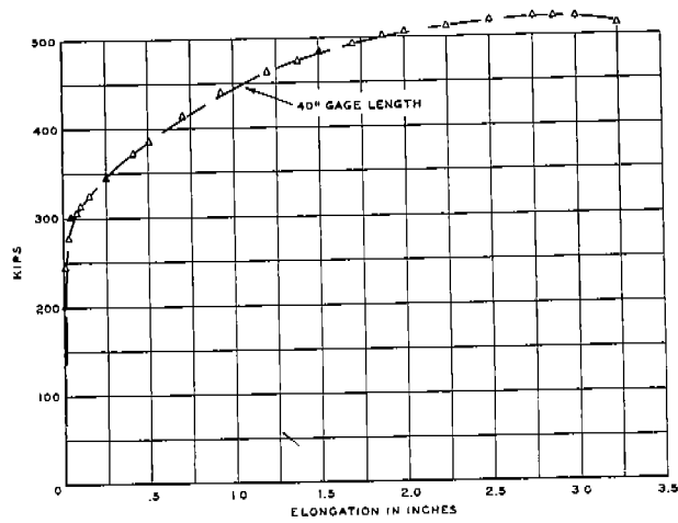
FIG. XXXIX-B LOAD-ELONGATION DIAGRAM TYPE ZC2 SPECIMEN DN-ZC2-H8 0°F
