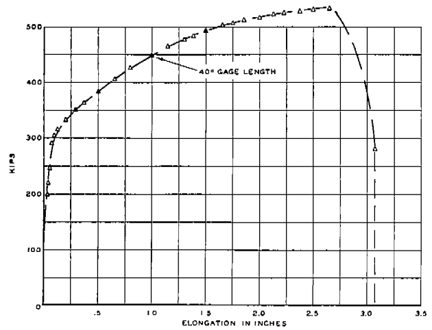
FIG. XL-B LOAD-ELONGATION DIAGRAM TYPE ZC2 SPECIMEN DN-ZC2-H15 -20°F
