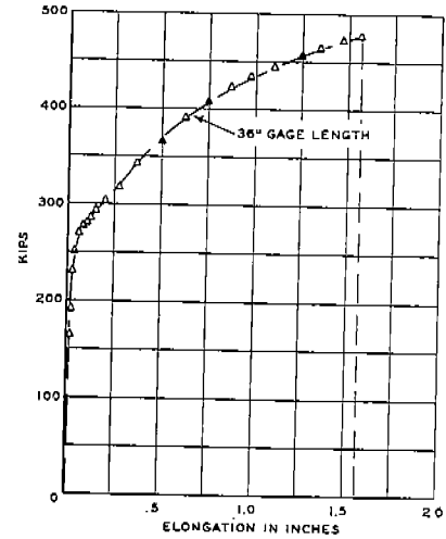
FIG. LVI-B LOAD-ELONGATION DIAGRAM TYPE ZE SPECIMEN ABS-B-ZE-II3 -20°F 0% SHEAR
