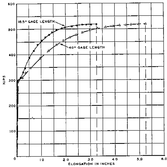
LEGEND: SPECIMEN SIZE: 13\frac{1}{2}'' \times 40'' \times \frac{3}{4}'' FIG. III-B LOAD-ELONGATION DIAGRAM TYPE YWI SPECIMEN DN-YWI-G7 20°F
