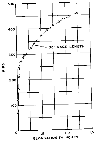
FIG. XLIX - B LOAD-ELONGATION DIAGRAM TYPE ZD SPECIMEN ABS-B-ZD-I8 0°F 0% SHEAR
