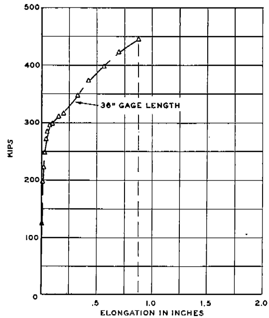
FIG. XXIV-B LOAD-ELONGATION DIAGRAM TYPE Z3 SPECIMEN ABS-B-Z3-I3 -40°F 0% SHEAR
