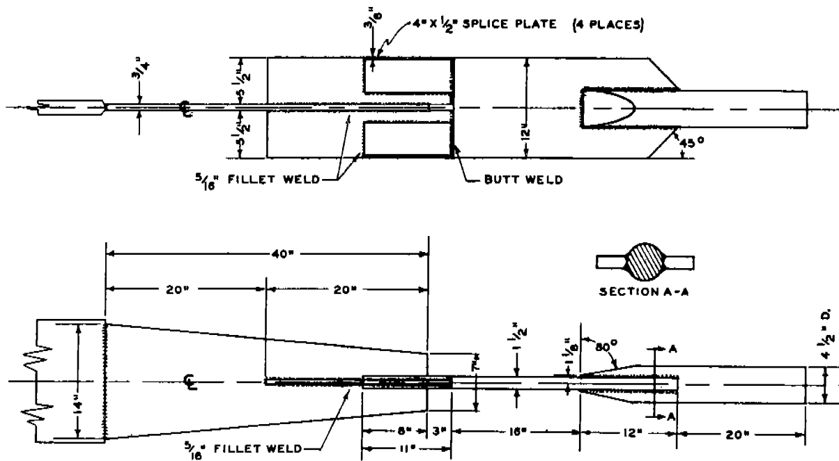
FIG. 2 TYPE DN-Z3 SPECIMEN ARRANGEMENT
