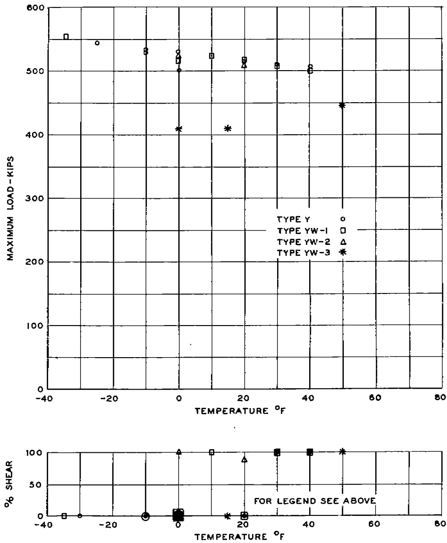
FIG.16A SUMMARY - MAXIMUM LOAD AND PERCENT SHEAR VS. TEMPERATURE TYPE Y SPECIMENS
