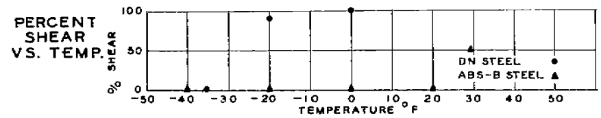
FIG. 36 SUMMARY TYPE ZC2 SPECIMENS
