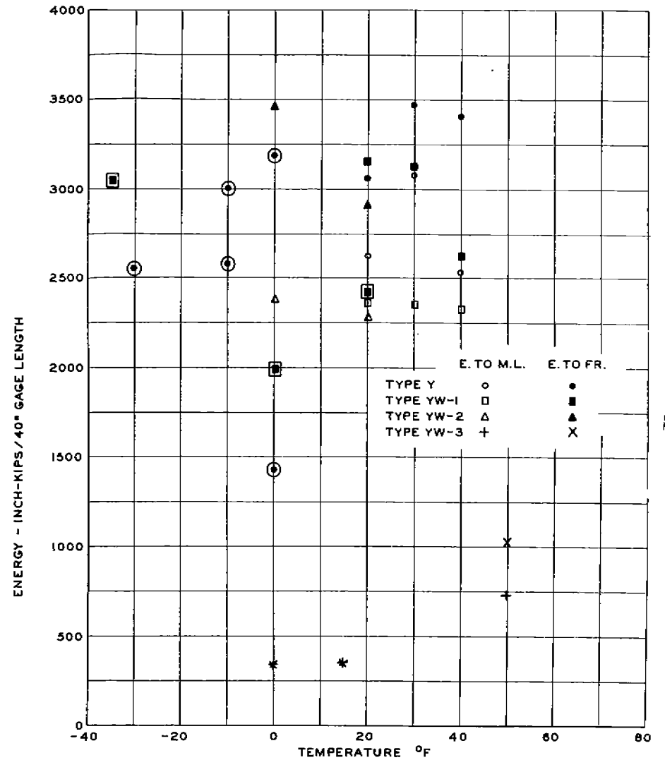
FIG.16B SUMMARY - ENERGIES TO MAXIMUM LOAD AND FRACTURE VS. TEMPERATURE TYPE Y SPECIMENS
