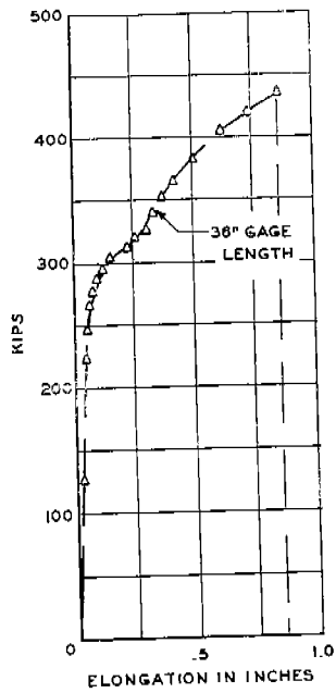
FIG. XXI-B LOAD-ELONGATION DIAGRAM TYPE Z3 SPECIMEN ABS-B-Z3-J15 -15°F 0% SHEAR
