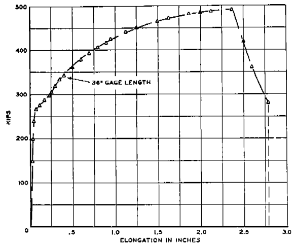
FIG. XLII-B LOAD-ELONGATION DIAGRAM TYPE ZC2 SPECIMEN ABS-B-ZC2-J6 29°F 50% SHEAR
