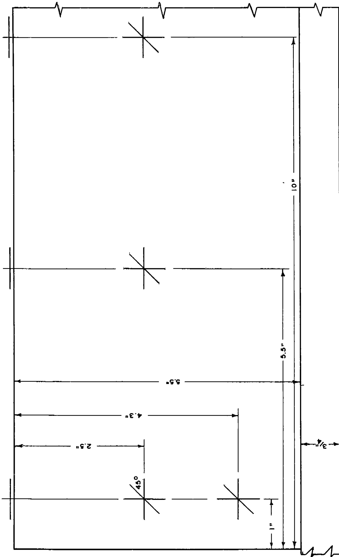
FIG. 15 STRAIN GAGE LOCATIONS - SPECIMEN DN - Z3 - H6
