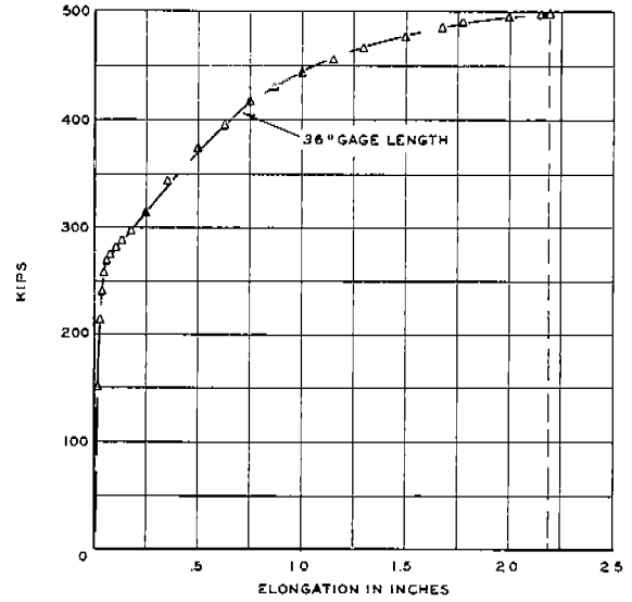
FIG. XVIII-B LOAD-ELONGATION DIAGRAM TYPE Z3 SPECIMEN ABS-B-Z3-I2 20°F 0% SHEAR
