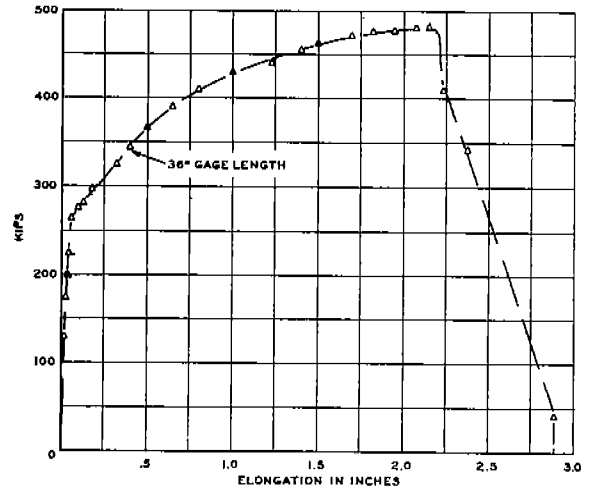
FIG. XVI-B LOAD-ELONGATION DIAGRAM TYPE Z3 SPECIMEN ABS-B-Z3-I5 50°F 100% SHEAR
