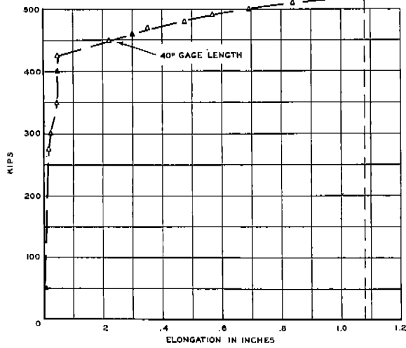
FIG. XV-B LOAD-ELONGATION DIAGRAM TYPE Z3 SPECIMEN DN-Z3-H5 -40°F
