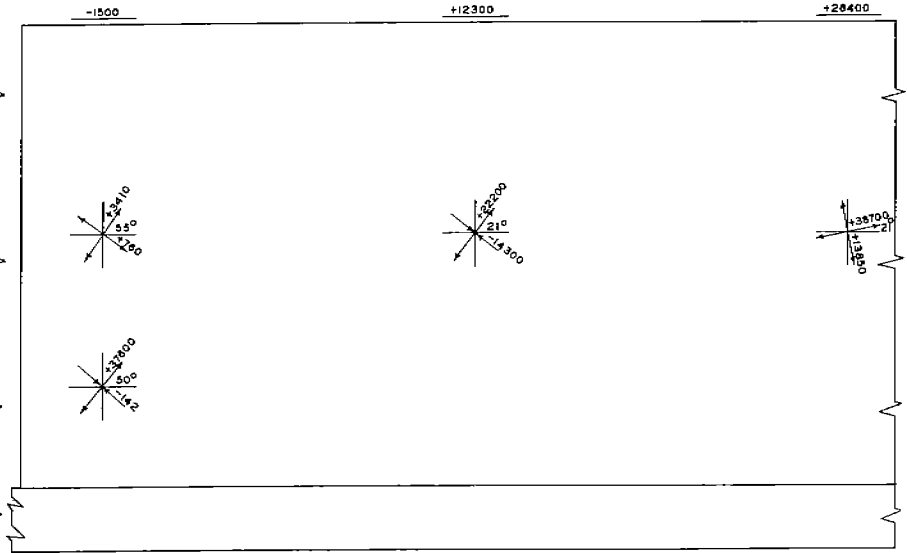
FIG. 30 PRINCIPAL STRESSES AT 350 KIPS SPECIMEN DN-Z3-H6
