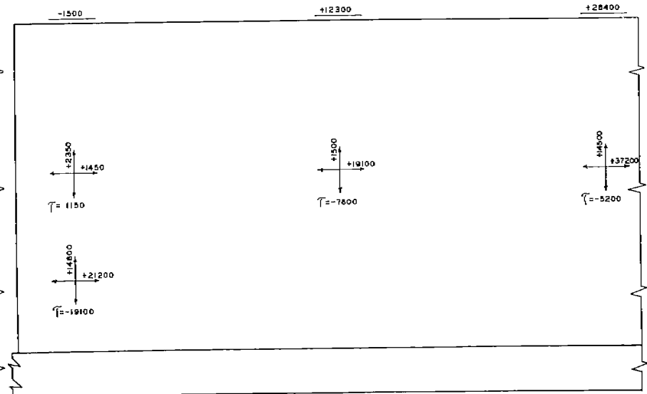
FIG. 32 STRESS COMPONENTS AT 350 KIPS SPECIMEN DN-Z3-H6
