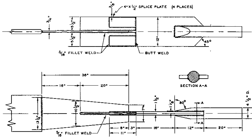
FIG. 3 TYPE ABS-B-Z3 SPECIMEN ARRANGEMENT
