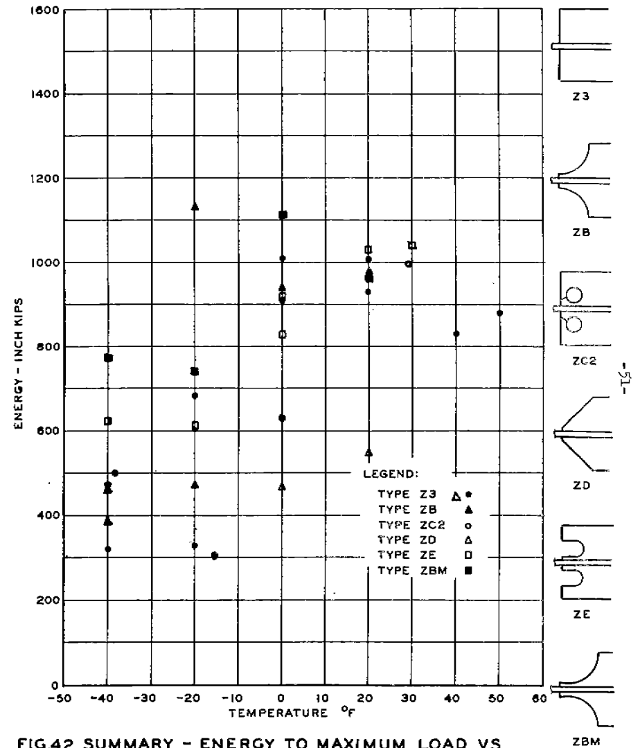
FIG.42 SUMMARY - ENERGY TO MAXIMUM LOAD VS. TEMPERATURE TYPE Z SPECIMENS - ABS-B STEEL GAGE LENGTH 36"
