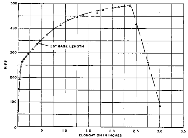
FIG. XXVIII-B LOAD-ELONGATION DIAGRAM TYPE ZB SPECIMEN ABS-B-ZB-II2 20°F 100% SHEAR
