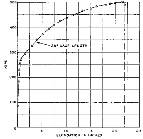
FIG. LIV-B LOAD ELONGATION DIAGRAM TYPE ZE SPECIMEN ABS-B-ZE-III 0°F 5% SHEAR
