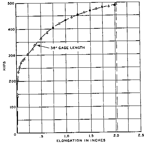
FIG. LV-B LOAD-ELONGATION DIAGRAM TYPE ZE SPECIMEN ABS-B-ZE-II8 0°F 0% SHEAR
