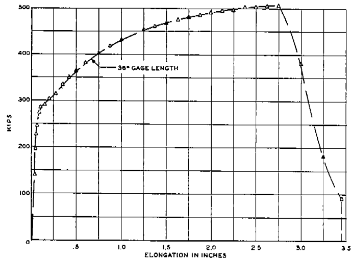
FIG. XXXII-B LOAD-ELONGATION DIAGRAM TYPE ZBM SPECIMEN ABS-B-ZBM-116 30°F 90% SHEAR
