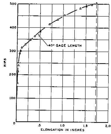
FIG. XXXVIII-B LOAD-ELONGATION DIAGRAM TYPE ZC1 SPECIMEN DN-ZC1-H10 -20°F
