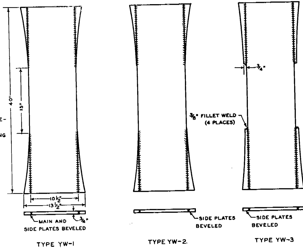
FIG. 1 SPECIMENS WITH LONGITUDINAL WELDMENT
