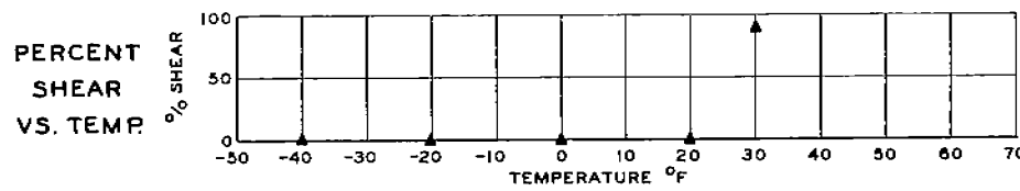
FIG. 35 SUMMARY TYPE ZBM SPECIMENS ABS-B STEEL
