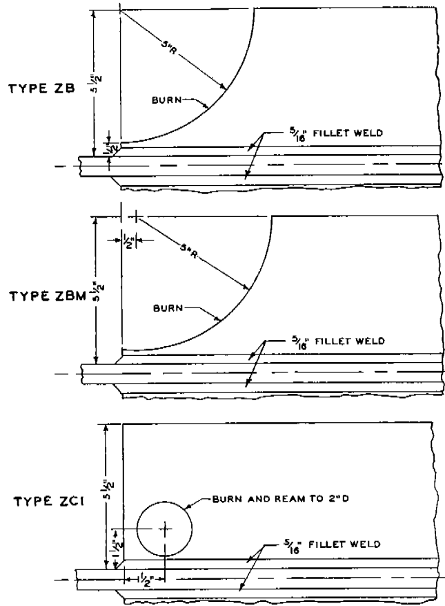
FIG. 4 END DETAIL VARIATIONS FOR TYPE "Z" SPECIMENS
