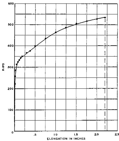
FIG. XL1-B LOAD-ELONGATION DIAGRAM TYPE ZC2 SPECIMEN DN-ZC2-H11 -35°F 0% SHEAR
