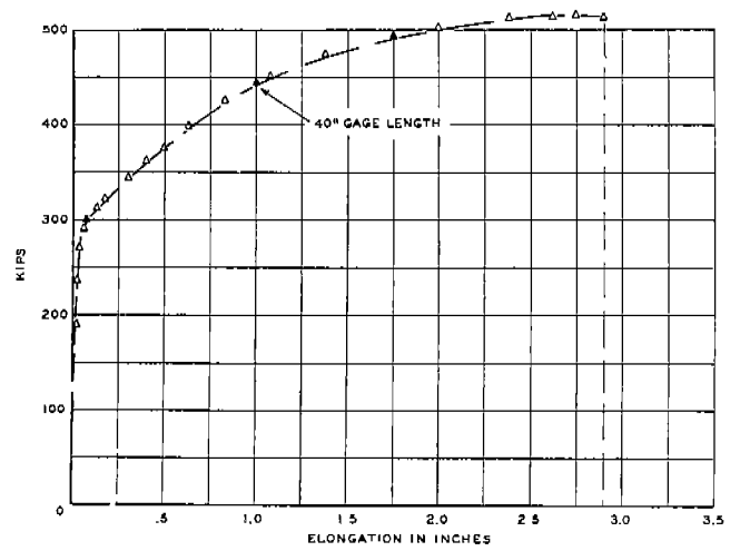
FIG. XII-B LOAD-ELONGATION DIAGRAM TYPE Z3 SPECIMEN DN-Z3-H8 40°F
