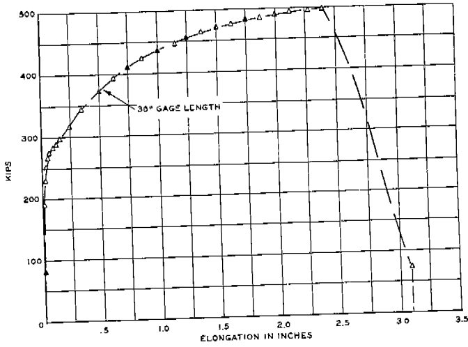
FIG. LVIII-B LOAD-ELONGATION DIAGRAM TYPE ZE SPECIMEN ABS-B-ZE-II0 20°F 100% SHEAR
