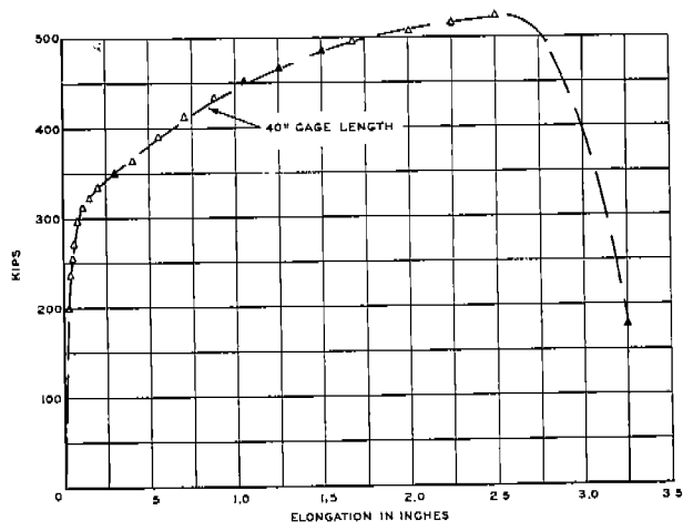
FIG. XXXVII-B LOAD-ELONGATION DIAGRAM TYPE ZC1 SPECIMEN DN-ZC1-H7 0°F
