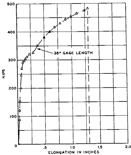
FIG. XXIII-B LOAD-ELONGATION DIAGRAM TYPE Z3 SPECIMEN ABS-B-Z3-J3 -38°F 0% SHEAR
