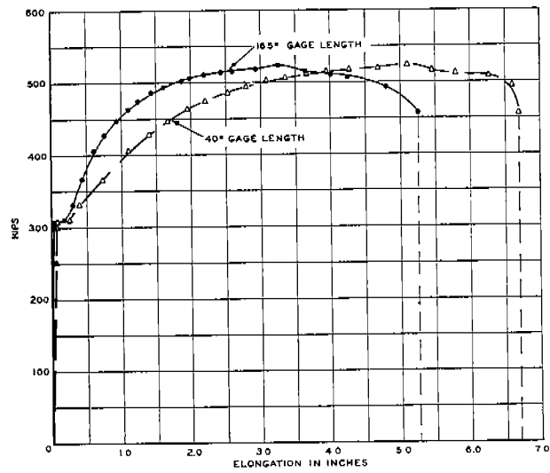
LEGEND: SPECIMEN SIZE: 13\frac{1}{2}'' \times 40'' \times \frac{3}{4}'' FIG. IV-B LOAD-ELONGATION DIAGRAM TYPE YWI SPECIMEN DN-YWI-G8 15°F
