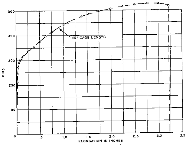
FIG. XXV-B LOAD-ELONGATION DIAGRAM TYPE ZB SPECIMEN DN-ZB-H9 0°F
