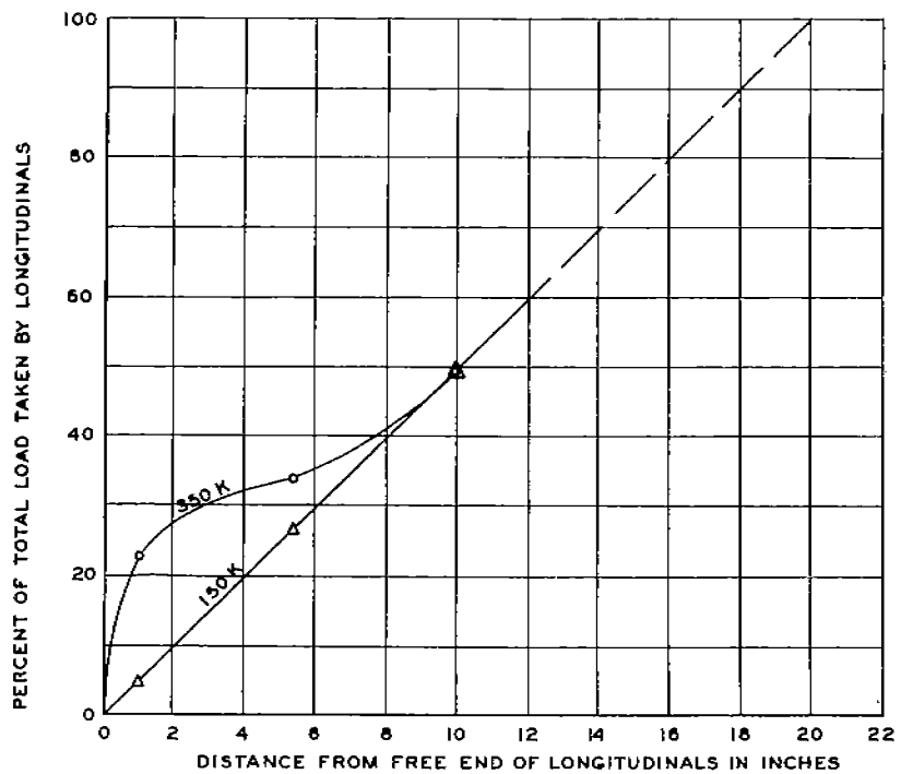
FIG. 33 UNLOADING CHARACTERISTICS OF LONGITUDINALS SPECIMEN DN-Z3-H6
