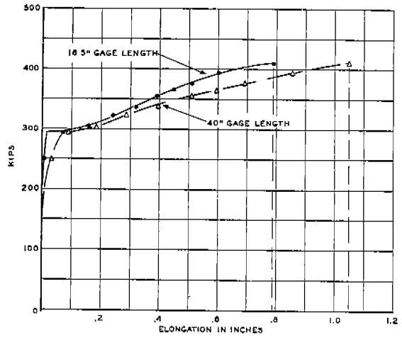
FIG. X-B LOAD-ELONGATION DIAGRAM TYPE YW3 SPECIMEN DN-YW3-H4 15°F
