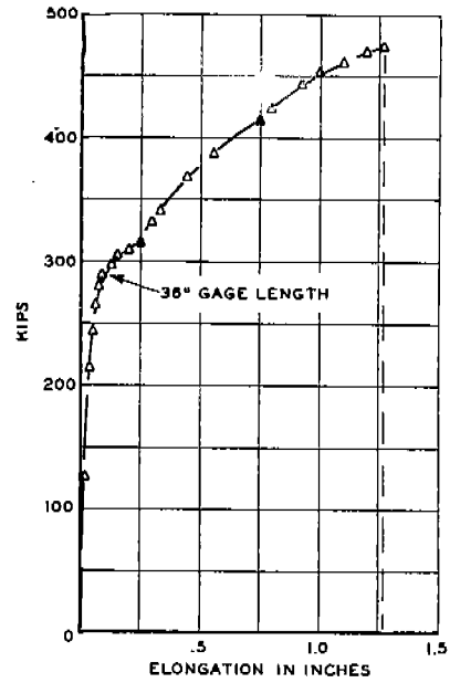
FIG. XLVI-B LOAD-ELONGATION DIAGRAM TYPE ZC2 SPECIMEN ABS-B-ZC2-J5 -40°F 0% SHEAR
