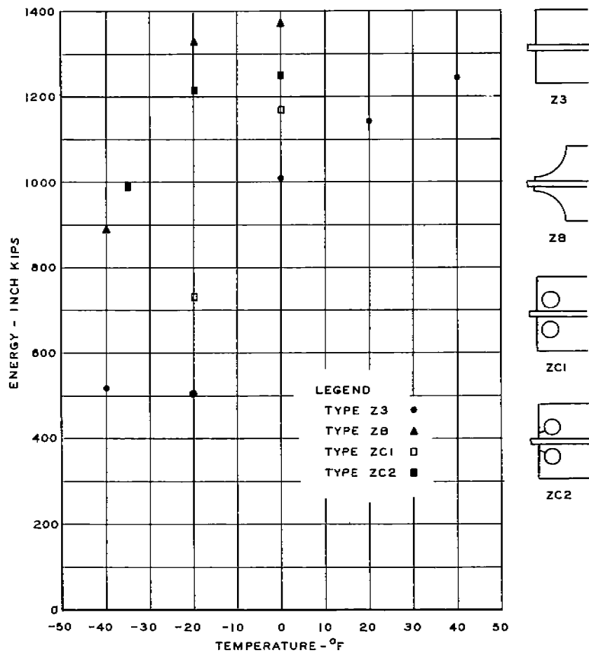
FIG.41 SUMMARY - ENERGY TO MAXIMUM LOAD VS. TEMPERATURE TYPE Z SPECIMENS - DN STEEL GAGE LENGTH 40"
