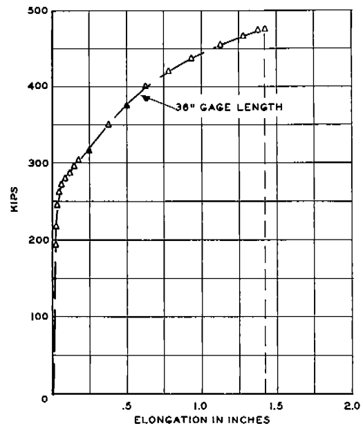
FIG. XLVIII-B LOAD-ELONGATION DIAGRAM TYPE ZD SPECIMEN ABS-B-ZD-I9 20°F 0% SHEAR
