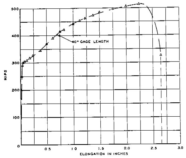
FIG. XIV-B LOAD-ELONGATION DIAGRAM TYPE Z3 SPECIMEN DN-Z3-G13 0°F
