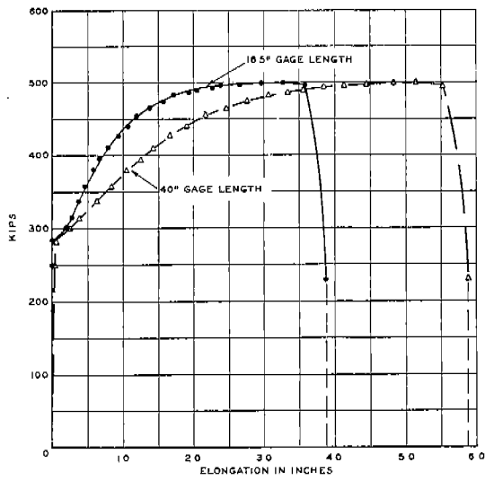
LEGEND: SPECIMEN SIZE: 13\frac{1}{2}'' \times 40'' \times \frac{3}{4}'' FIG. I-B LOAD-ELONGATION DIAGRAM TYPE YWI SPECIMEN DN-YWI-G6 40°F
