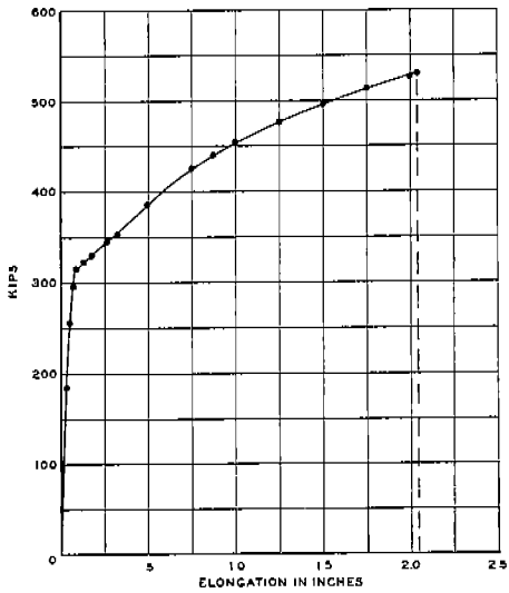
FIG. XXVII-B LOAD-ELONGATION DIAGRAM TYPE ZB SPECIMEN DN-ZB-H13 -40°F 0% SHEAR
