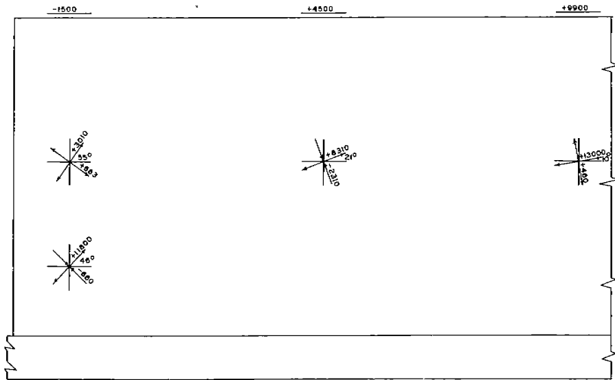
FIG. 29 PRINCIPAL STRESSES AT 150 KIPS SPECIMEN DN-Z3-H6
