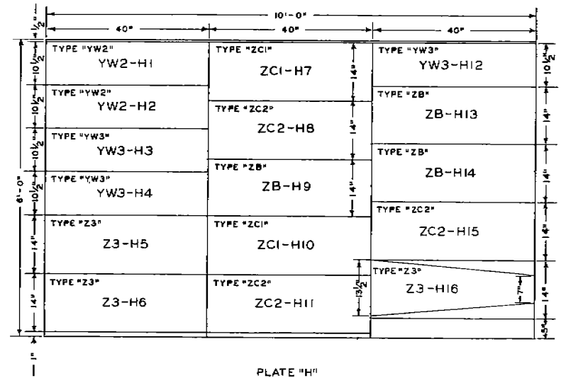
FIG. 10 3/4" DN PLATE LAYOUT
