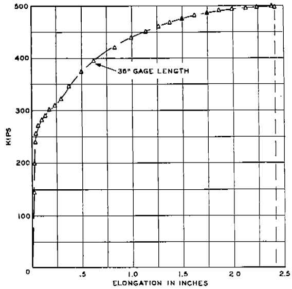
FIG. LII - B LOAD-ELONGATION DIAGRAM TYPE ZE SPECIMEN ABS-B-ZE-J8 30°F 5% SHEAR
