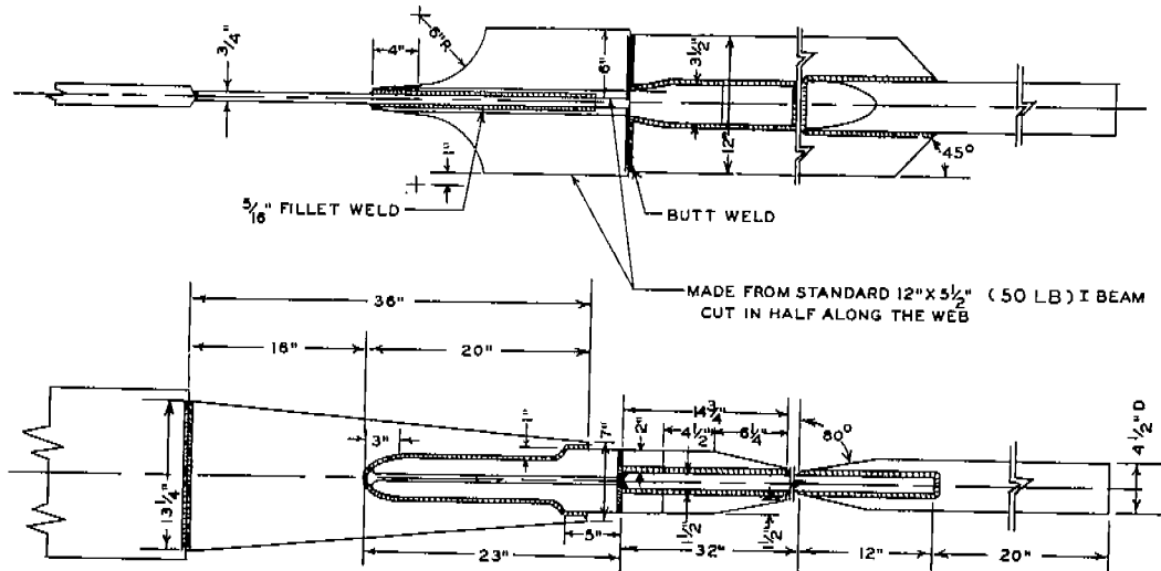
FIG. 6 TYPE ABS-B-ZT2 SPECIMEN ARRANGEMENT
