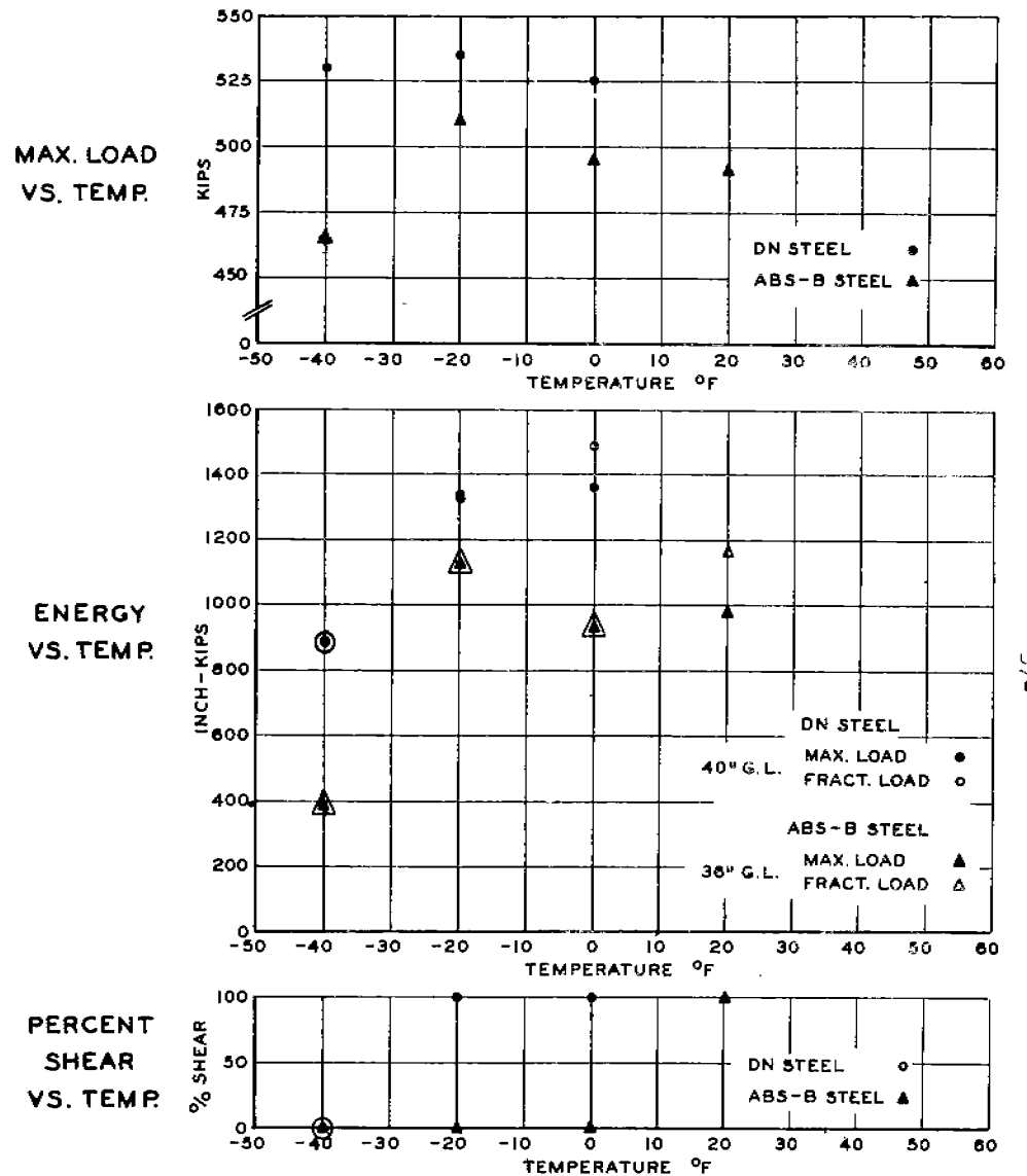
FIG. 34 SUMMARY TYPE ZB SPECIMENS
