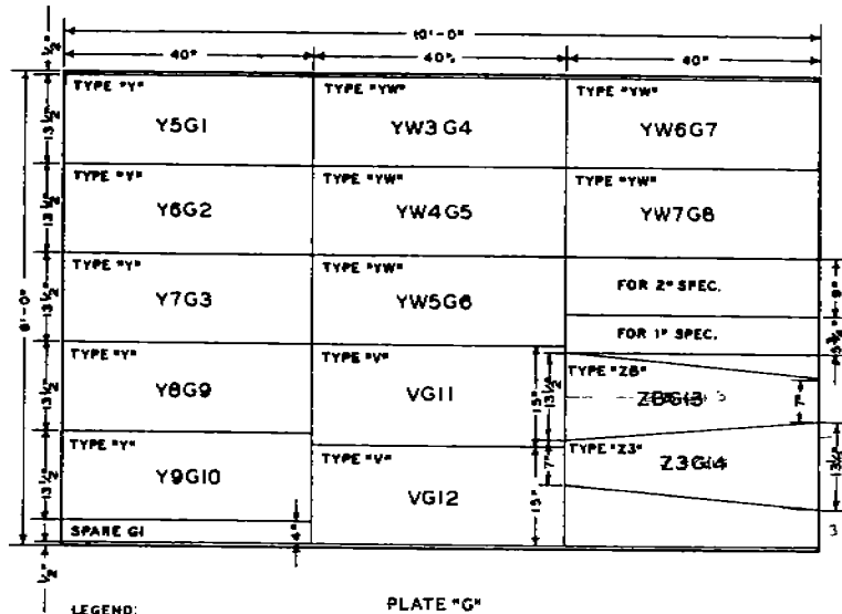
FIG. 9 3/4" DN PLATE LAYOUT CODE C.G.
